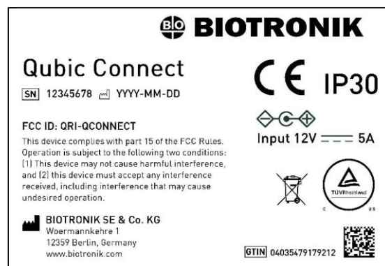
Figure 3: Qubic Connect type label
