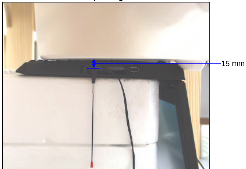
EUT Set-up configuration 1
