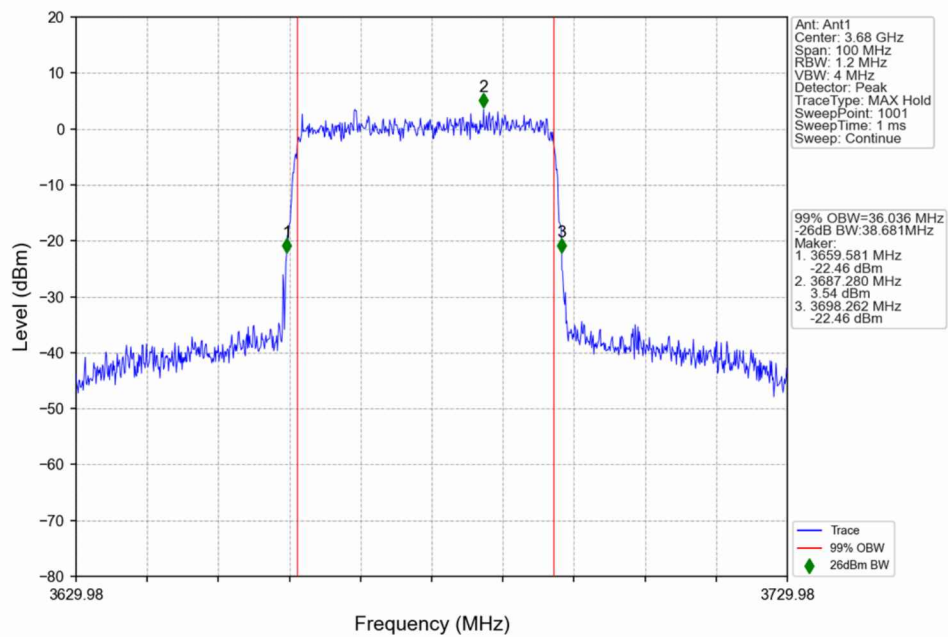
n48_30kHz_SISO_NTNV_40MHz_DFT-s-OFDM_16_QAM_3679.98MHz_Outer_Full
