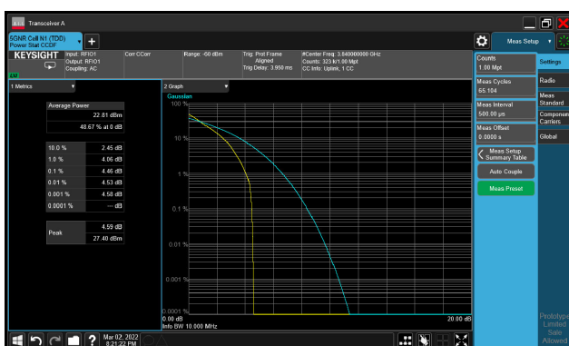
5G NR n77_CH656000_10M_1RB_QPSK_Ratio
