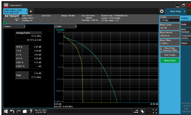
5G NR n77_CH647000_10M_1RB_16-QAM_Ratio
