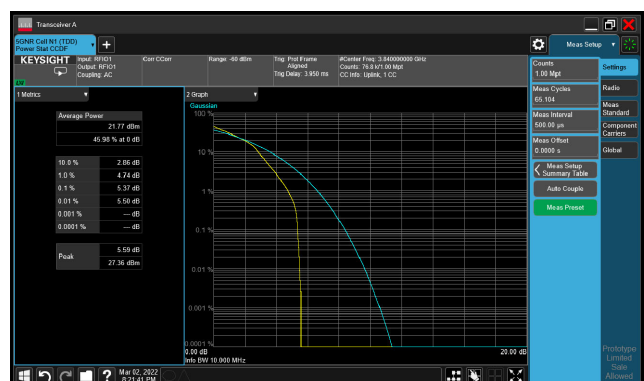
5G NR n77_CH656000_10M_1RB_16-QAM_Ratio
