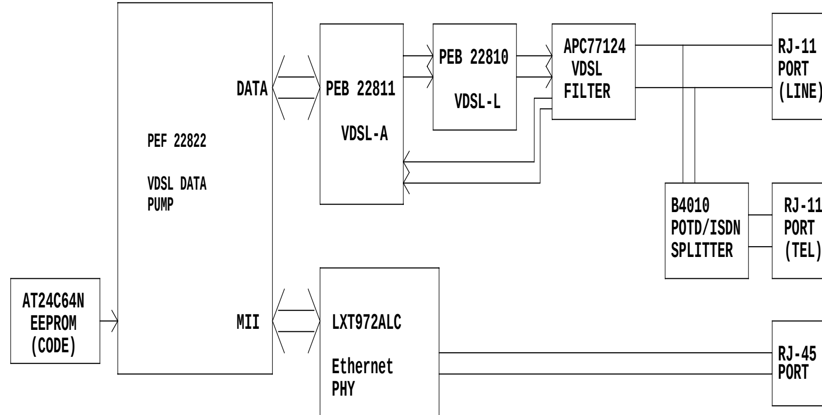
1. Block Diagram
