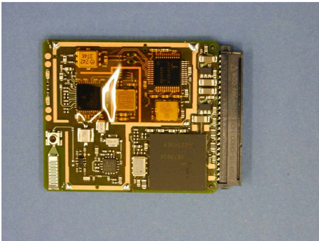
Module-Bottom without RF Shield
