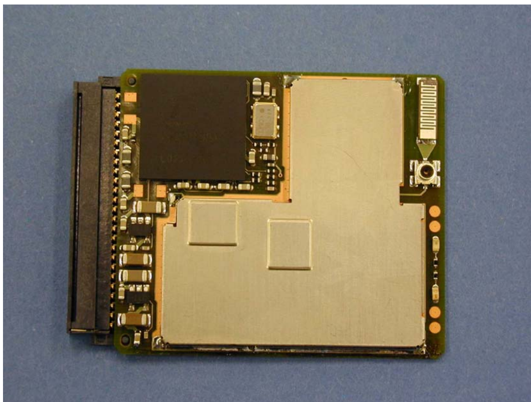
Module-Bottom with RF Shield
