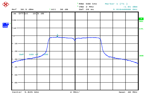
a_5825MHz_Chain 0 -1.91dBm/MHz
