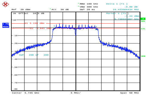
n20_5745MHz_Chain 0 16.434MHz
