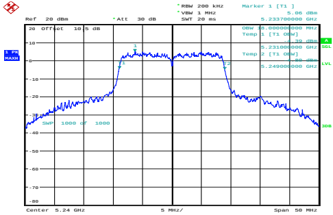
n20_5240MHz_Chain 0 18MHz
