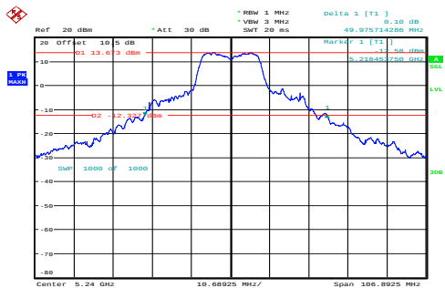
a_5240MHz_Chain 0 49.976MHz
