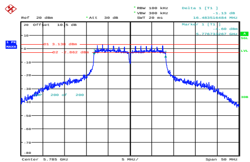
a_5785MHz_Chain 0 16.484MHz
