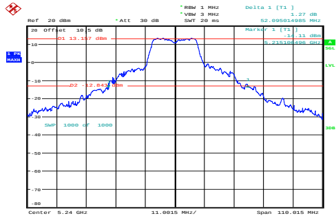
n20_5240MHz_Chain 0 52.095MHz
