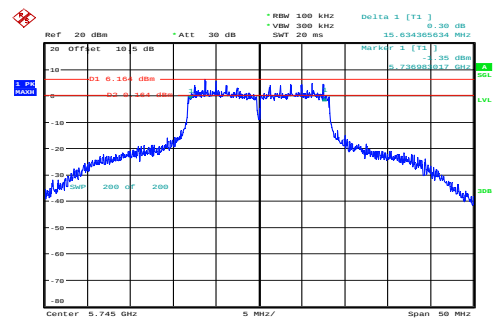
a_5745MHz_Chain 0 15.634MHz
