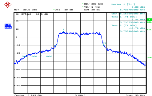
a_5745MHz_Chain 0 18.150MHz
