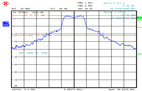
a_5200MHz_Chain 0 44.754MHz
