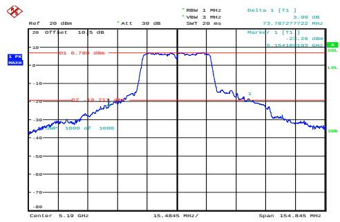
n40_5190MHz_Chain 0 73.787MHz
