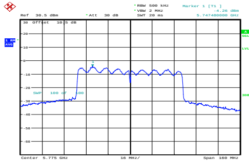
ac80_5775MHz_Chain 0 -4.26dBm/MHz
