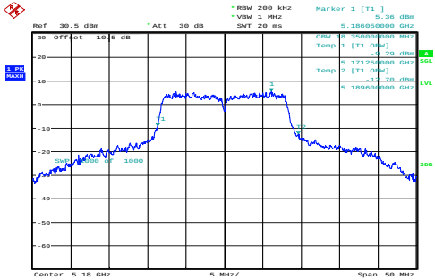
a_5180MHz_Chain 0 18.350MHz
