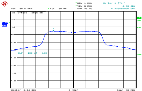
n20_5240MHz_Chain 0 4.33dBm/MHz
