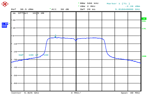
n20_5825MHz_Chain 0 -2.28dBm/MHz
