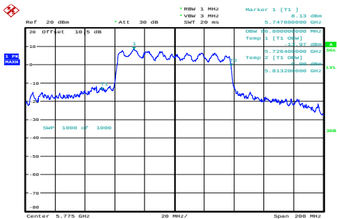
ac80_5775MHz_Chain 0 86.800MHz
