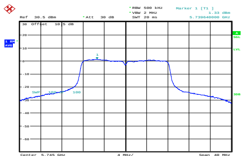
a_5745MHz_Chain 0 1.33dBm/MHz
