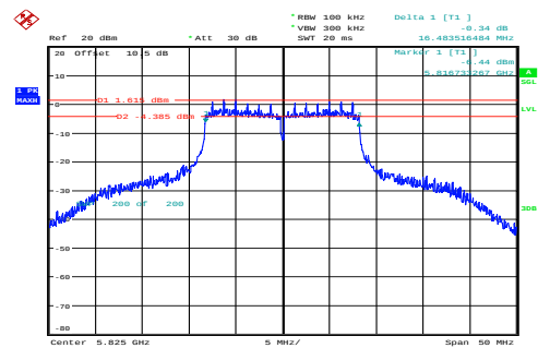
a_5825MHz_Chain 0 16.484MHz
