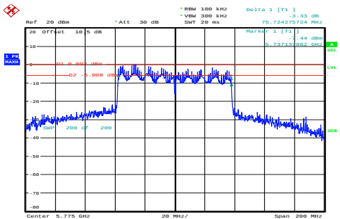
ac80_5775MHz_Chain 0 75.724MHz
