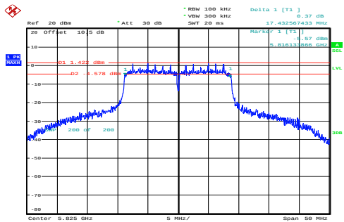
n20_5825MHz_Chain 0 17.433MHz
