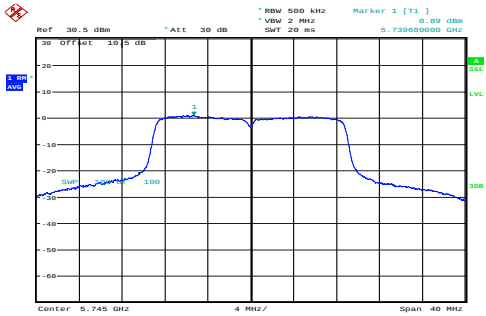
n20_5745MHz_Chain 0 0.89dBm/MHz
