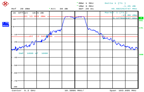
n20_5200MHz_Chain 0 46.602MHz
