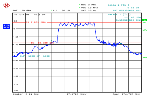
ac80_5210MHz_Chain 0 147.654MHz
