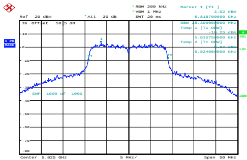
n20_5825MHz_Chain 0 18.300MHz
