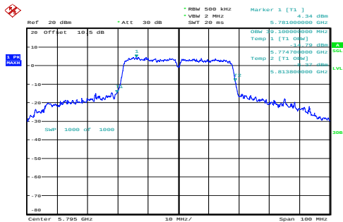
n40_5795MHz_Chain 0 39.100MHz
