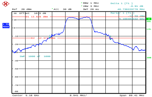
a_5180MHz_Chain 0 40.730MHz
