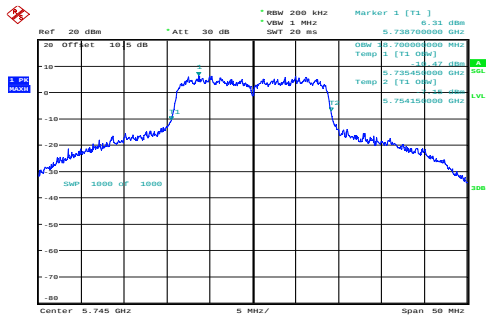
n20_5745MHz_Chain 0 18.700MHz
