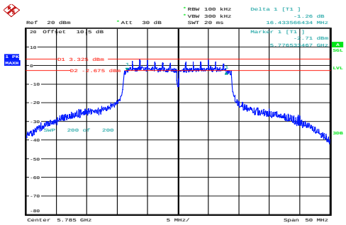
n20_5785MHz_Chain 0 16.434MHz
