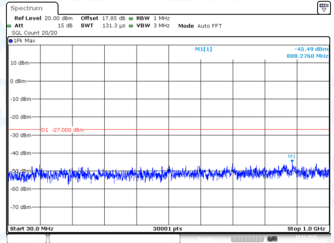
11N20-CDD-Ant2-5825-30~1000-PASS
