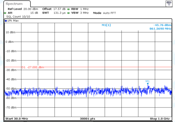
11N20-CDD-Ant2-5240-30~1000-PASS
