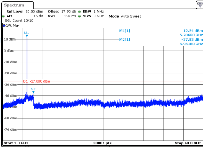
11N40-CDD-Ant1-5710-1000~40000-PASS
