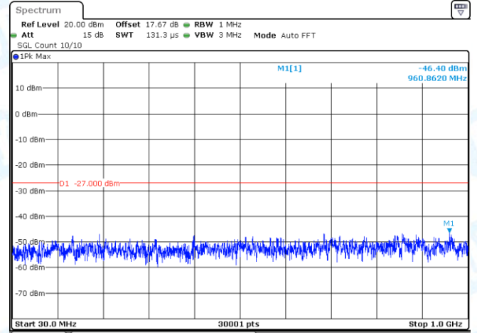
11N40-CDD-Ant2-5550-30~1000-PASS
