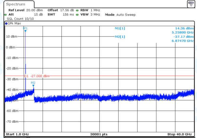
11N20-CDD-Ant2-5260-1000~40000-PASS
