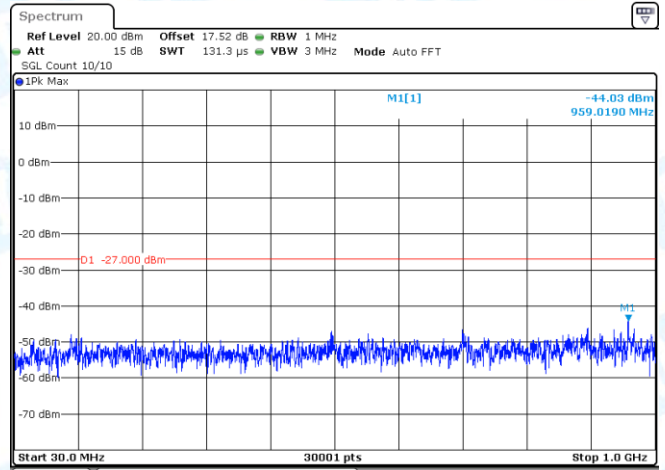
11N20-CDD-Ant2-5320-30~1000-PASS
