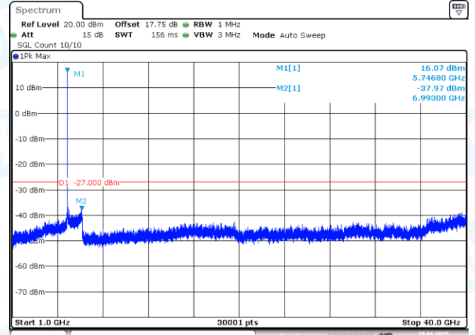
11N20-CDD-Ant2-5745-1000~40000-PASS
