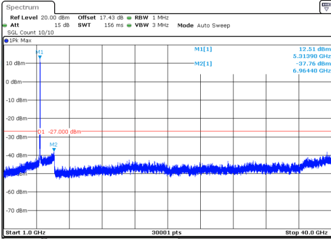
11N40-CDD-Ant1-5310-1000~40000-PASS
