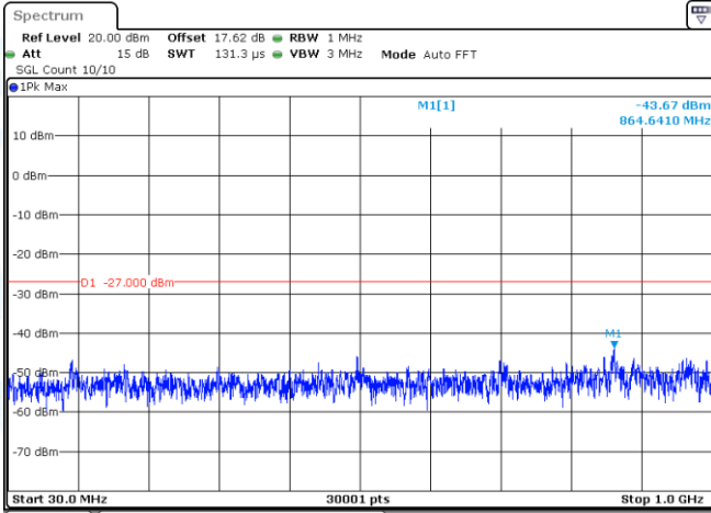
11N40-CDD-Ant1-5550-30~1000-PASS
