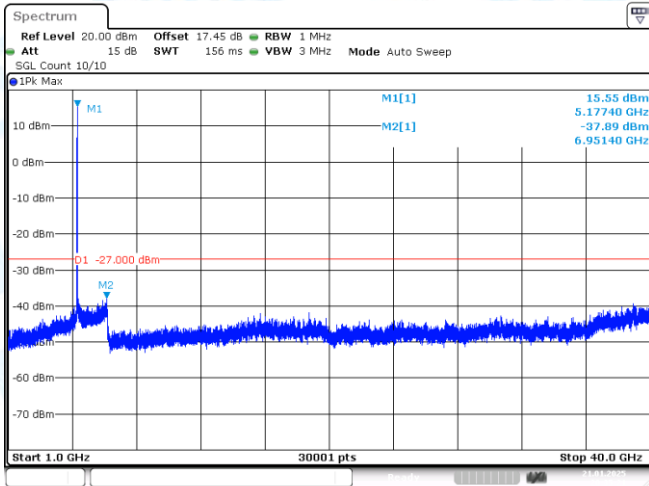
11N20-CDD-Ant1-5180-1000~40000-PASS
