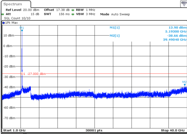
11N40-CDD-Ant1-5190-1000~40000-PASS
