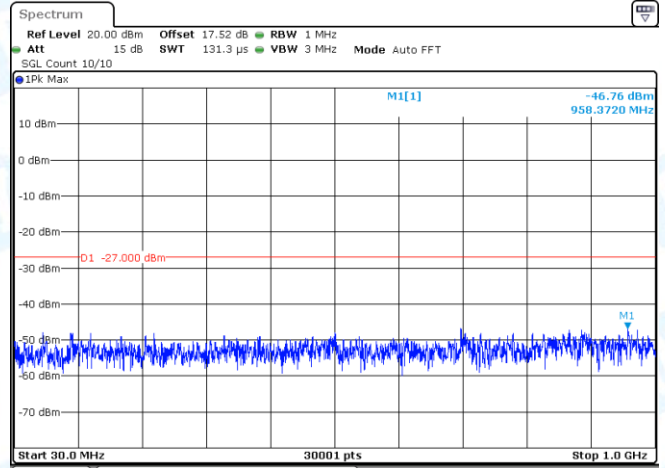
11N40-CDD-Ant2-5270-30~1000-PASS
