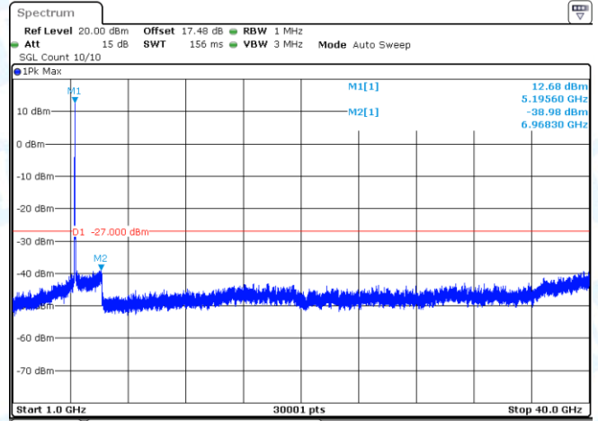
11N40-CDD-Ant2-5190-1000~40000-PASS
