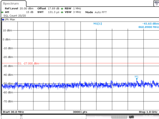
11N40-CDD-Ant1-5795-30~1000-PASS
