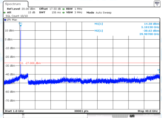
11N20-CDD-Ant2-5180-1000~40000-PASS
