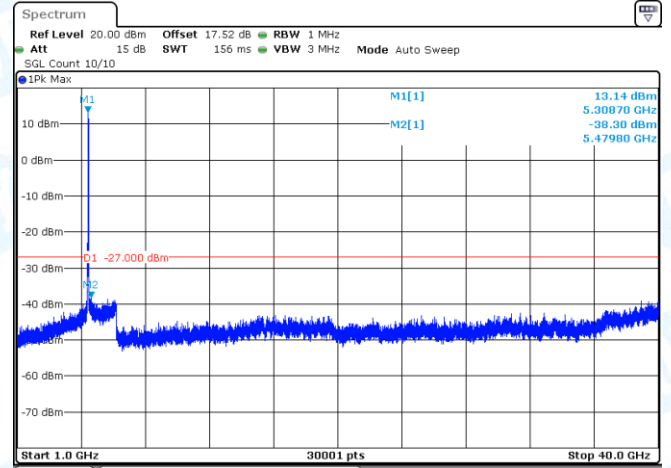
11N40-CDD-Ant2-5310-1000~40000-PASS
