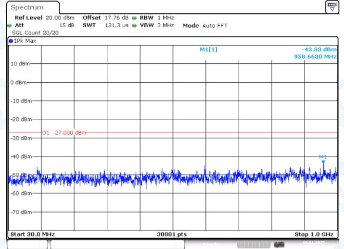
11N40-CDD-Ant2-5795-30~1000-PASS
