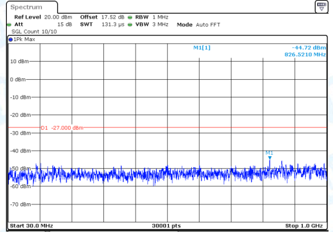
11A-CDD-Ant2-5320-30~1000-PASS
