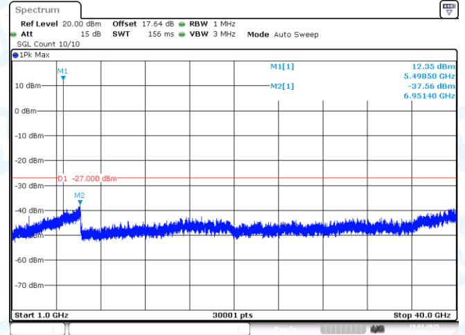
11N20-CDD-Ant2-5500-1000~40000-PASS
