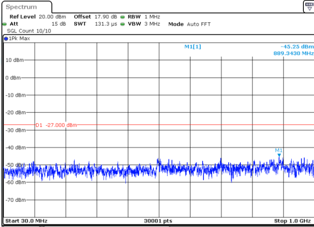
11A-CDD-Ant1-5720-30~1000-PASS
