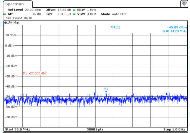
11A-CDD-Ant2-5720-30~1000-PASS
