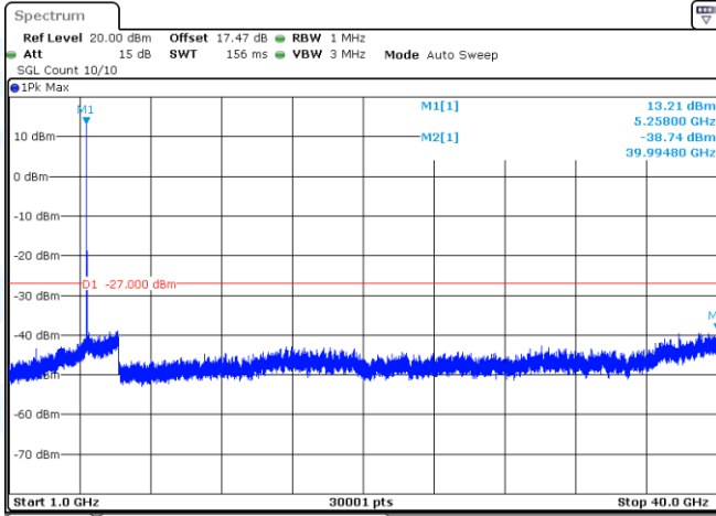
11N20-CDD-Ant1-5260-1000~40000-PASS
