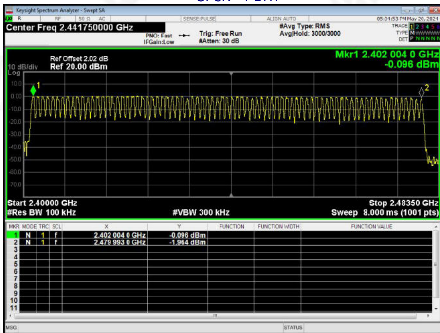
GFSK - 1-DH1
