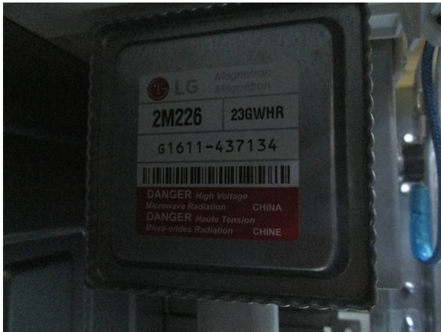
EUT – Magnetron Label View
