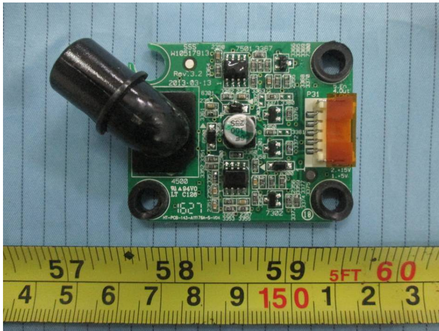
EUT – Main Board 3 Front View
