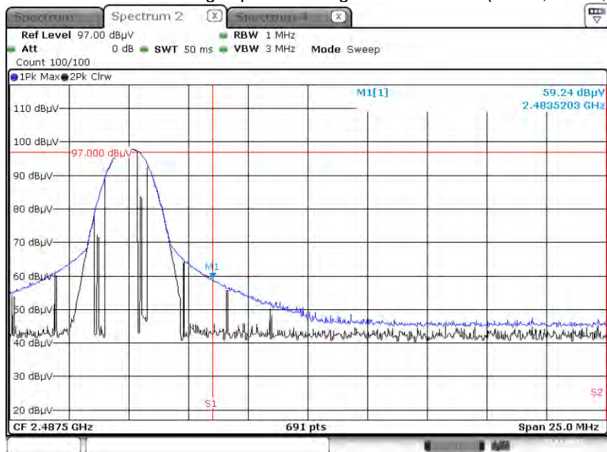
Radiated Restricted Band Edges plot – Average & Peak Result (GFSK, Ch.78, Z-V)
