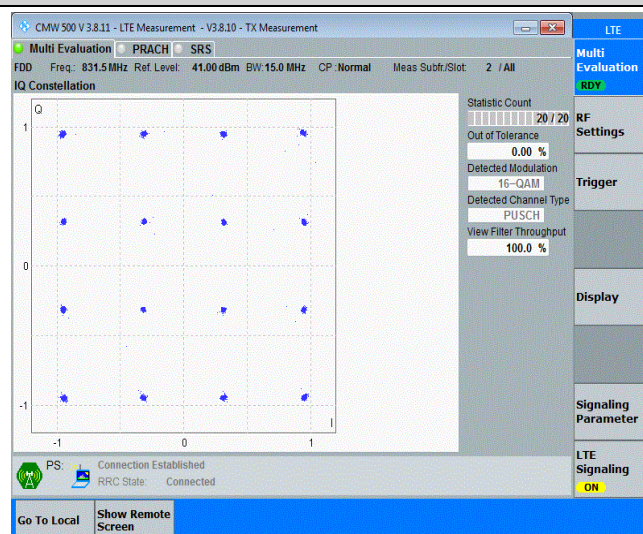
Band26-15MHz-16QAM-26915-75RB#0
