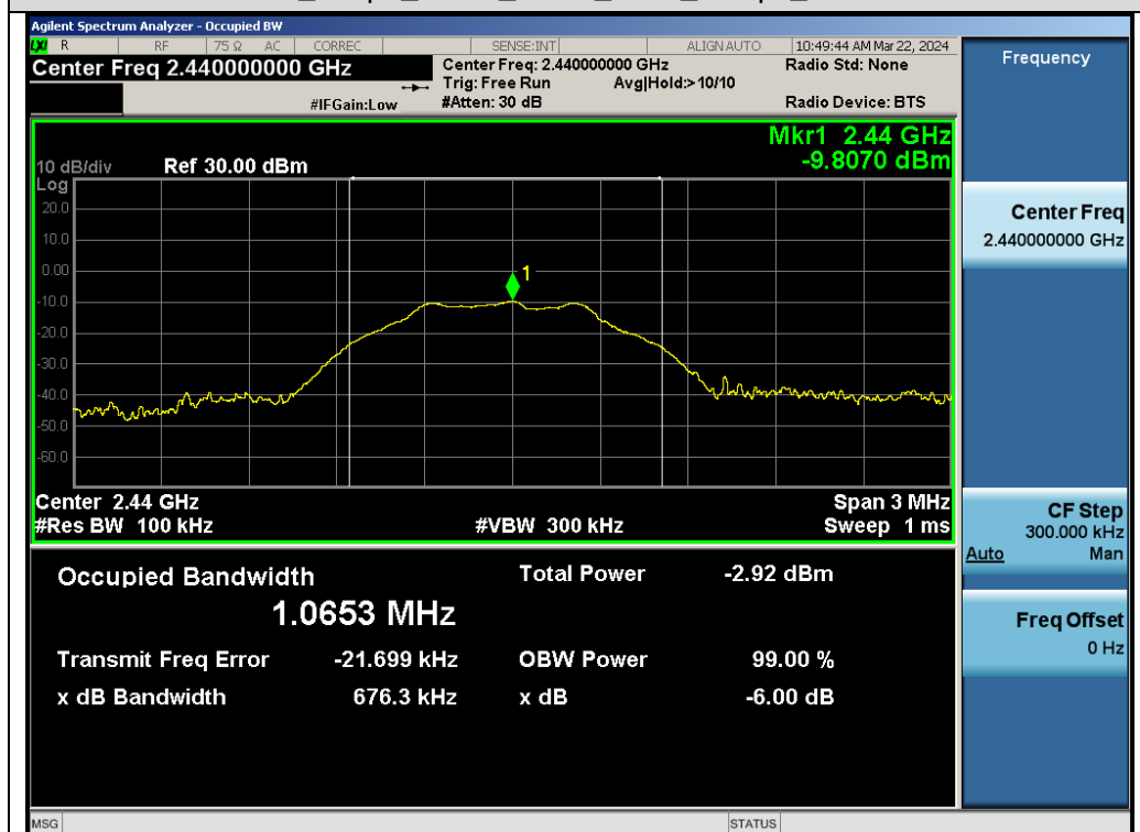
Test_Graph_LE1M_ANT1_2440_1Mbps_DTBSW
