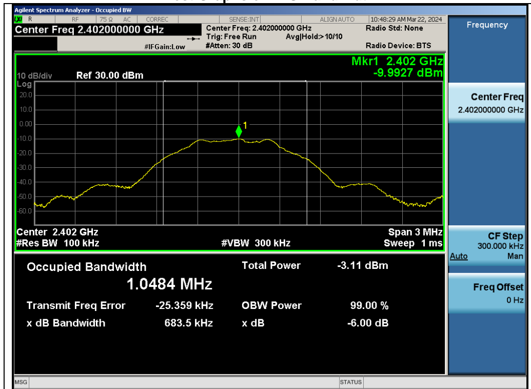
Test_Graph_LE1M_ANT1_2402_1Mbps_DTBSW
