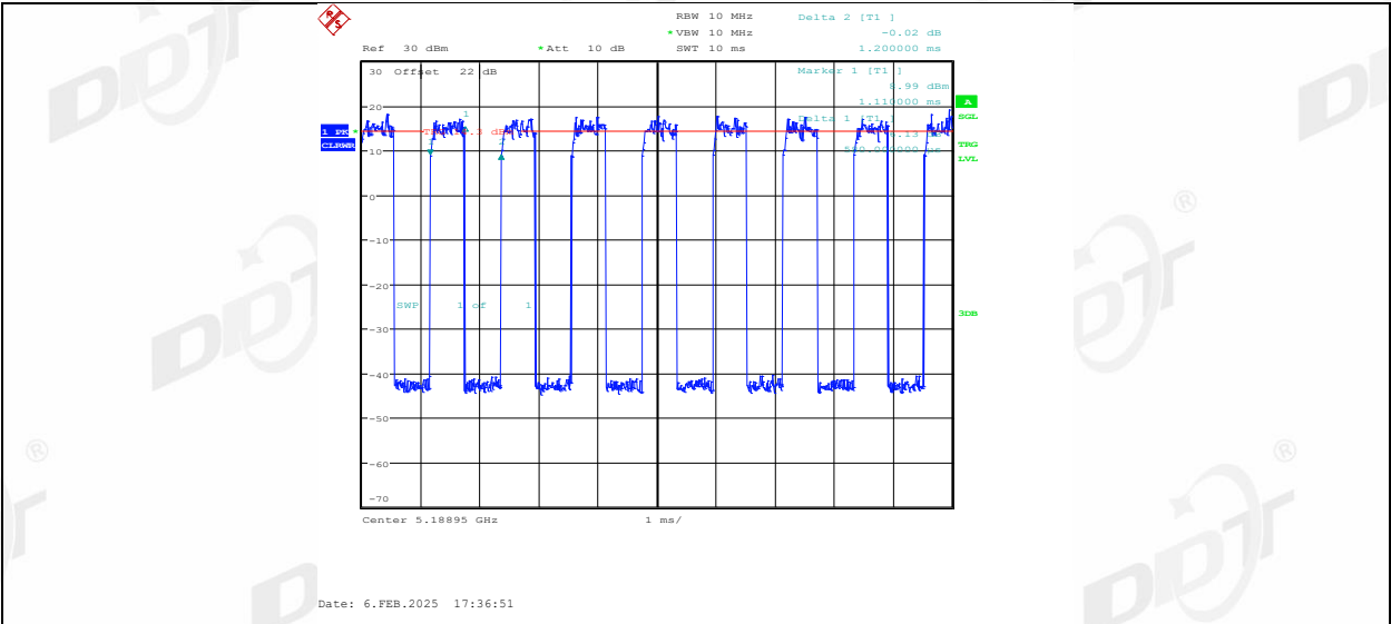
11AX20MIMO Ant2 5180 52Tone RU37
