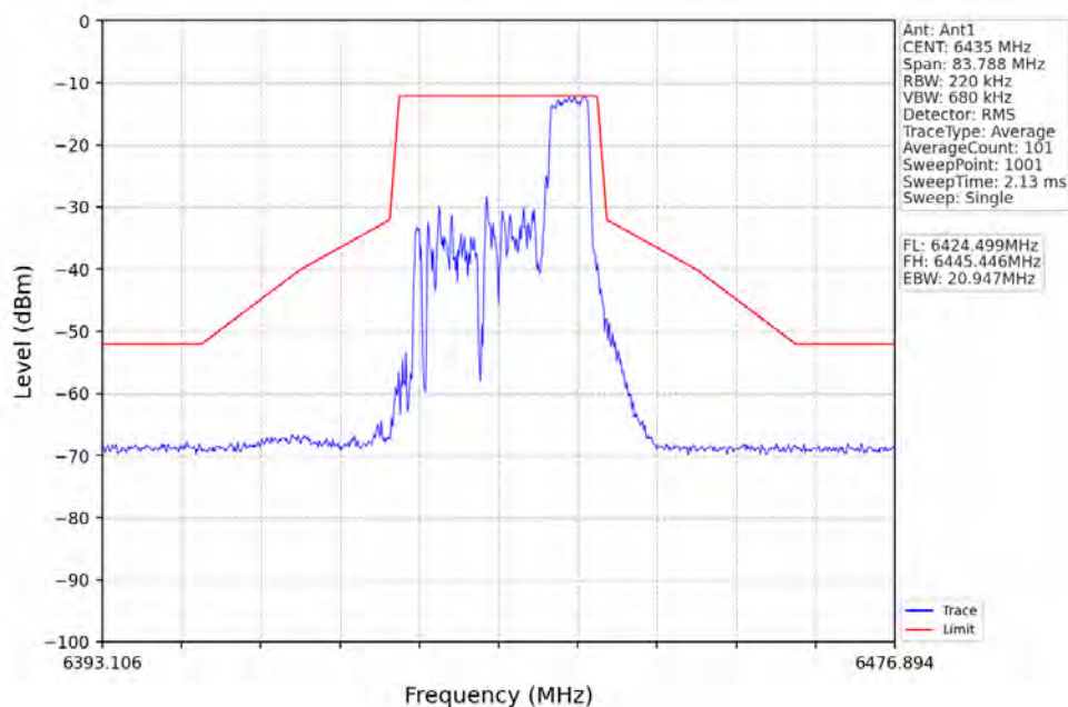
802.11ax(HEW20)_LCH_6435MHz_RU52_Right_Ant1_NTNV
