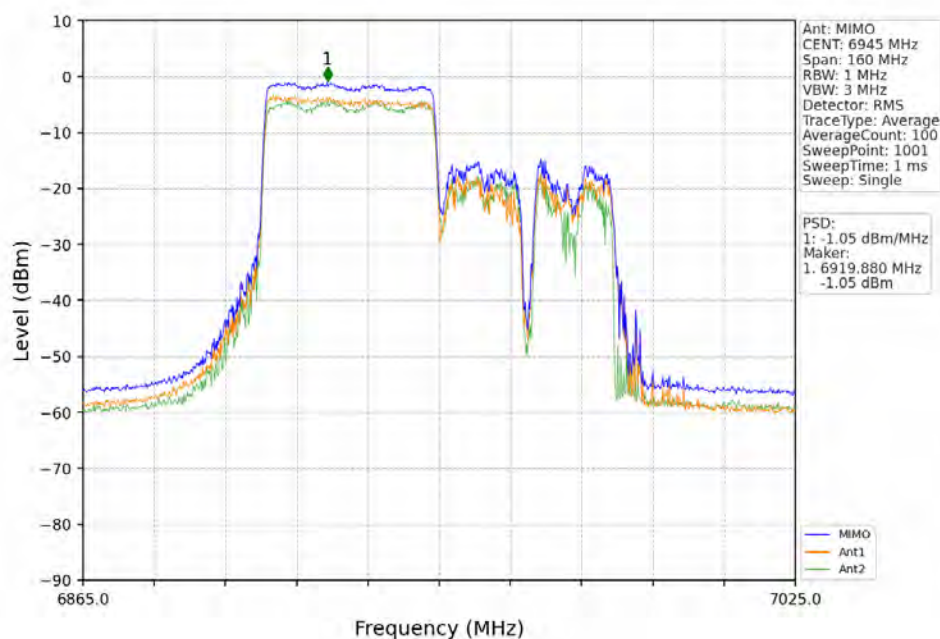
802.11ax(HEW80)_LCH_6945MHz_RU484_Right_MIMO_NTNV
