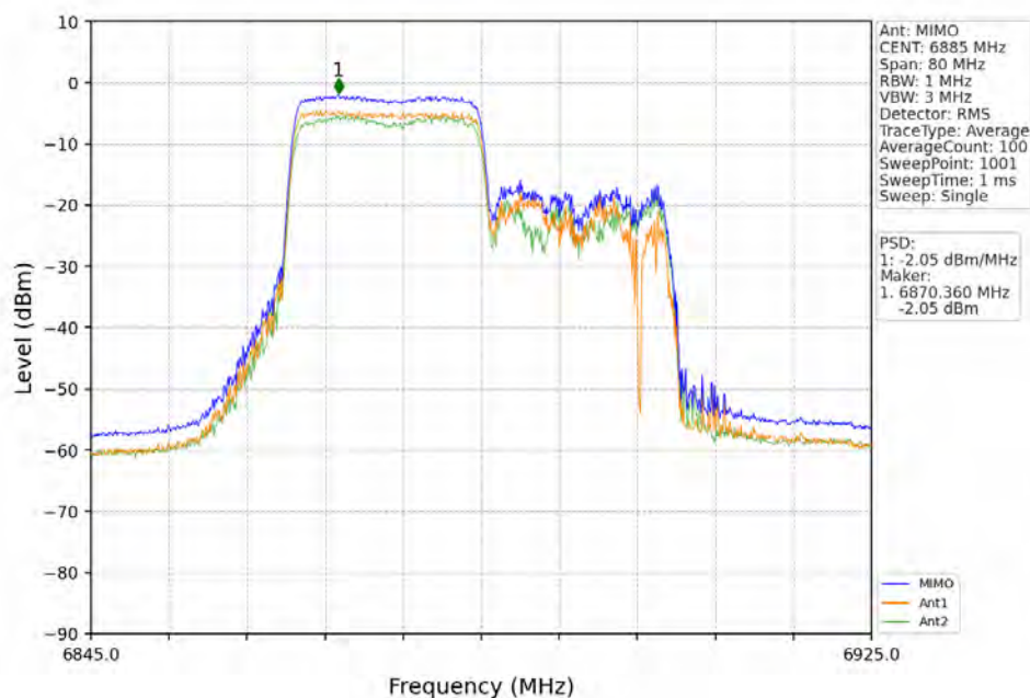
802.11ax(HEW40)_HCH_6885MHz_RU242_Left_MIMO_NTNV
