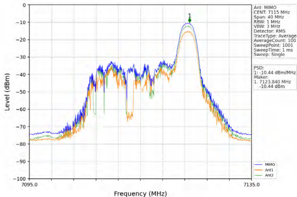
802.11ax(HEW20)_HCH_7115MHz_RU26_Right_MIMO_NTNV
