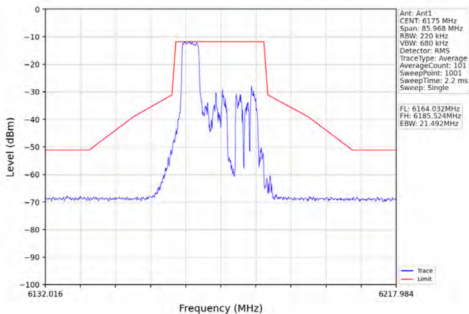
802.11ax(HEW20)_MCH_6175MHz_RU52_Left_Ant1_NTNV
