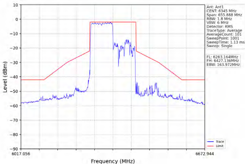
802.11ax(HEW160)_HCH_6345MHz_RU996_Left_Ant1_NTNV
