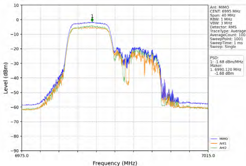
802.11ax(HEW20)_MCH_6995MHz_RU106_Left_MIMO_NTNV
