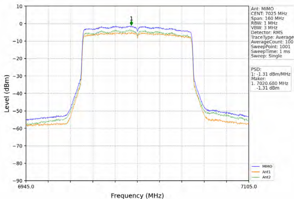
802.11ax(HEW80)_HCH_7025MHz_RU996_Left_MIMO_NTNV
