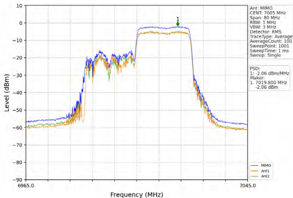
802.11ax(HEW40)_MCH_7005MHz_RU242_Right_MIMO_NTNV
