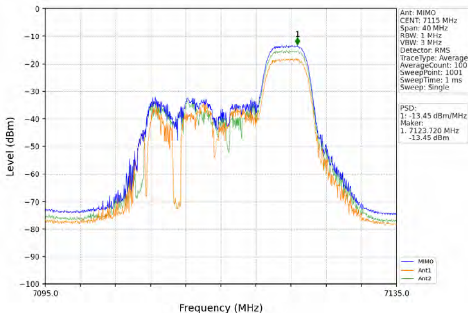
802.11ax(HEW20)_HCH_7115MHz_RU52_Right_MIMO_NTNV
