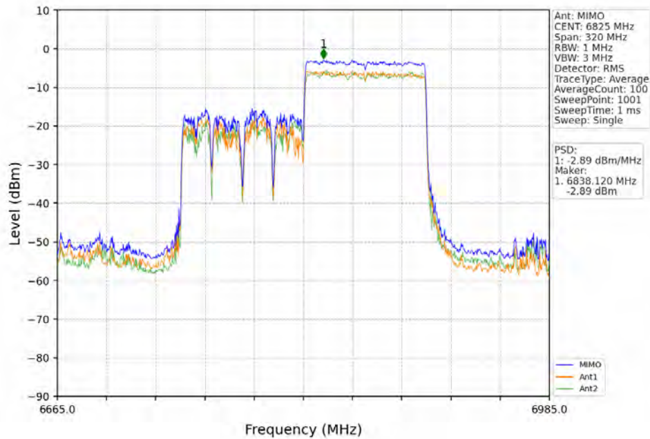
802.11ax(HEW160)_HCH_6825MHz_2xRU996_Left_MIMO_NTNV
