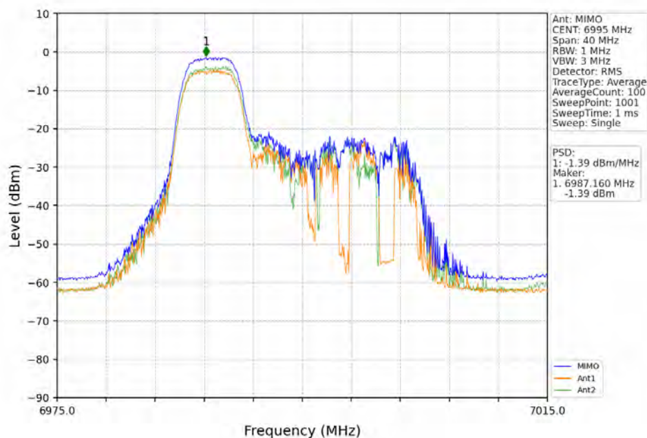
802.11ax(HEW20)_MCH_6995MHz_RU52_Left_MIMO_NTNV
