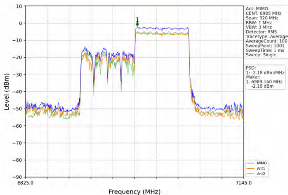
802.11ax(HEW160)_MCH_6985MHz_RU996_Right_MIMO_NTNV
