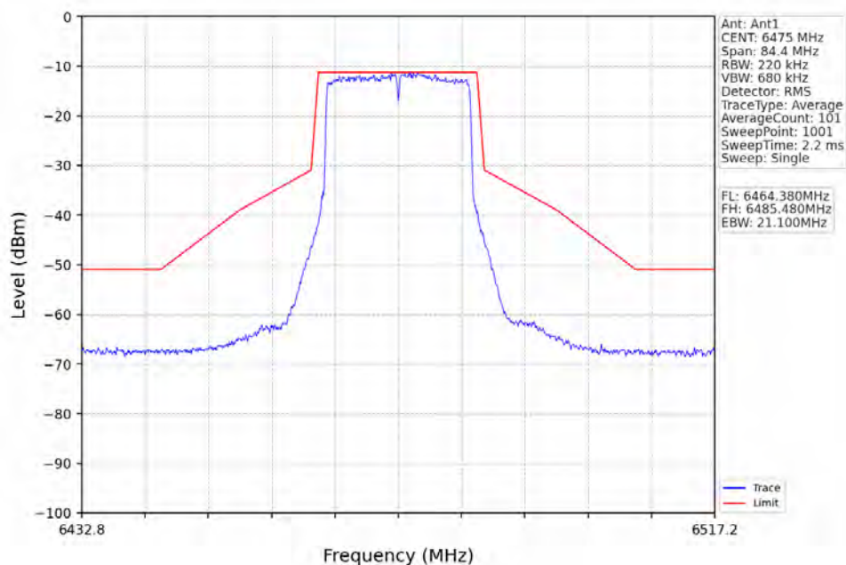
802.11ax(HEW20)_MCH_6475MHz_RU242_Left_Ant1_NTNV
