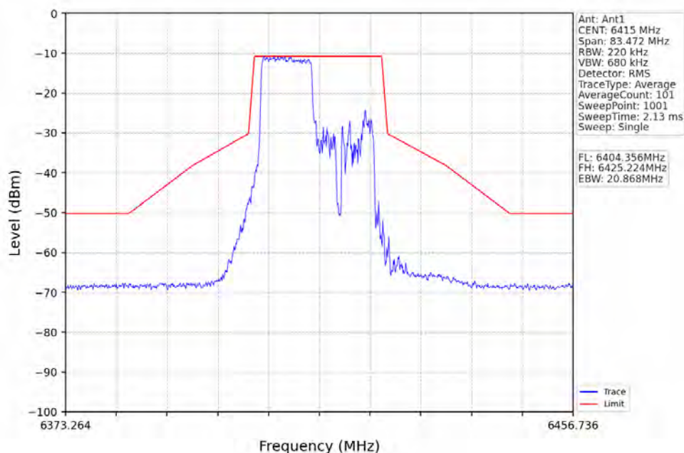
802.11ax(HEW20)_HCH_6415MHz_RU106_Right_Ant1_NTNV
