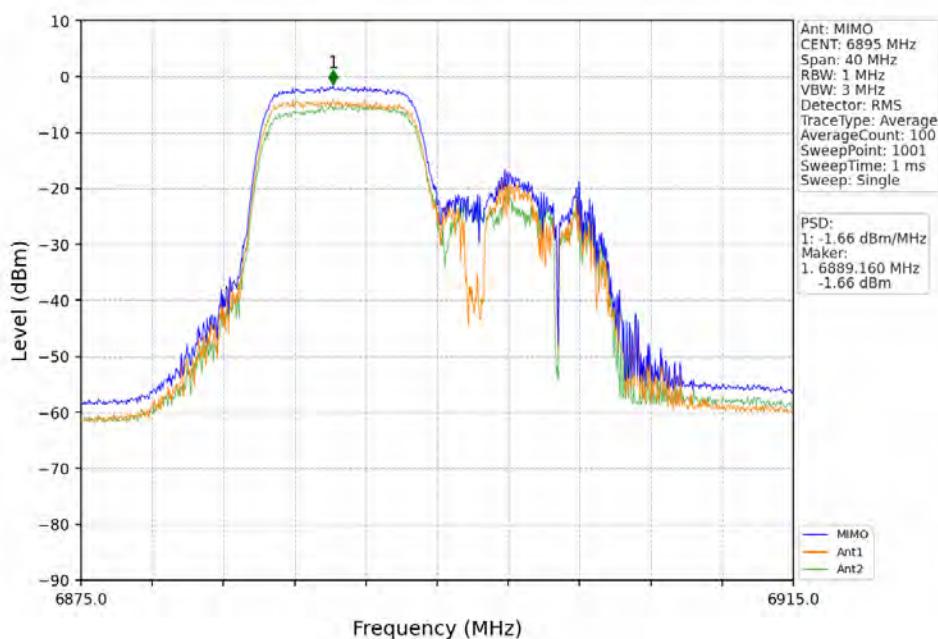
802.11ax(HEW20)_LCH_6895MHz_RU106_Right_MIMO_NTNV
