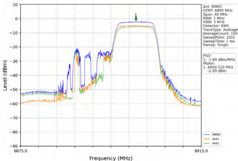
802.11ax(HEW20)_LCH_6895MHz_RU106_Right_MIMO_NTNV
