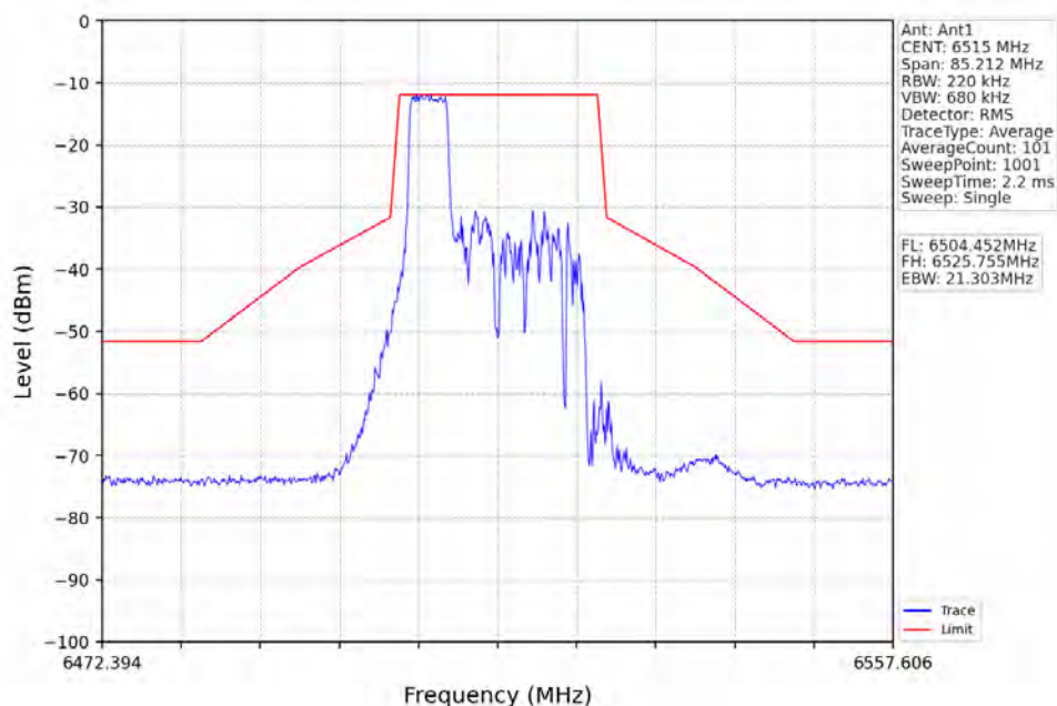
802.11ax(HEW20)_HCH_6515MHz_RU52_Right_Ant1_NTNV
