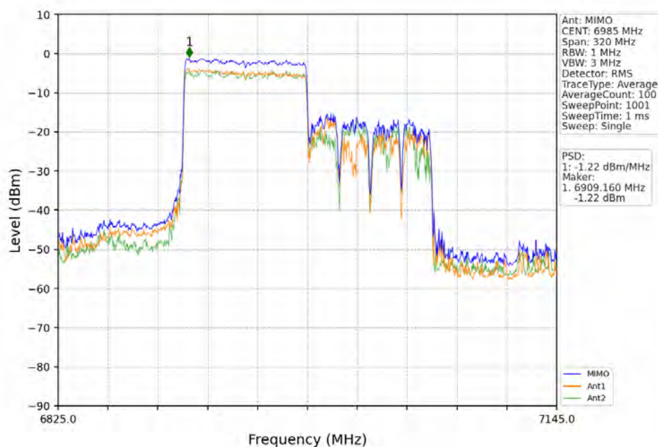
802.11ax(HEW160)_MCH_6985MHz_RU996_Right_MIMO_NTNV
