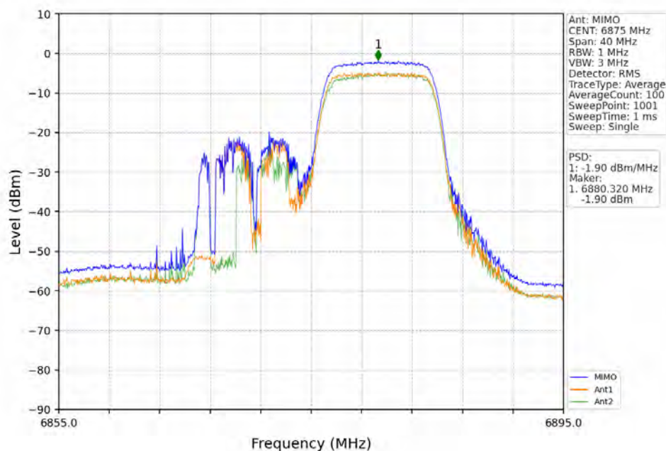
802.11ax(HEW20)_HCH_6875MHz_RU106_Right_MIMO_NTNV
