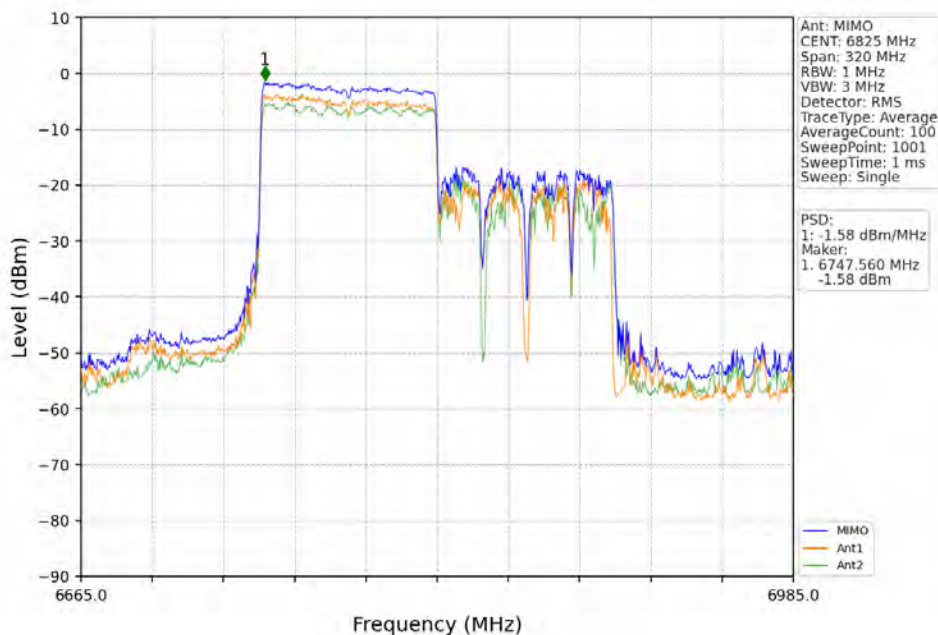
802.11ax(HEW160)_HCH_6825MHz_RU996_Left_MIMO_NTNV
