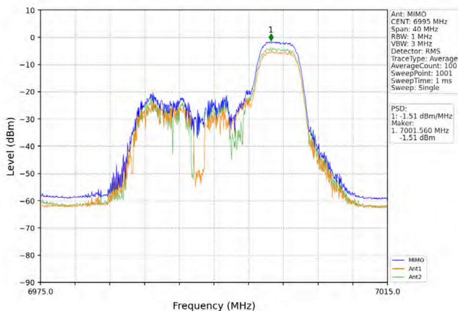
802.11ax(HEW20)_MCH_6995MHz_RU106_Left_MIMO_NTNV
