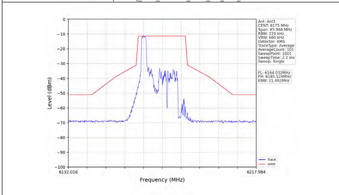
802.11ax(HEW20)_MCH_6175MHz_RU26_Left_Ant1_NTNV
