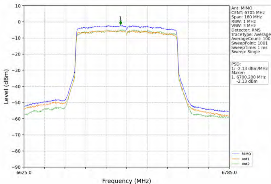
802.11ax(HEW80)_MCH_6705MHz_RU996_Left_MIMO_NTNV
