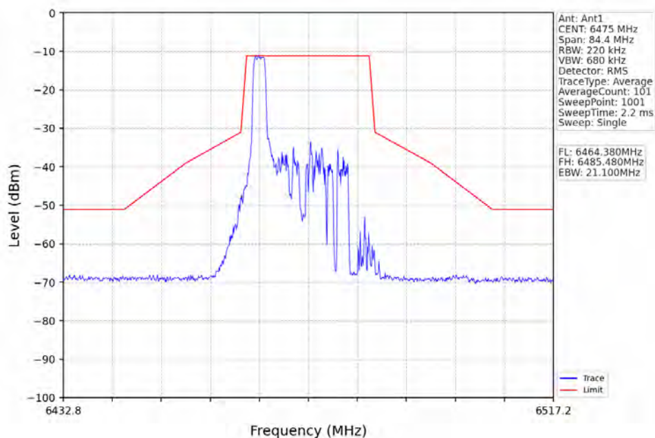
802.11ax(HEW20)_MCH_6475MHz_RU26_Left_Ant1_NTNV
