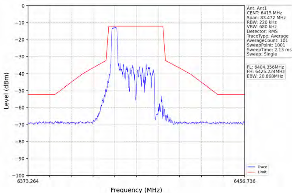
802.11ax(HEW20)_HCH_6415MHz_RU26_Right_Ant1_NTNV
