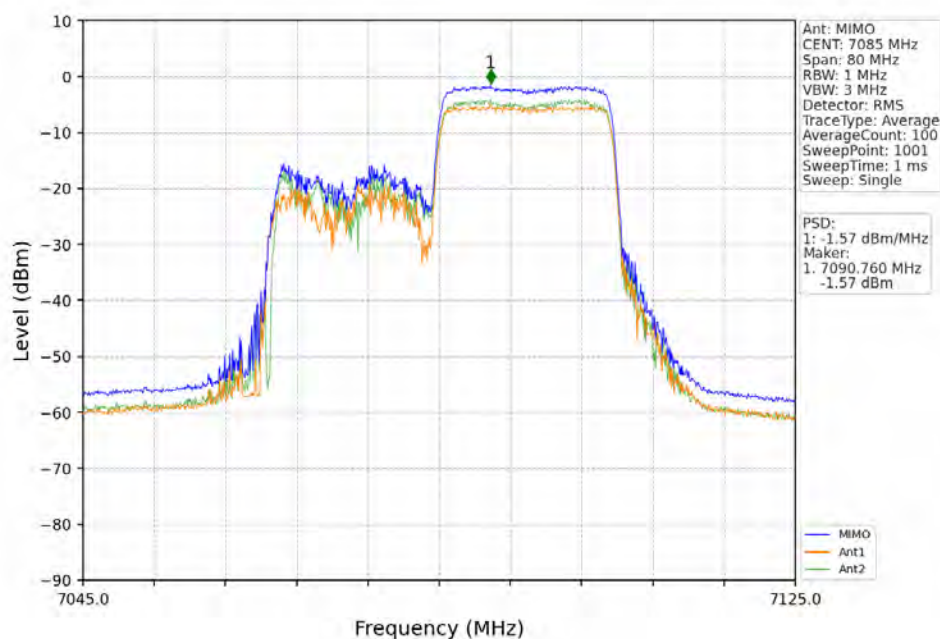
802.11ax(HEW40)_HCH_7085MHz_RU484_Left_MIMO_NTNV
