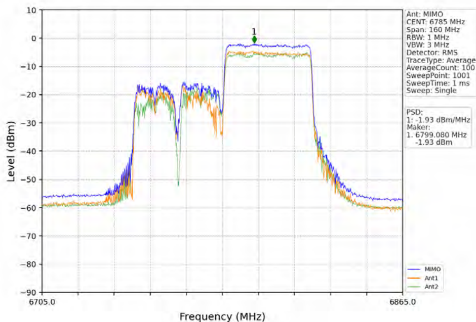
802.11ax(HEW80)_HCH_6785MHz_RU484_Right_MIMO_NTNV
