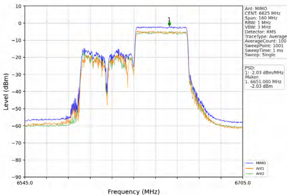
802.11ax(HEW80)_LCH_6625MHz_RU484_Right_MIMO_NTNV
