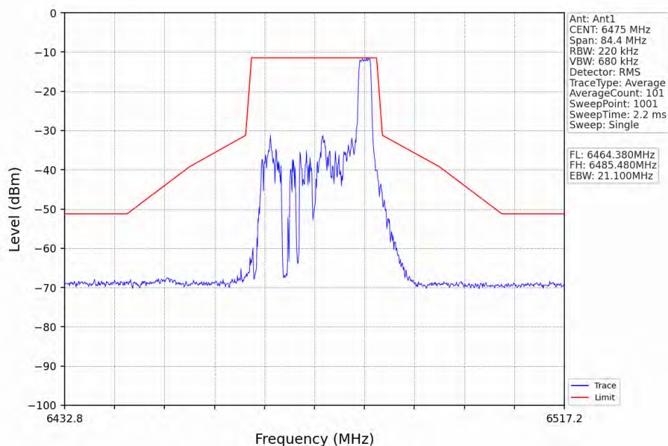
802.11ax(HEW20)_MCH_6475MHz_RU52_Left_Ant1_NTNV
