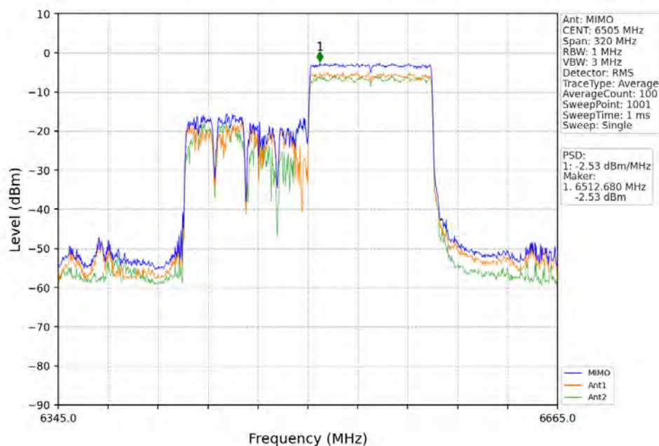
802.11ax(HEW160)_HCH_6505MHz_RU996_Right_MIMO_NTNV
