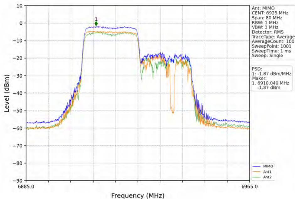
802.11ax(HEW40)_LCH_6925MHz_RU242_Left_MIMO_NTNV
