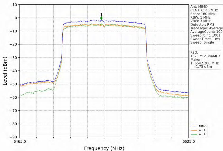
802.11ax(HEW80)_HCH_6545MHz_RU996_Left_MIMO_NTNV
