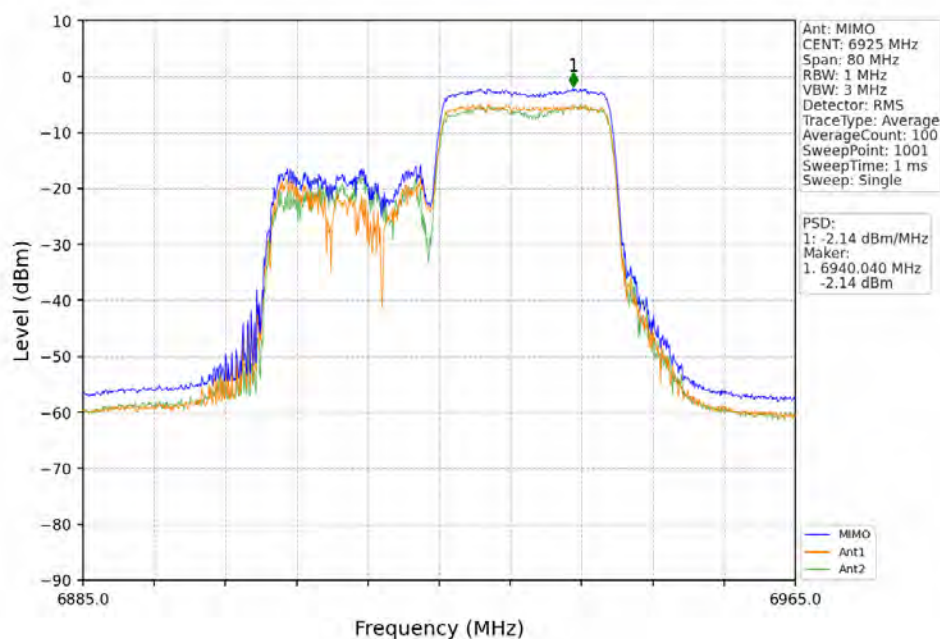
802.11ax(HEW40)_LCH_6925MHz_RU484_Left_MIMO_NTNV
