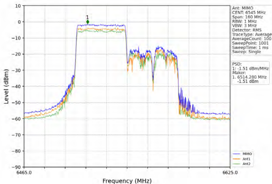
802.11ax(HEW80)_HCH_6545MHz_RU484_Left_MIMO_NTNV
