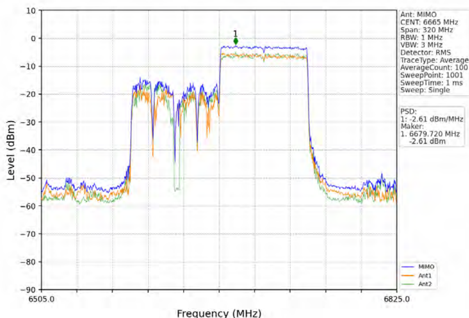
802.11ax(HEW160)_MCH_6665MHz_2xRU996_Left_MIMO_NTNV
