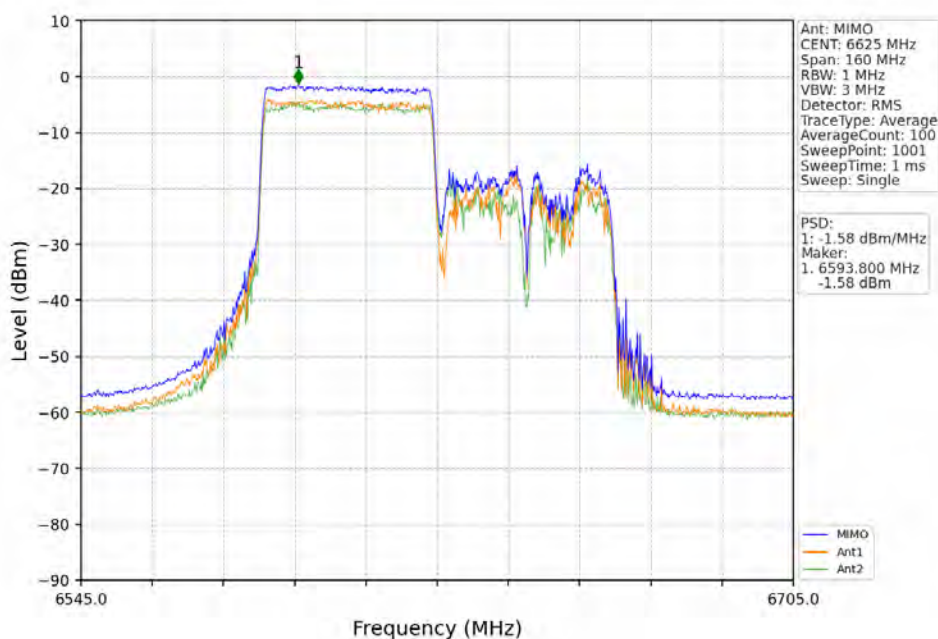
802.11ax(HEW80)_LCH_6625MHz_RU484_Right_MIMO_NTNV
