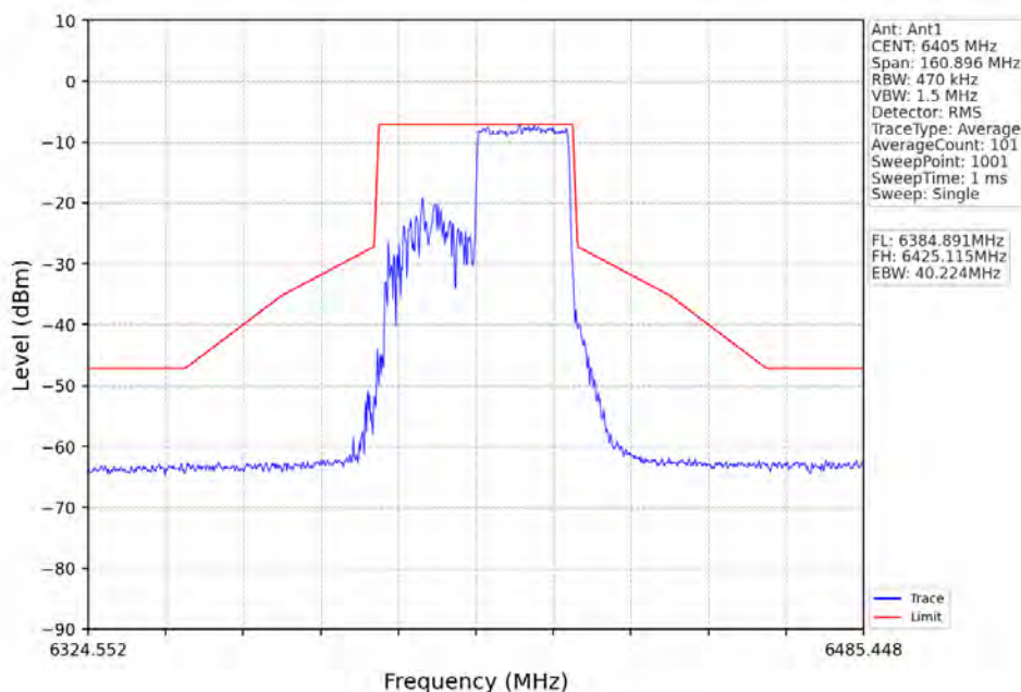
802.11ax(HEW40)_HCH_6405MHz_RU484_Left_Ant1_NTNV
