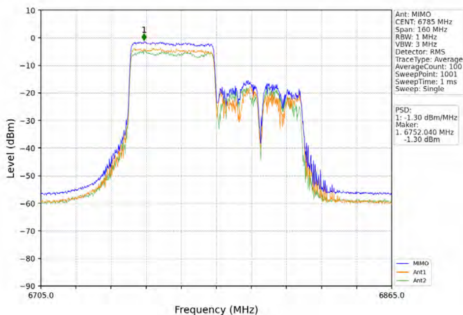
802.11ax(HEW80)_HCH_6785MHz_RU484_Right_MIMO_NTNV
