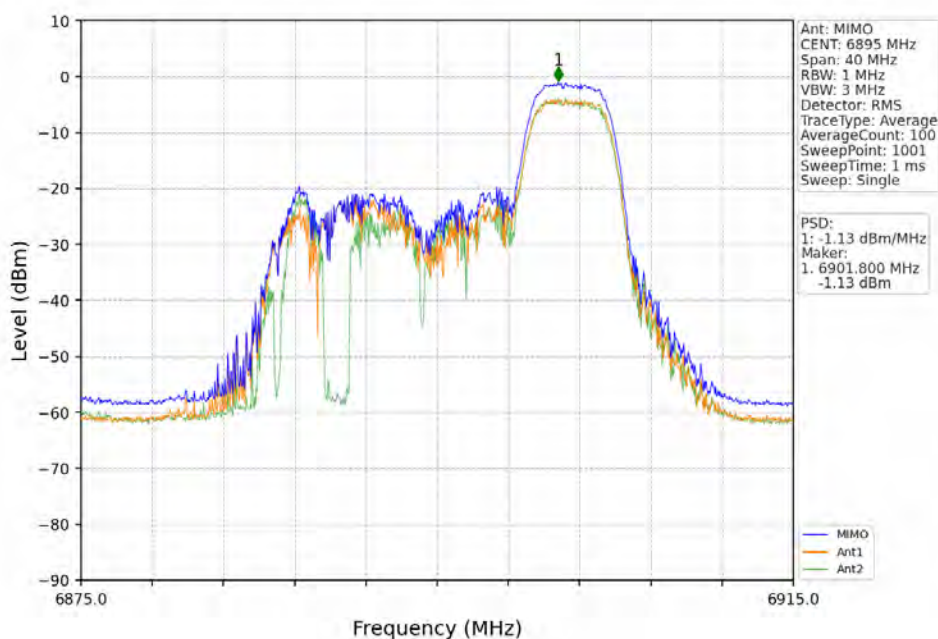
802.11ax(HEW20)_LCH_6895MHz_RU52_Right_MIMO_NTNV
