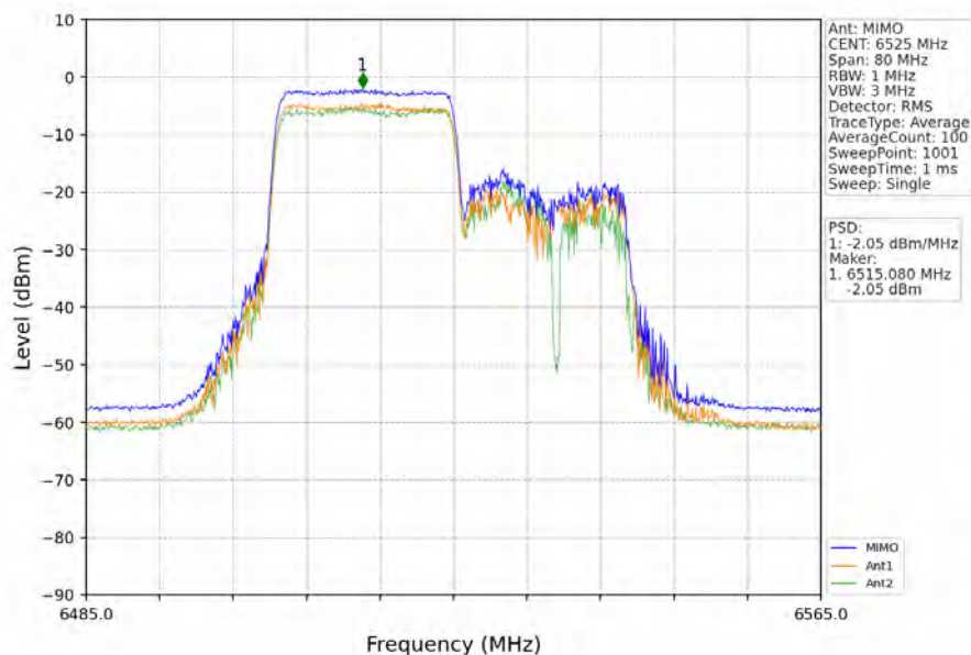
802.11ax(HEW40)_HCH_6525MHz_RU242_Right_MIMO_NTNV
