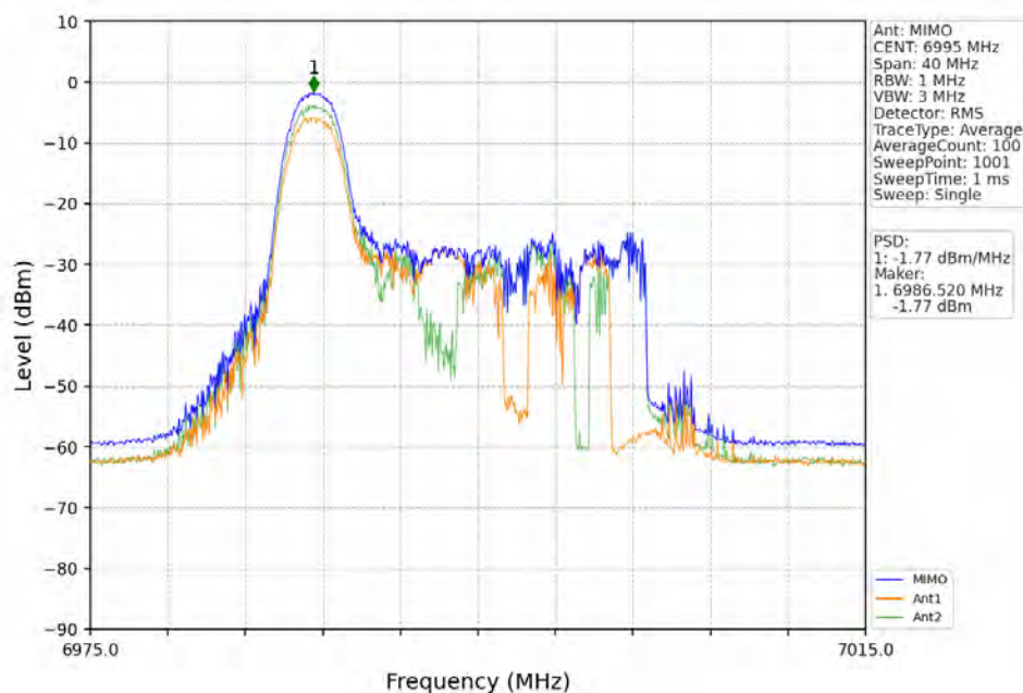
802.11ax(HEW20)_MCH_6995MHz_RU26_Left_MIMO_NTNV
