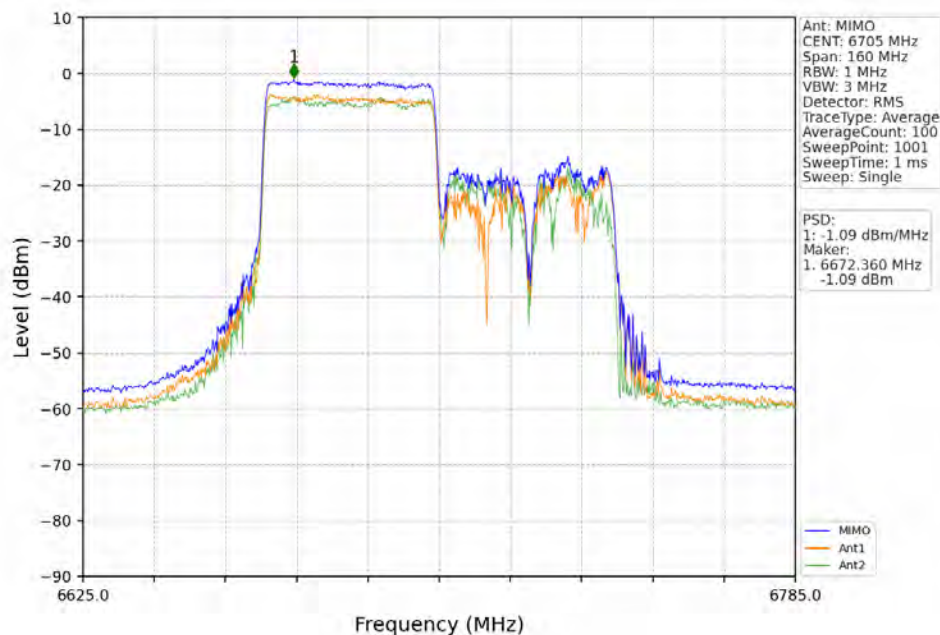
802.11ax(HEW80)_MCH_6705MHz_RU484_Left_MIMO_NTNV
