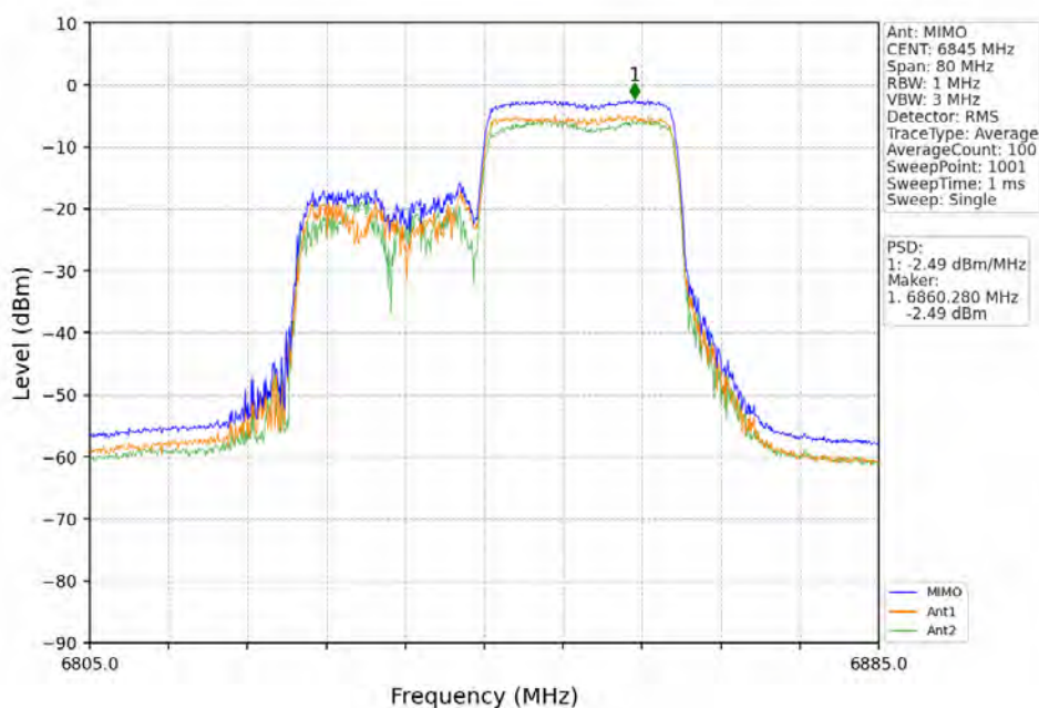
802.11ax(HEW40)_HCH_6845MHz_RU484_Left_MIMO_NTNV
