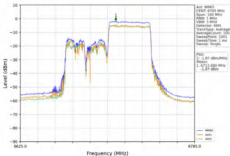
802.11ax(HEW80)_MCH_6705MHz_RU996_Left_MIMO_NTNV
