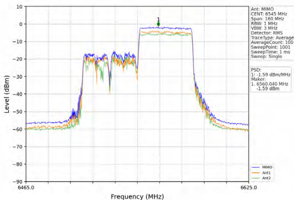
802.11ax(HEW80)_HCH_6545MHz_RU996_Left_MIMO_NTNV
