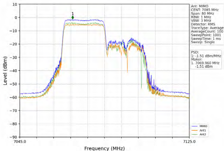
802.11ax(HEW40)_HCH_7085MHz_RU242_Left_MIMO_NTNV
