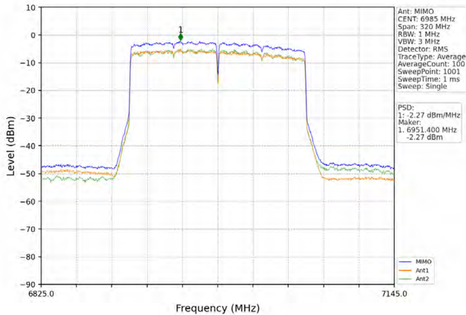
802.11ax(HEW160)_MCH_6985MHz_2xRU996_Left_MIMO_NTNV
