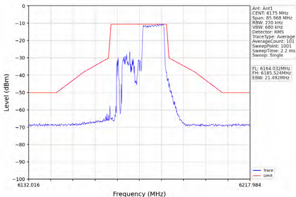
802.11ax(HEW20)_MCH_6175MHz_RU242_Left_Ant1_NTNV
