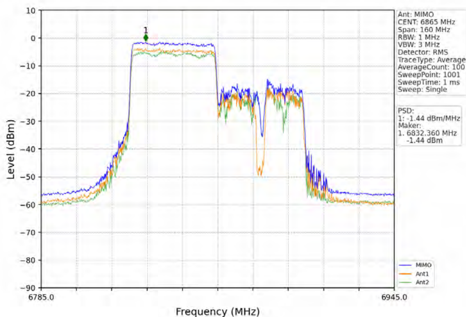
802.11ax(HEW80)_HCH_6865MHz_RU484_Right_MIMO_NTNV
