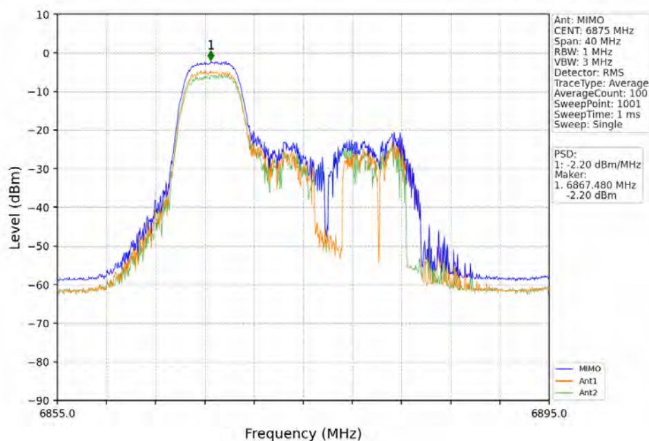
802.11ax(HEW20)_HCH_6875MHz_RU52_Right_MIMO_NTNV
