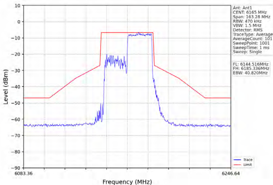
802.11ax(HEW40)_MCH_6165MHz_RU242_Right_Ant1_NTNV
