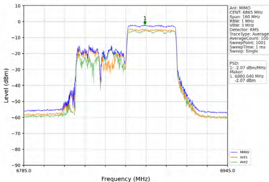
802.11ax(HEW80)_HCH_6865MHz_RU484_Right_MIMO_NTNV
