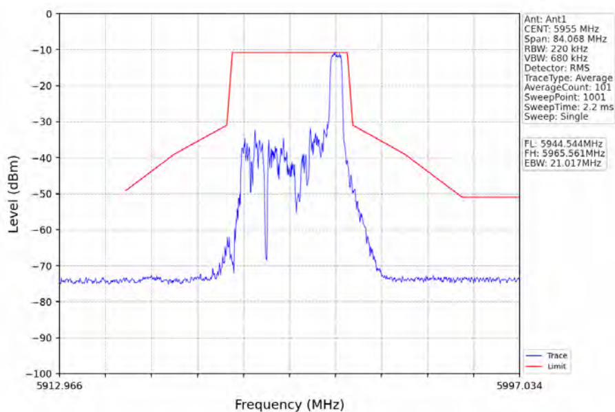
802.11ax(HEW20)_LCH_5955MHz_RU26_Right_Ant1_NTNV
