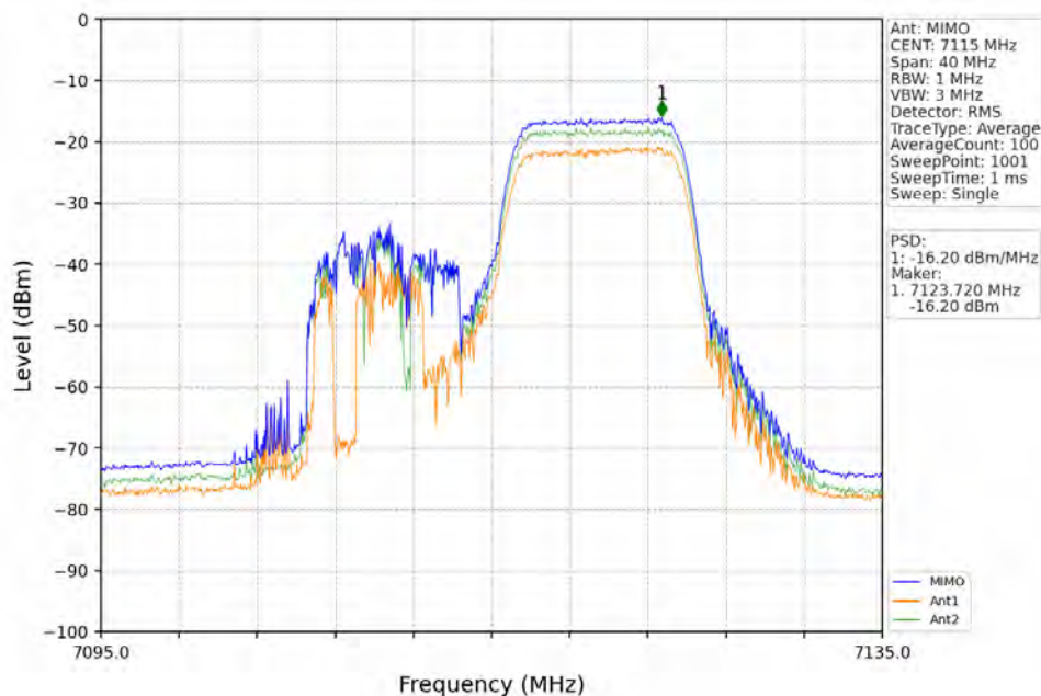
802.11ax(HEW20)_HCH_7115MHz_RU106_Right_MIMO_NTNV
