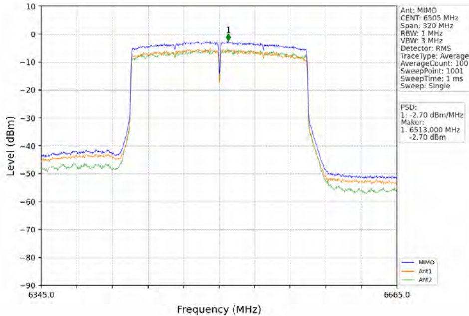
802.11ax(HEW160)_HCH_6505MHz_2xRU996_Left_MIMO_NTNV
