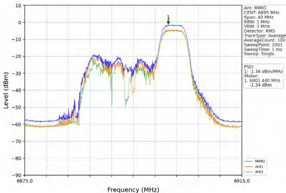
802.11ax(HEW20)_LCH_6895MHz_RU52_Right_MIMO_NTNV
