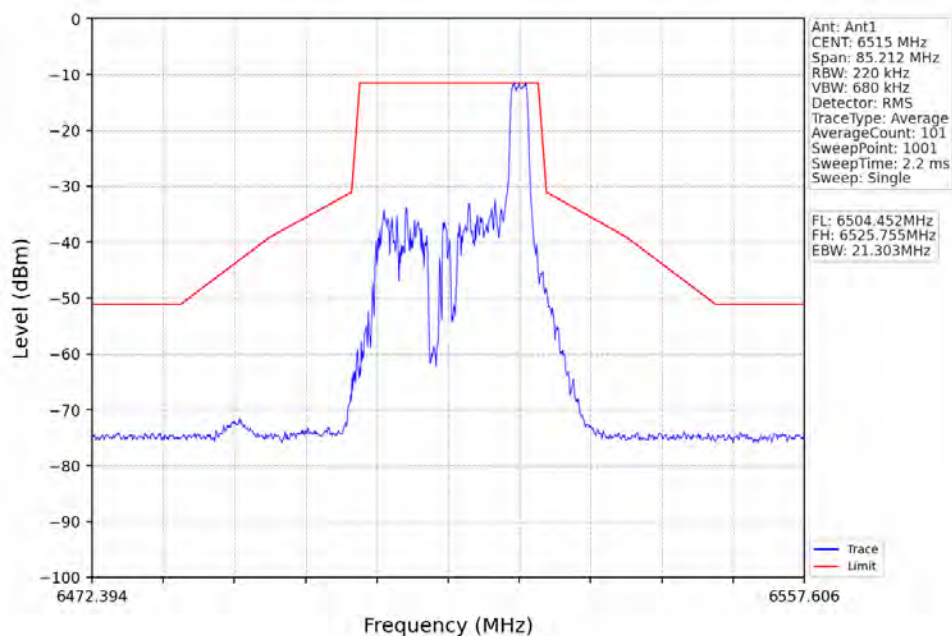
802.11ax(HEW20)_HCH_6515MHz_RU26_Right_Ant1_NTNV
