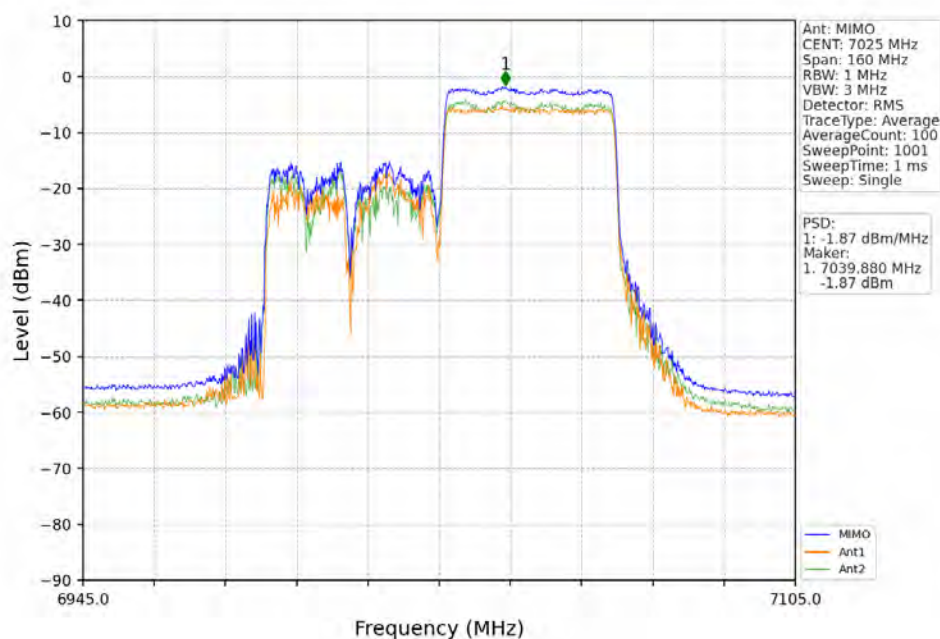
802.11ax(HEW80)_HCH_7025MHz_RU996_Left_MIMO_NTNV
