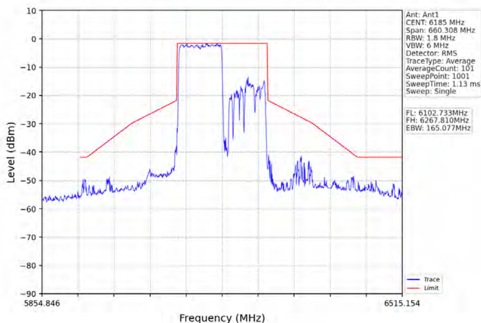
802.11ax(HEW160)_MCH_6185MHz_RU996_Right_Ant1_NTNV
