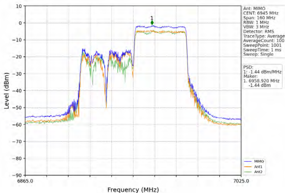
802.11ax(HEW80)_LCH_6945MHz_RU484_Right_MIMO_NTNV
