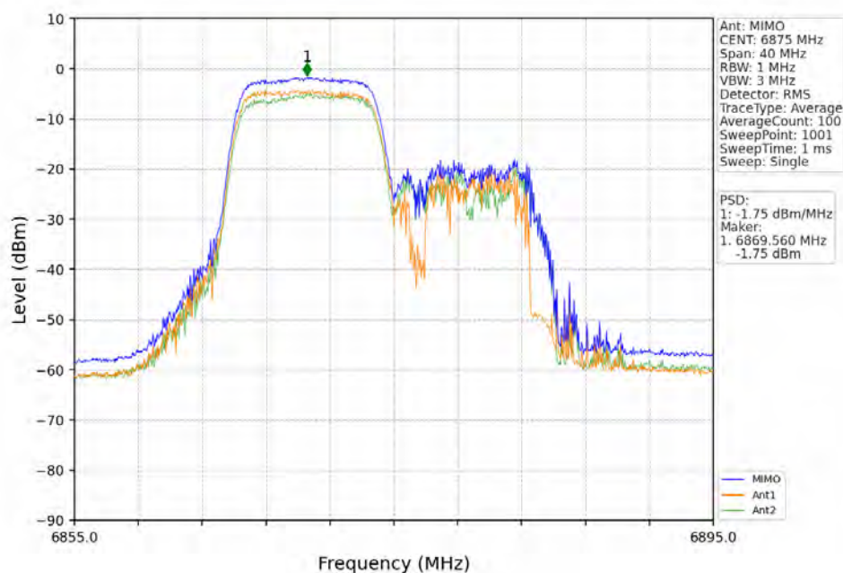
802.11ax(HEW20)_HCH_6875MHz_RU106_Right_MIMO_NTNV
