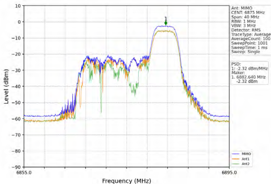
802.11ax(HEW20)_HCH_6875MHz_RU52_Right_MIMO_NTNV
