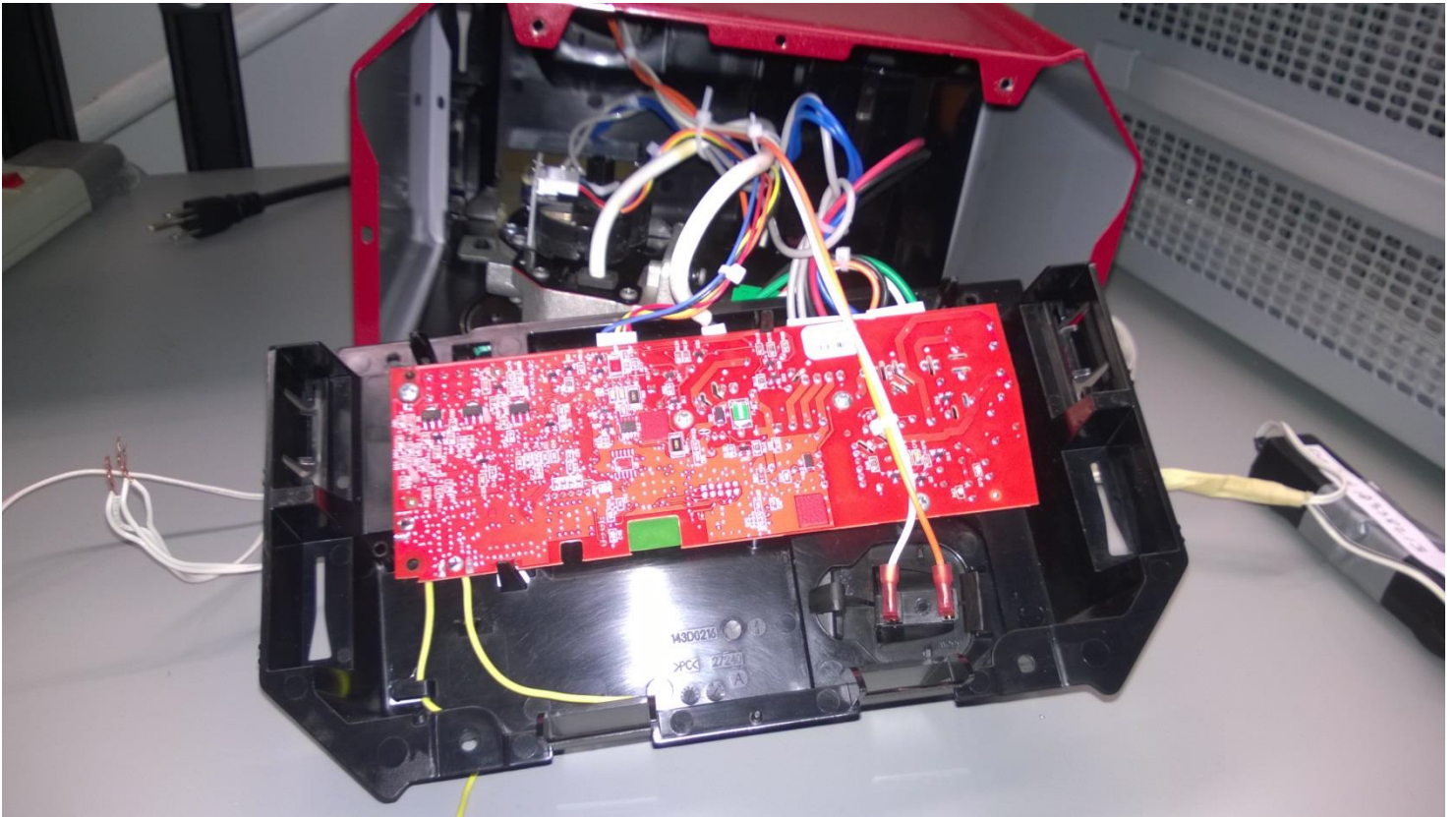
Board installed inside the operator.
