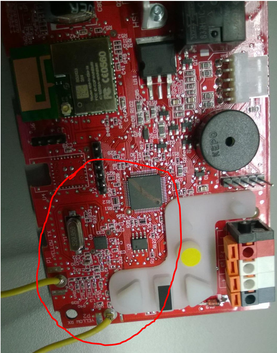
RED Circle – 900MHz Radio Section. Top Yellow Wire on the left is the Transceiver Antenna and yellow wire on the bottom is the RX antenna for 300MHz/400MHz.
