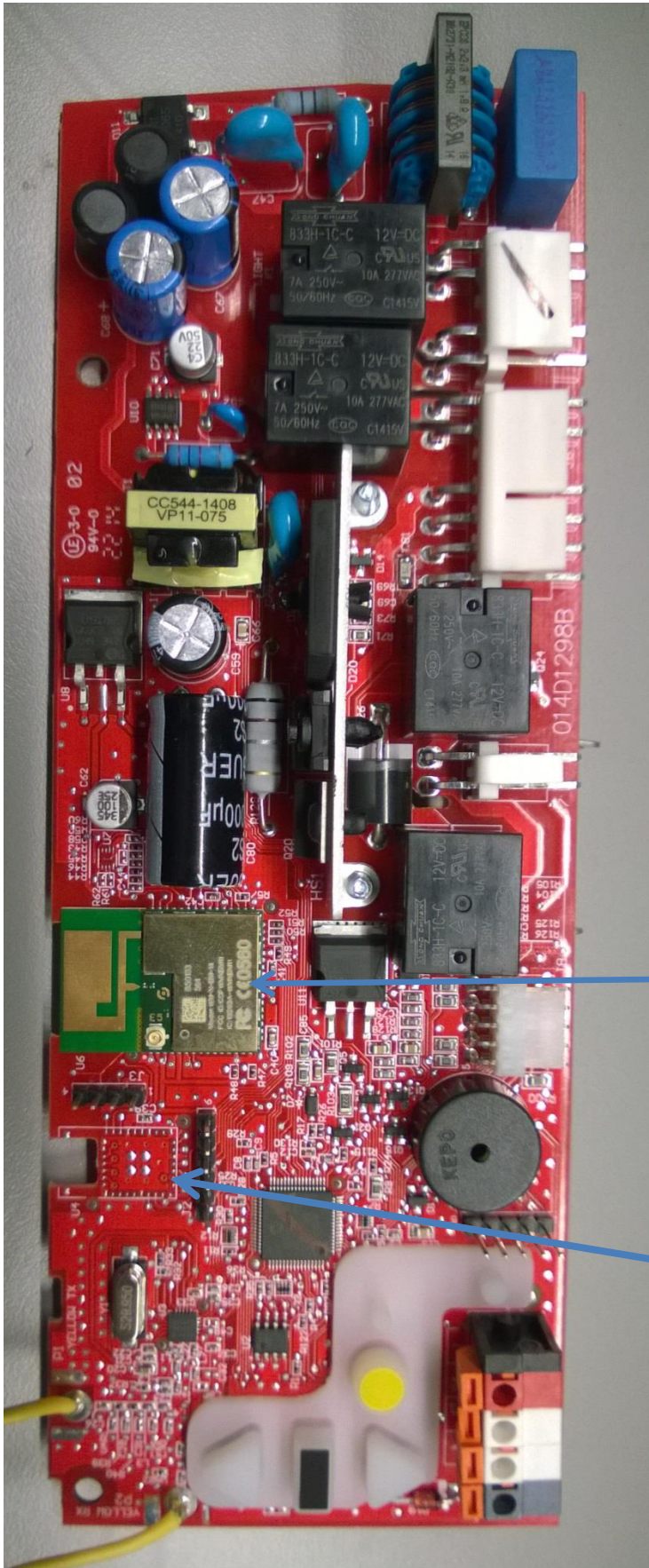
Board – Top View
