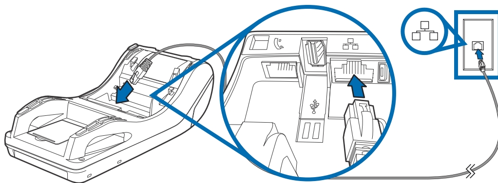
Figure 9 Ethernet Connection
