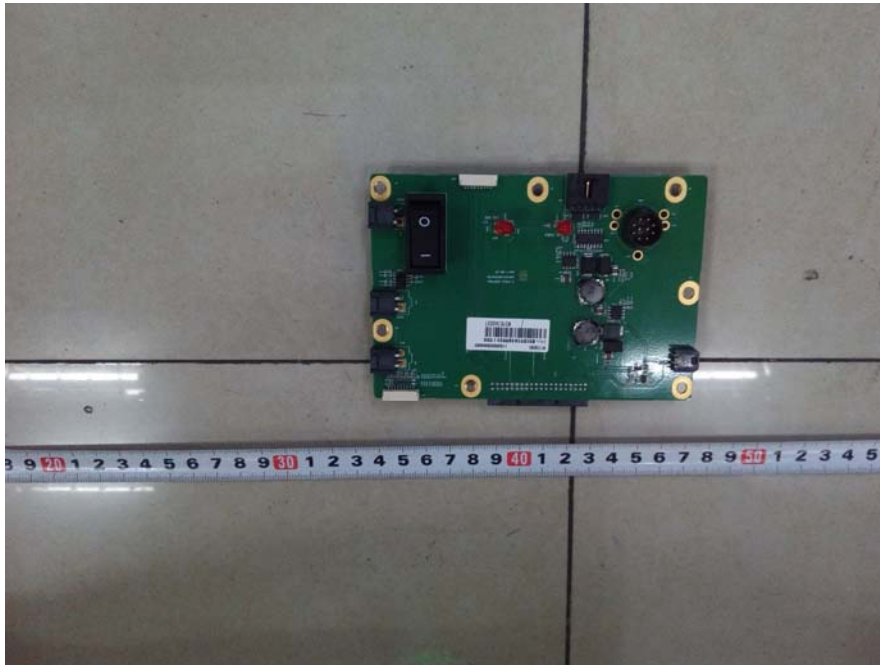
EUT – Controller Board Bottom View
