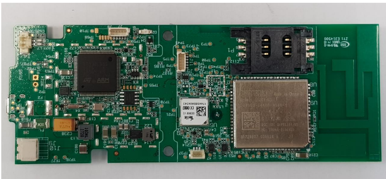
Fig. 8 PC Board Front View with Controller Circuitry Cover Removed
