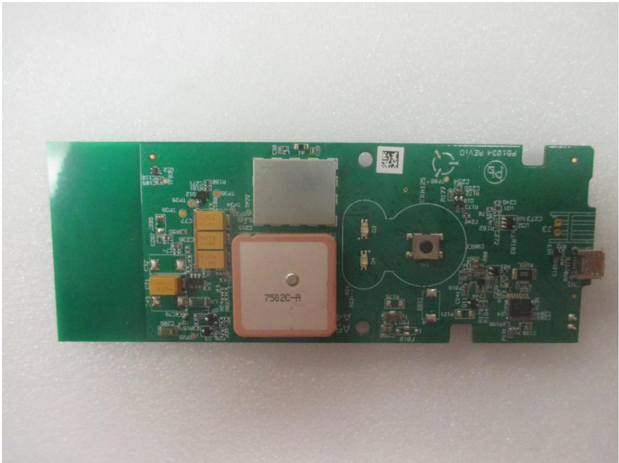
Fig. 9 PC Board Back View
