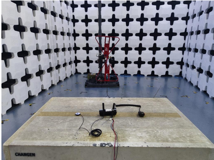
9. Radiated Emissions (Part 22/24/27, 30M-1GHz)
