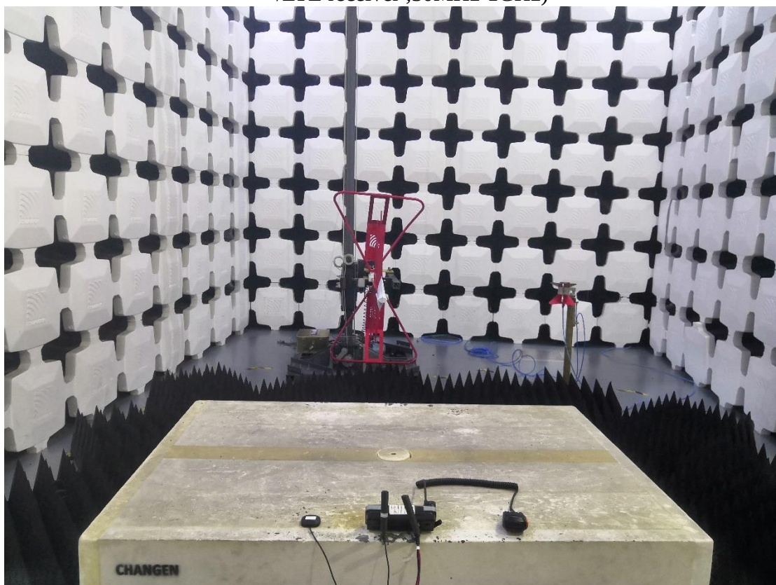
4. Radiated Emissions (Part 15B, Video Player/GSM receiver/WCDMA receiver /LTE receiver,1GHz-18GHz)
