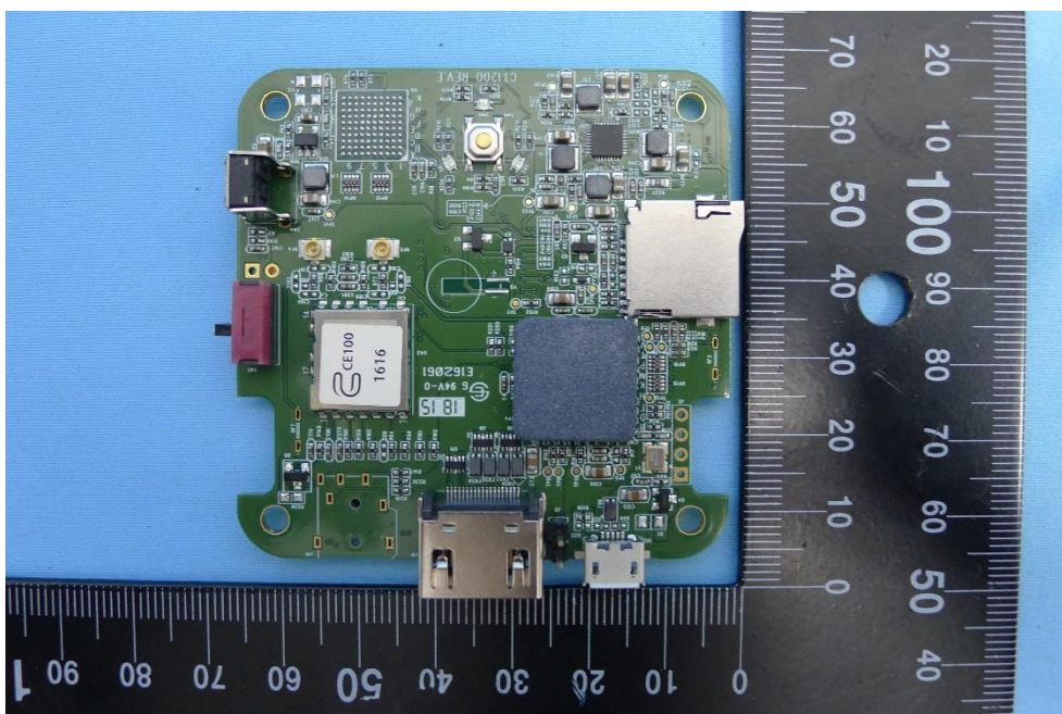
(16) EUT Photo- CT1200 (External Antenna)
