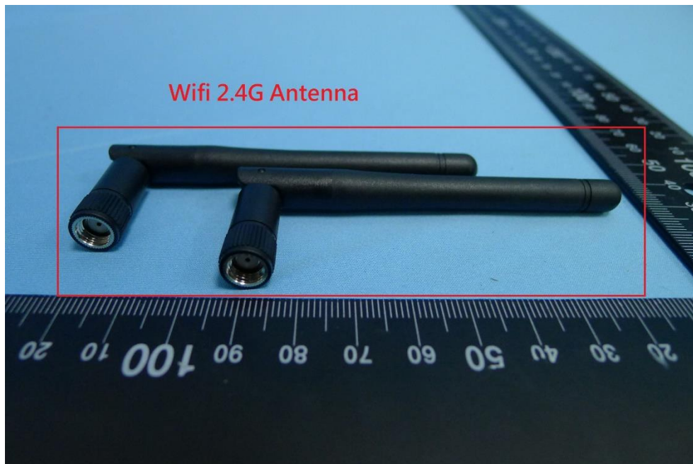
(14) EUT Photo- CT1200 (External Antenna)
