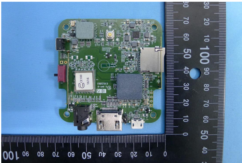
(6) EUT Photo- CT1200 (Internal Antenna)
