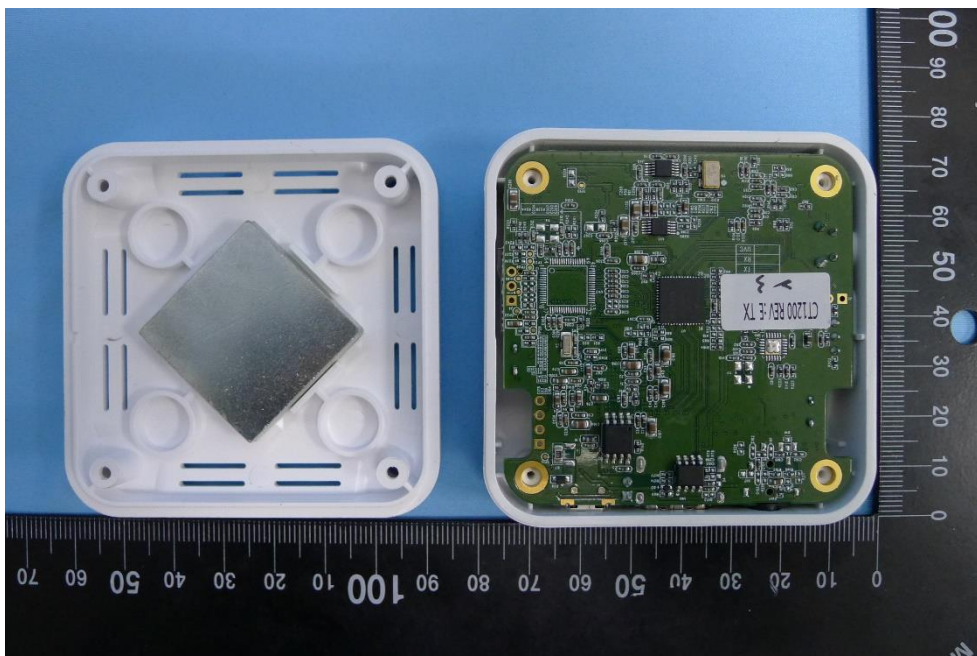
(2) EUT Photo- CT1200 (Internal Antenna)
