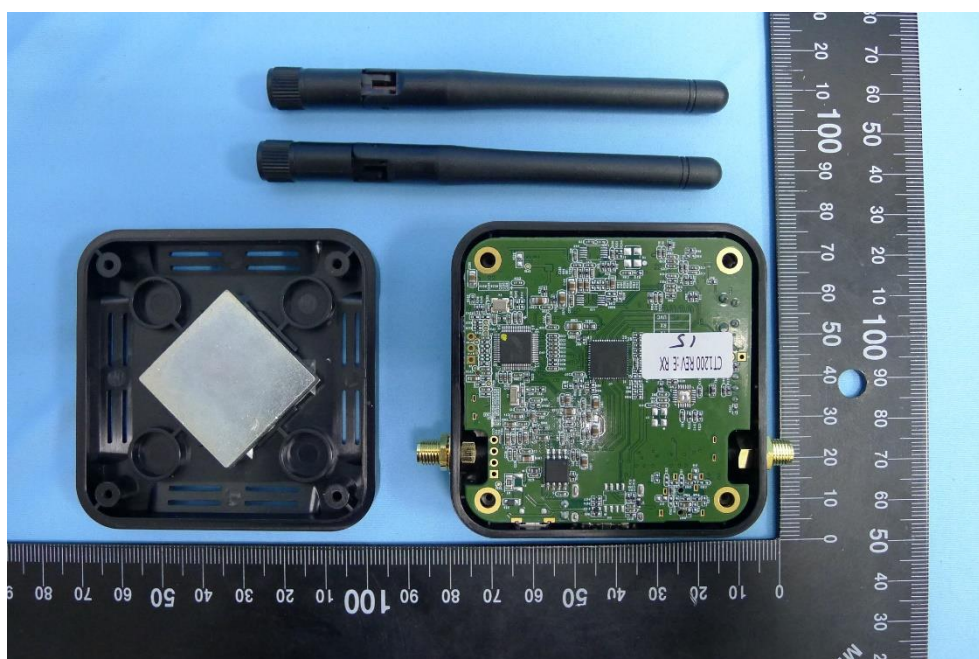
(12) EUT Photo- CT1200 (External Antenna)
