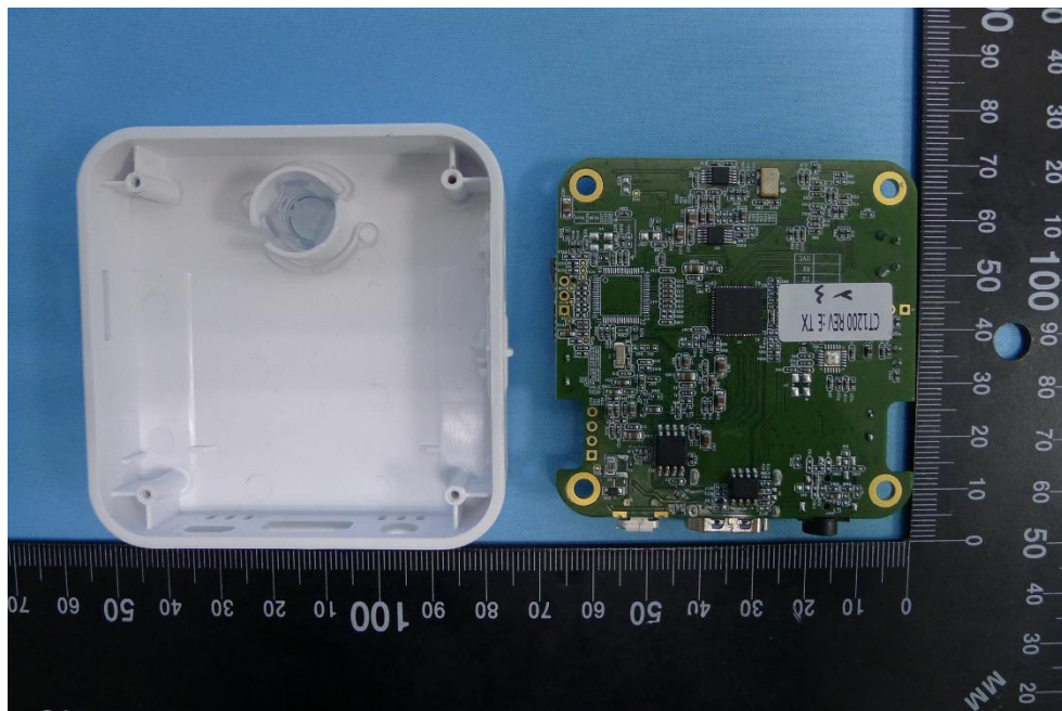
(4) EUT Photo- CT1200 (Internal Antenna)
