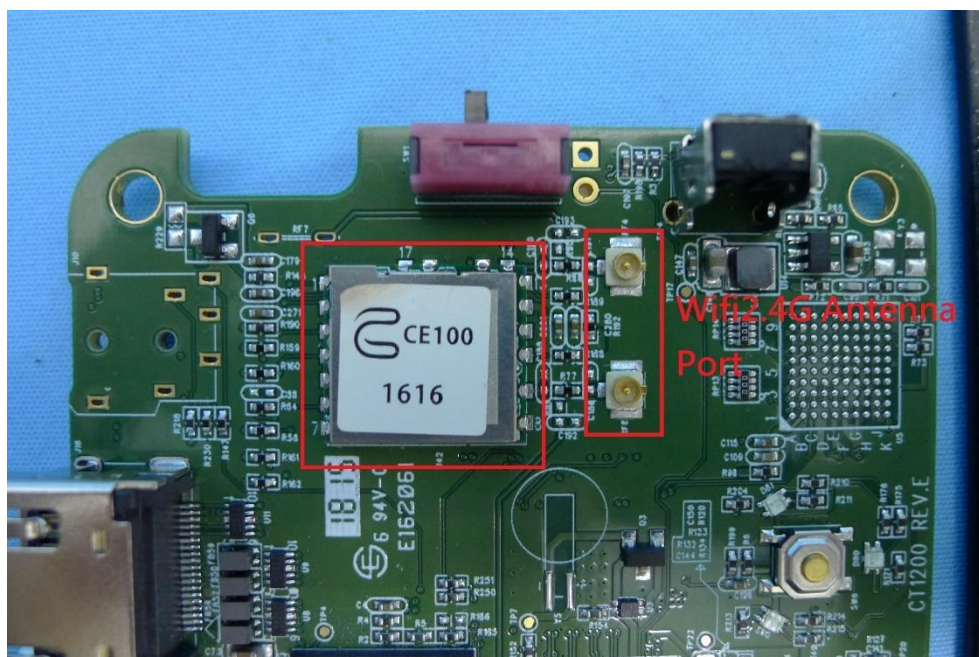
(18) EUT Photo- CT1200 (External Antenna)
