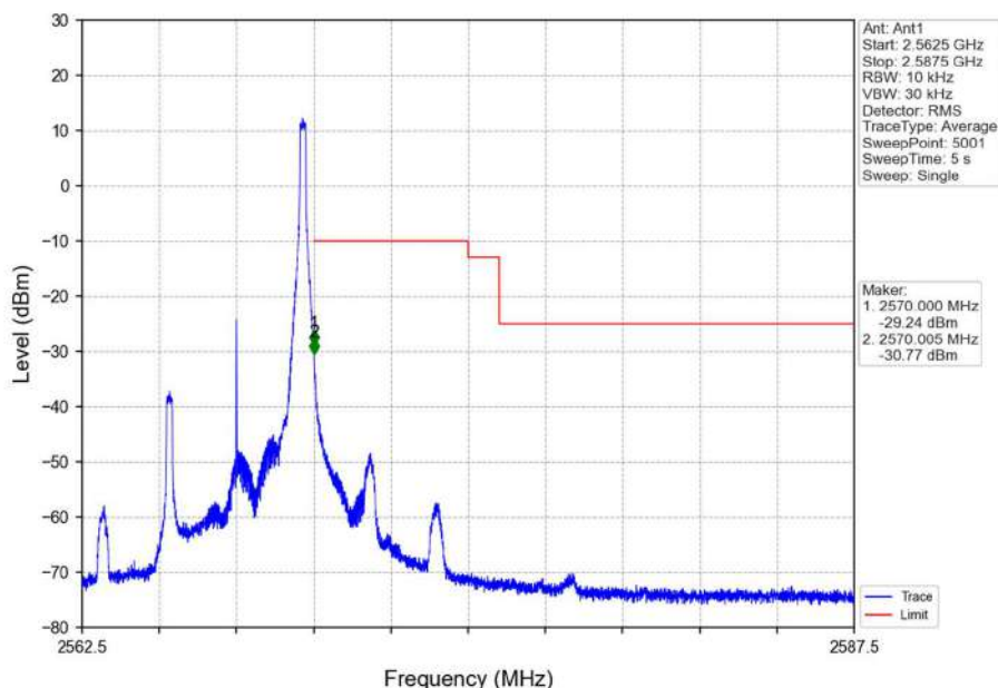
Band7_5MHz_16QAM_HCH_2567.5MHz_RB_1_24_NTNV
