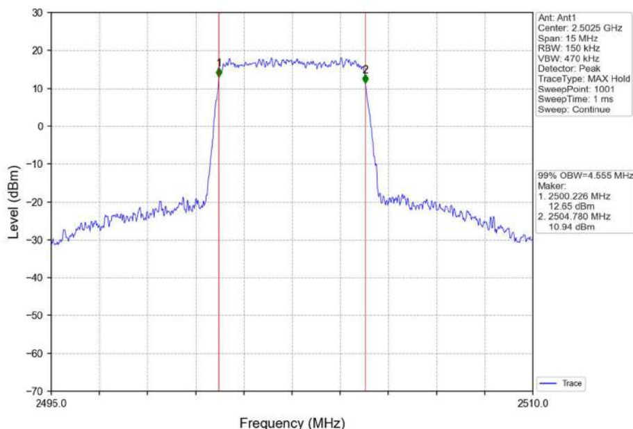
Band7_5MHz_16QAM_LCH_2502.5MHz_RB_25_0_NTNV
