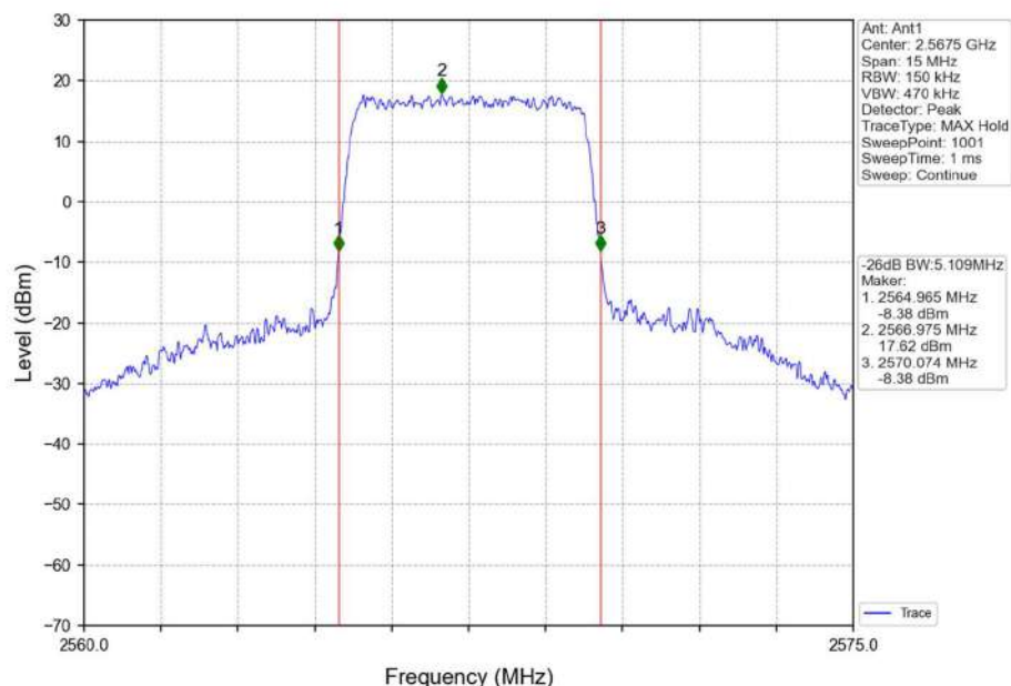
Band7_5MHz_16QAM_HCH_2567.5MHz_RB_25_0_NTNV
