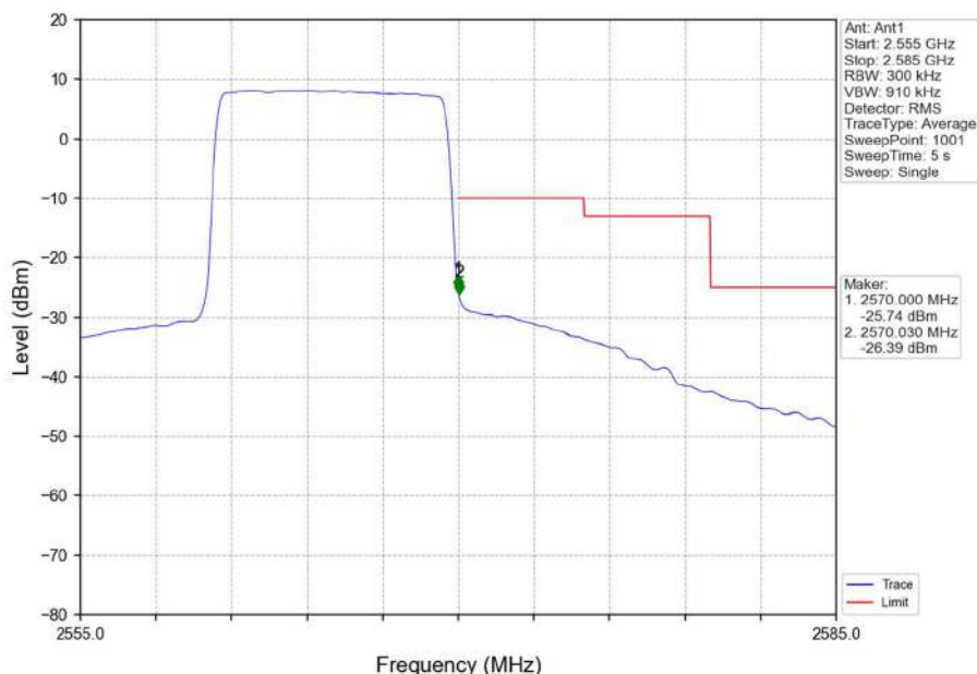
Band7_10MHz_16QAM_HCH_2565MHz_RB_50_0_NTNV
