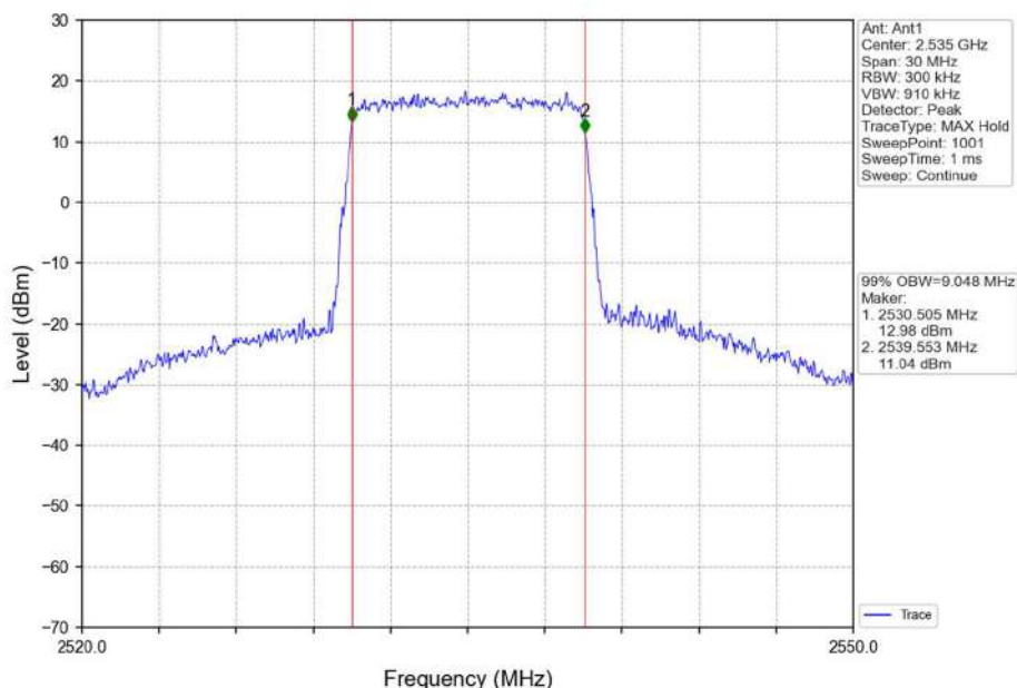
Band7_10MHz_16QAM_MCH_2535MHz_RB_50_0_NTNV
