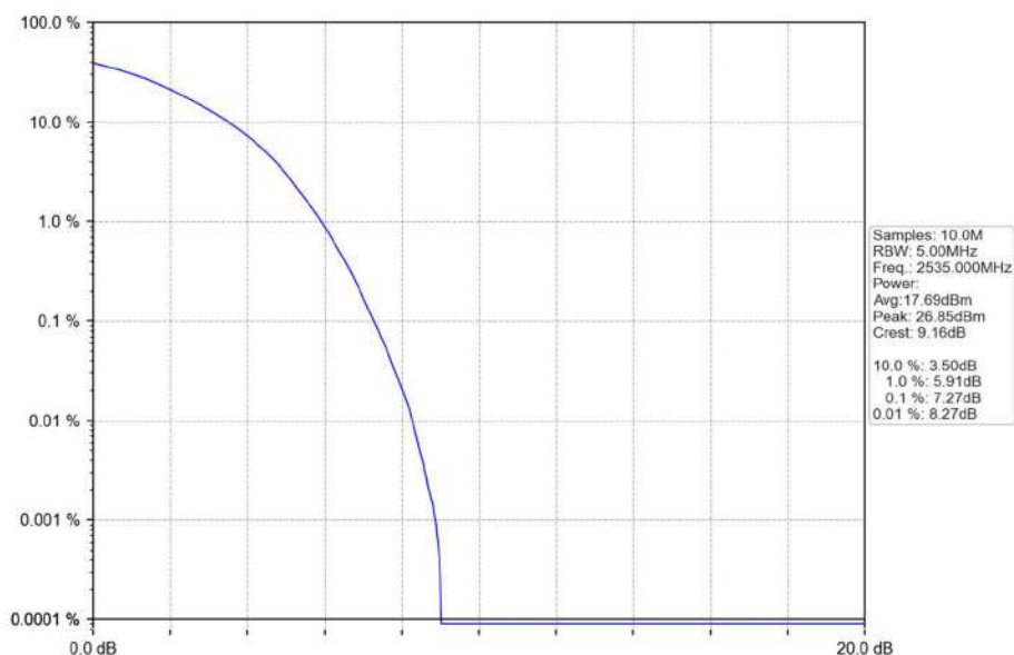
Band7_15MHz_16QAM_MCH_2535MHz_RB_75_0_NTNV
