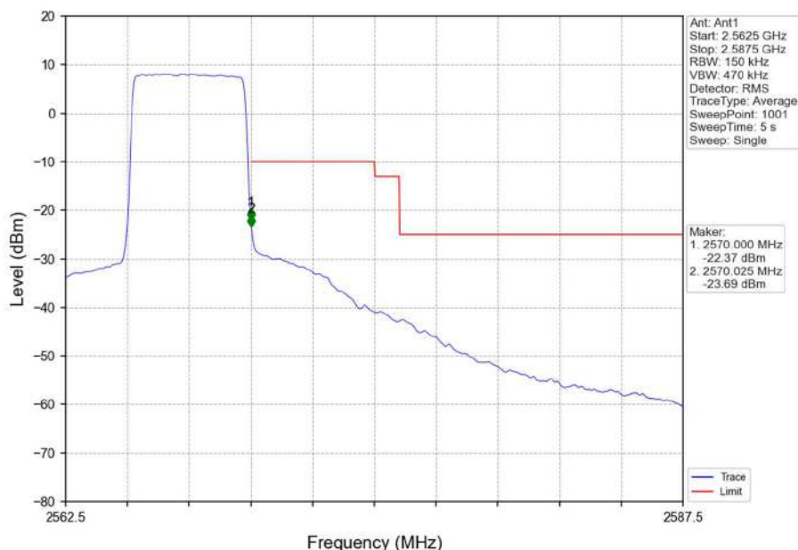
Band7_5MHz_16QAM_HCH_2567.5MHz_RB_25_0_NTNV
