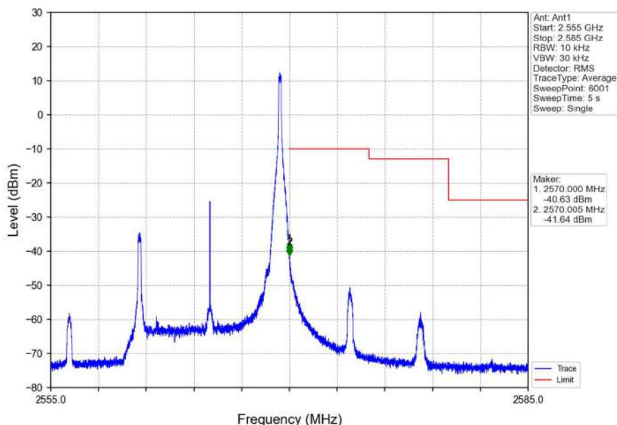
Band7_10MHz_16QAM_HCH_2565MHz_RB_1_49_NTNV
