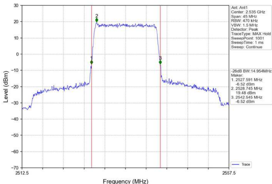
Band7_15MHz_QPSK_MCH_2535MHz_RB_75_0_NTNV
