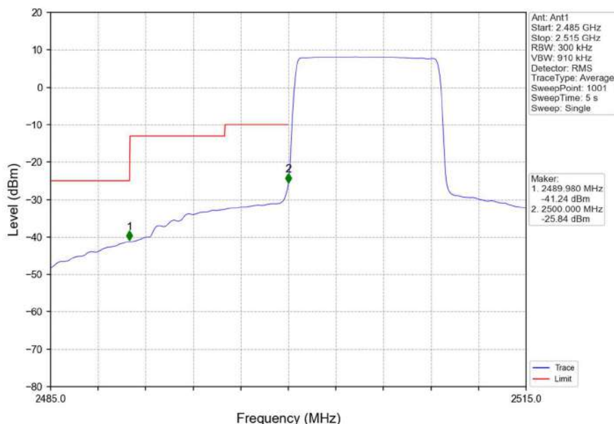
Band7_10MHz_16QAM_LCH_2505MHz_RB_50_0_NTNV
