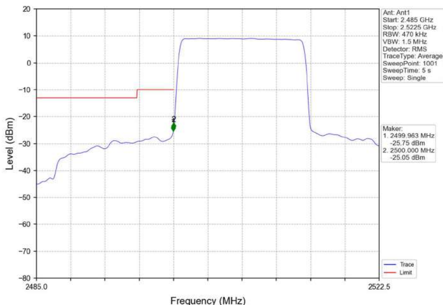
Band7_15MHz_QPSK_LCH_2507.5MHz_RB_75_0_NTNV
