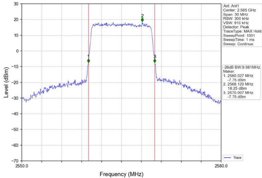
Band7_10MHz_16QAM_HCH_2565MHz_RB_50_0_NTNV
