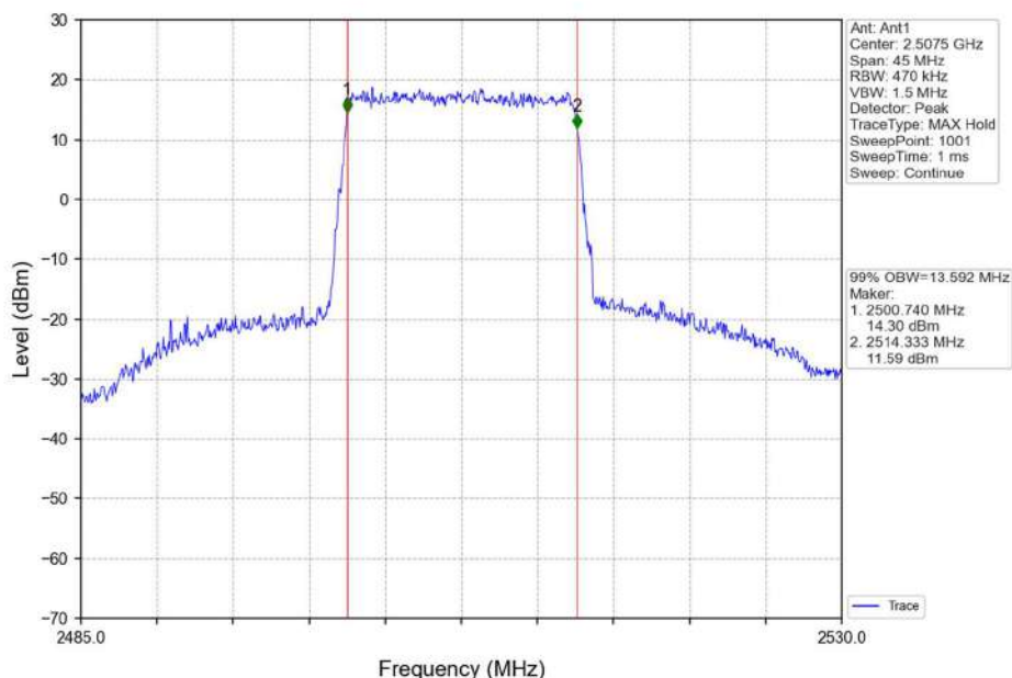
Band7_15MHz_16QAM_LCH_2507.5MHz_RB_75_0_NTNV
