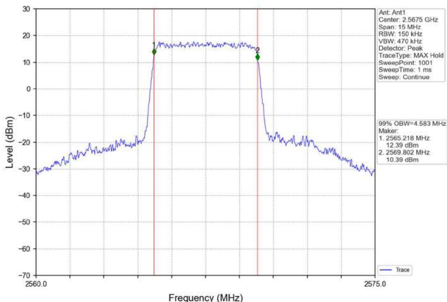
Band7_5MHz_16QAM_HCH_2567.5MHz_RB_25_0_NTNV
