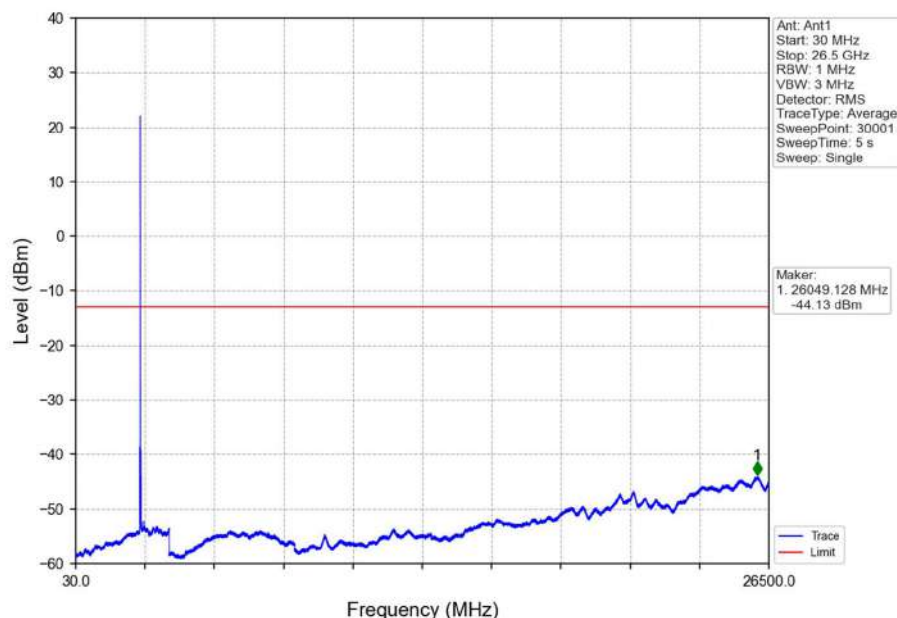
Band7_15MHz_QPSK_LCH_2507.5MHz_RB_1_0_NTNV
