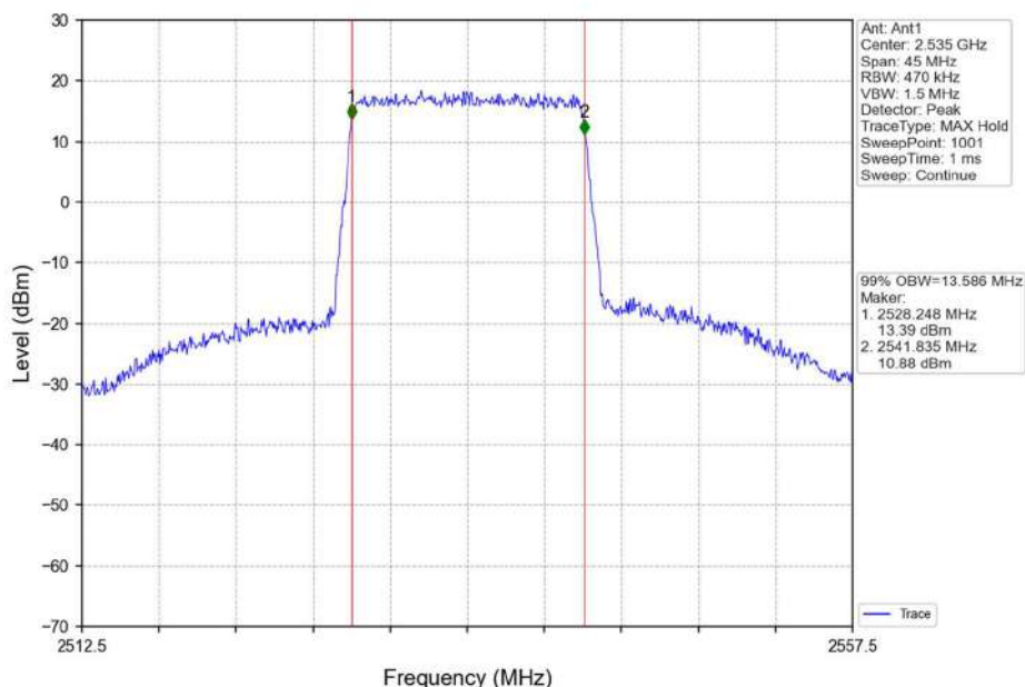
Band7_15MHz_16QAM_MCH_2535MHz_RB_75_0_NTNV
