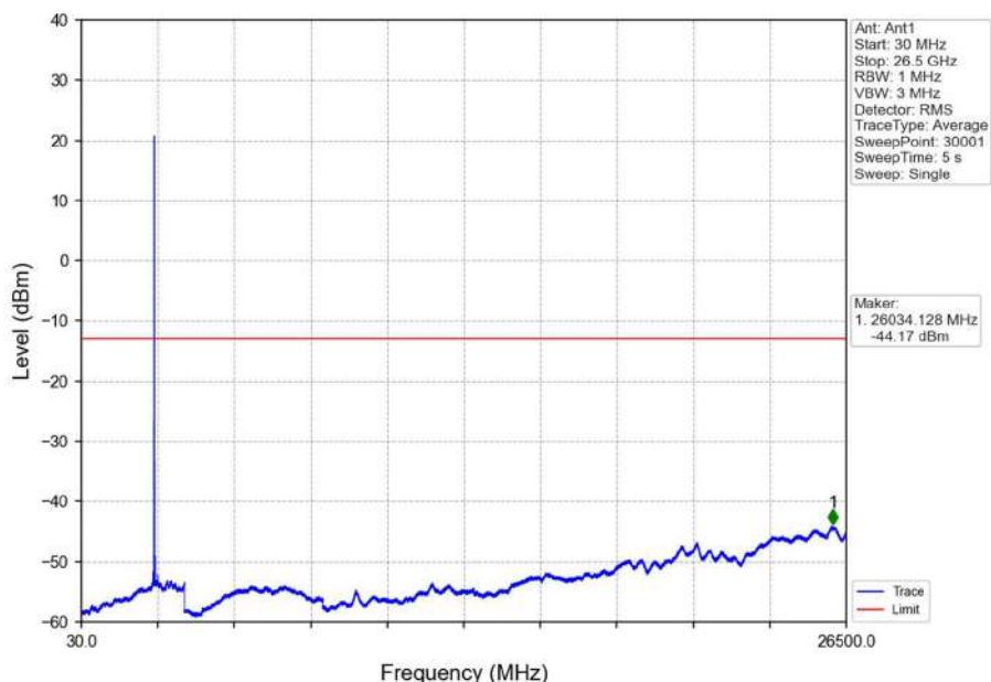
Band7_15MHz_16QAM_HCH_2562.5MHz_RB_1_0_NTNV
