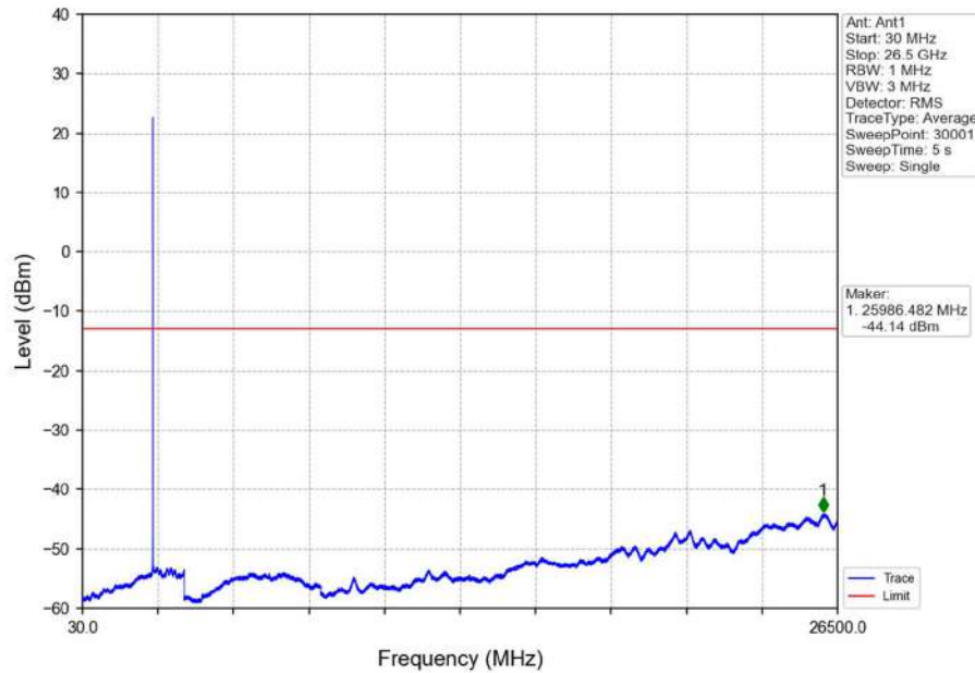
Band7_5MHz_16QAM_LCH_2502.5MHz_RB_1_0_NTNV
