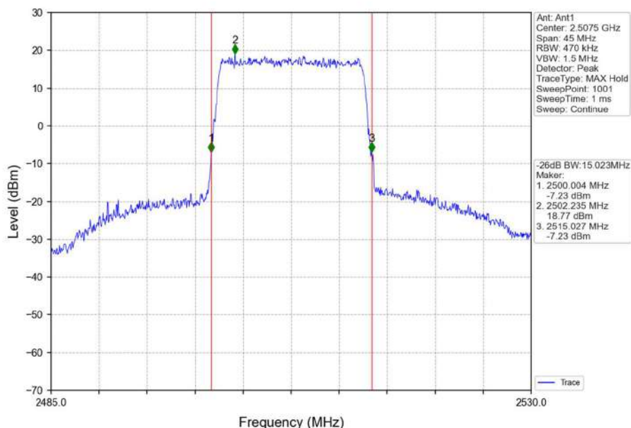
Band7_15MHz_16QAM_LCH_2507.5MHz_RB_75_0_NTNV
