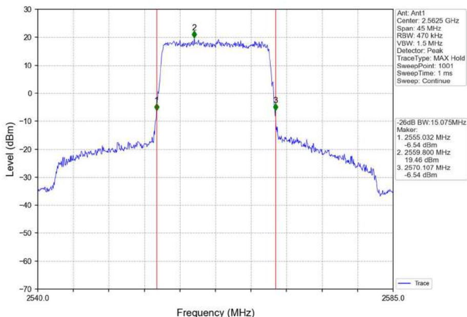
Band7_15MHz_QPSK_HCH_2562.5MHz_RB_75_0_NTNV
