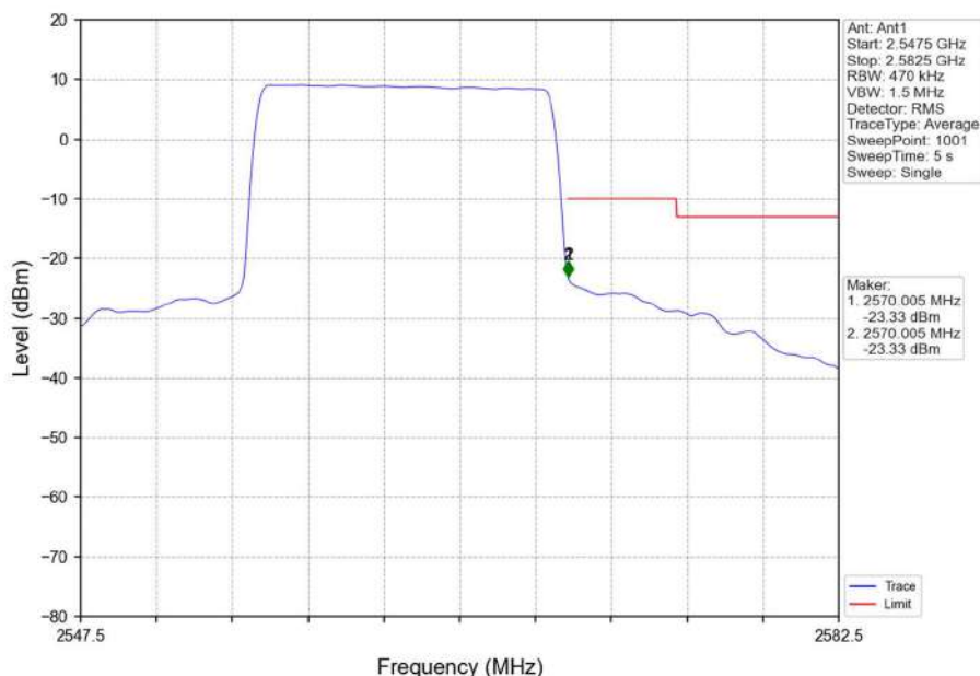
Band7_15MHz_QPSK_HCH_2562.5MHz_RB_75_0_NTNV
