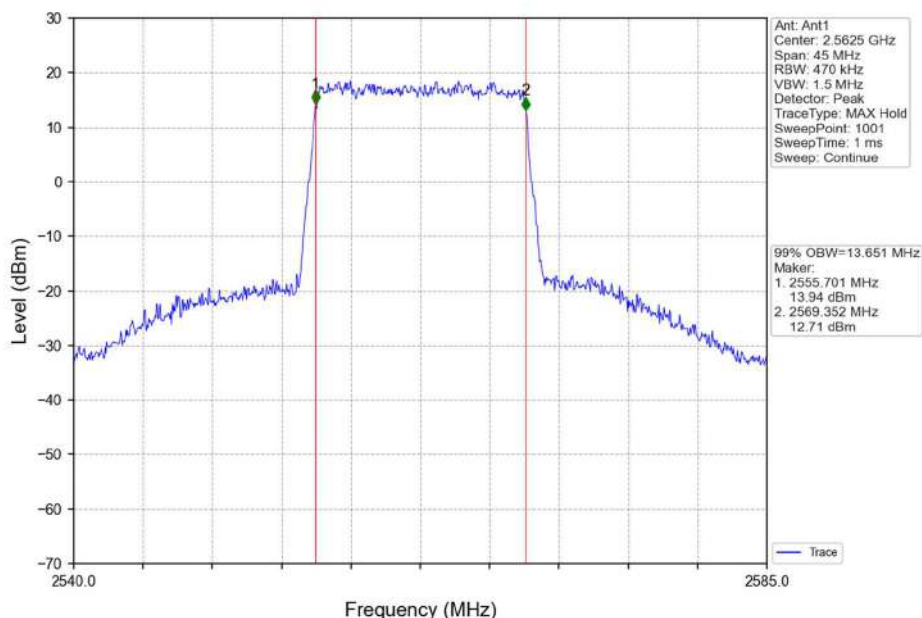
Band7_15MHz_16QAM_HCH_2562.5MHz_RB_75_0_NTNV
