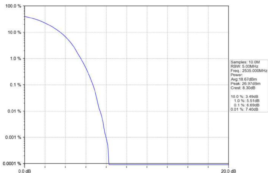
Band7_15MHz_QPSK_MCH_2535MHz_RB_75_0_NTNV
