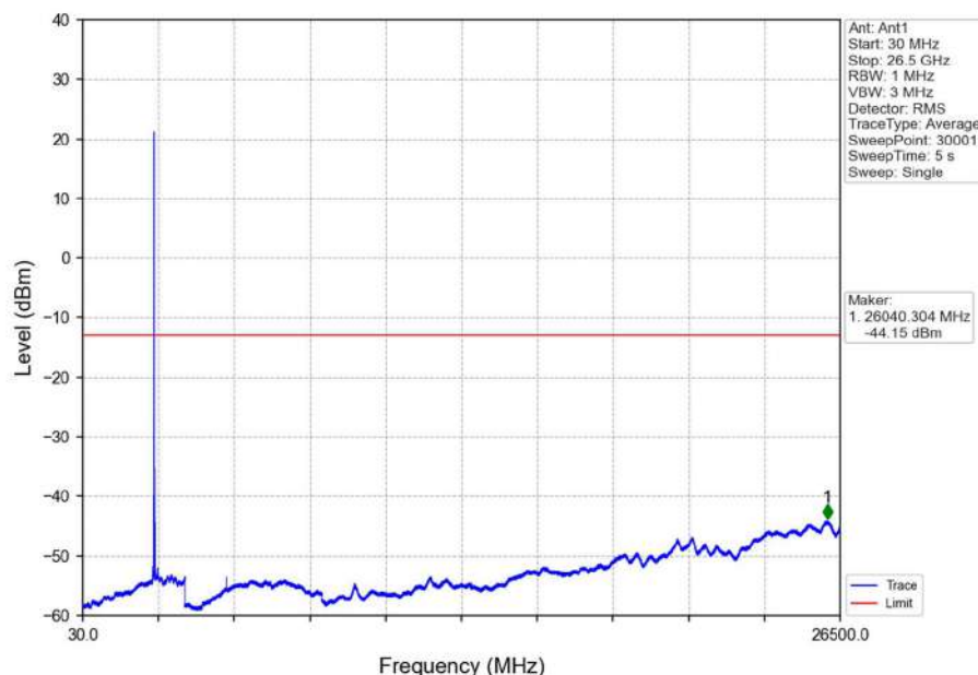
Band7_15MHz_QPSK_MCH_2535MHz_RB_1_0_NTNV
