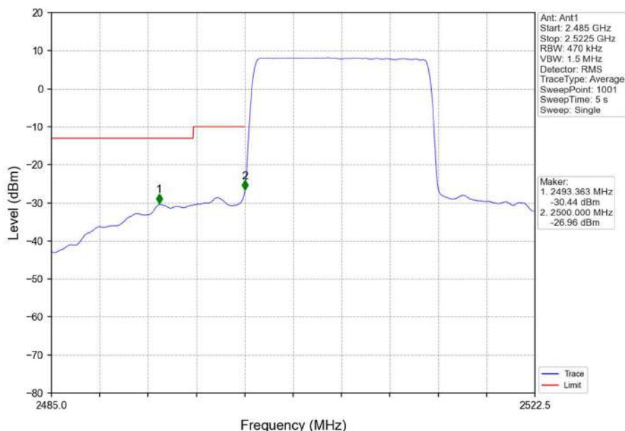
Band7_15MHz_16QAM_LCH_2507.5MHz_RB_75_0_NTNV
