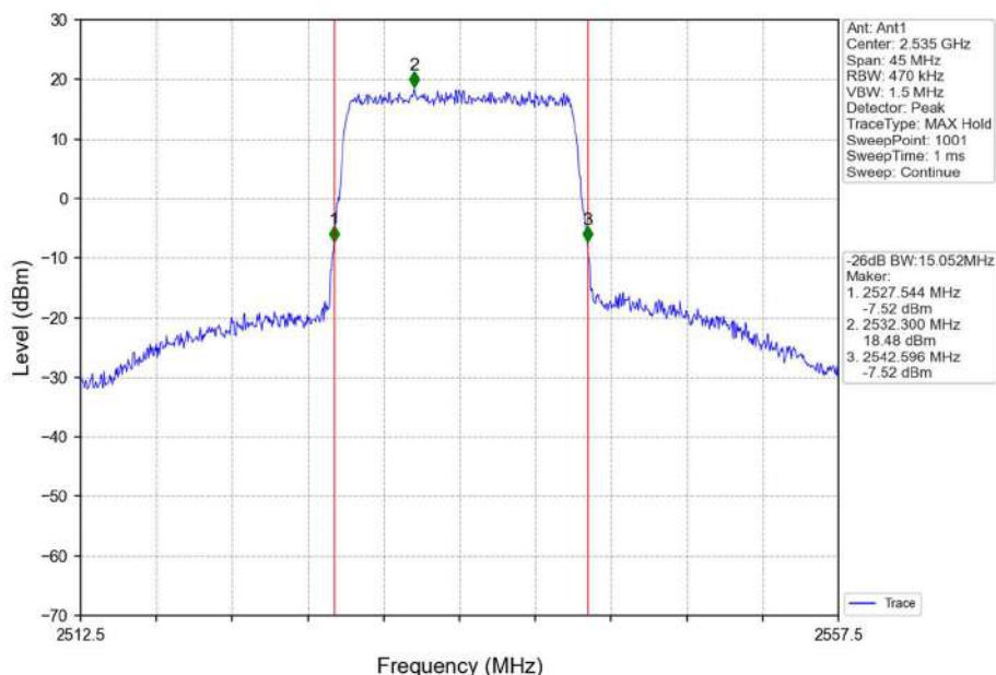
Band7_15MHz_16QAM_MCH_2535MHz_RB_75_0_NTNV
