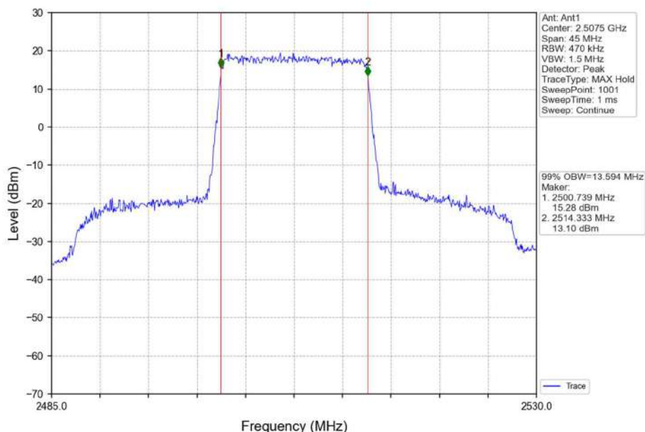
Band7_15MHz_QPSK_LCH_2507.5MHz_RB_75_0_NTNV
