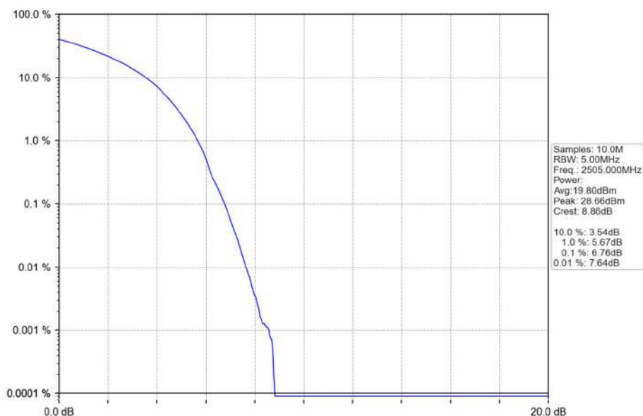
Band7_10MHz_16QAM_LCH_2505MHz_RB_50_0_NTNV
