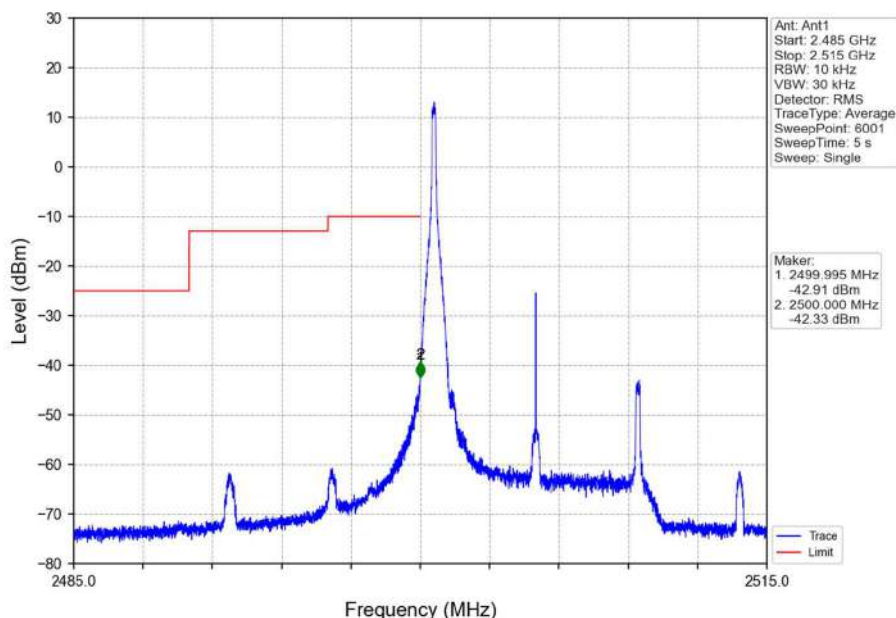
Band7_10MHz_16QAM_LCH_2505MHz_RB_1_0_NTNV
