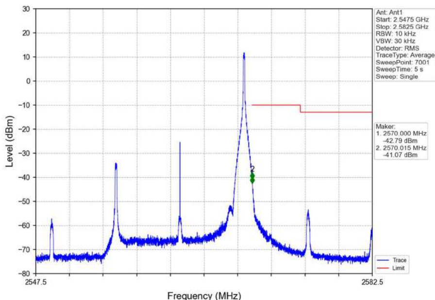
Band7_15MHz_16QAM_HCH_2562.5MHz_RB_1_74_NTNV
