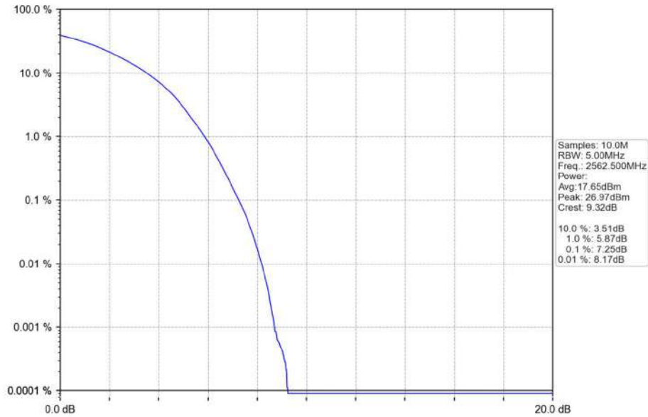
Band7_15MHz_16QAM_HCH_2562.5MHz_RB_75_0_NTNV
