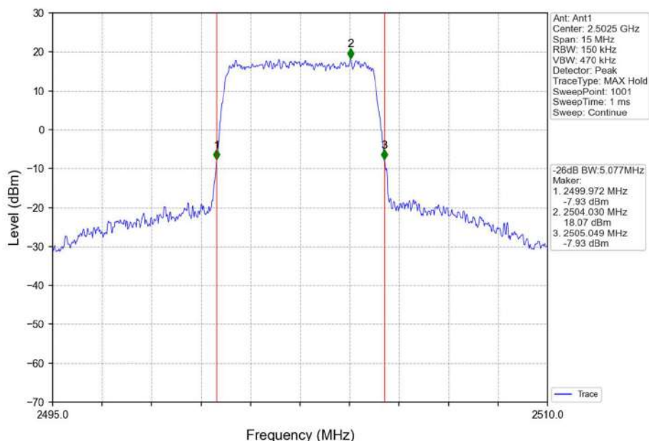
Band7_5MHz_16QAM_LCH_2502.5MHz_RB_25_0_NTNV
