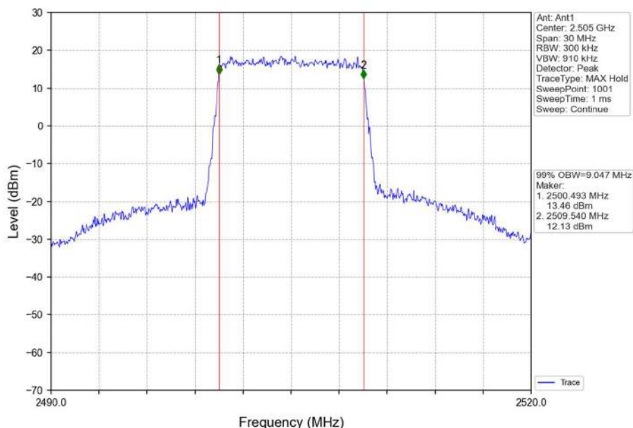
Band7_10MHz_16QAM_LCH_2505MHz_RB_50_0_NTNV
