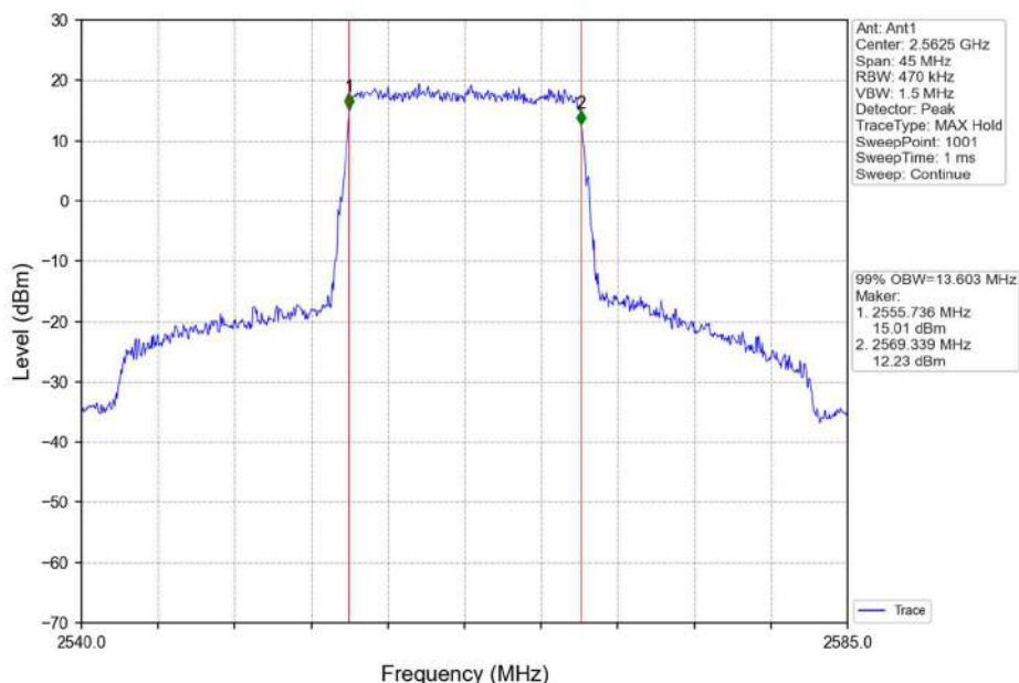
Band7_15MHz_QPSK_HCH_2562.5MHz_RB_75_0_NTNV
