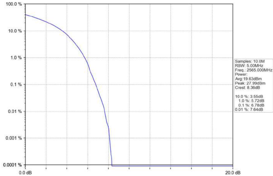
Band7_10MHz_16QAM_HCH_2565MHz_RB_50_0_NTNV
