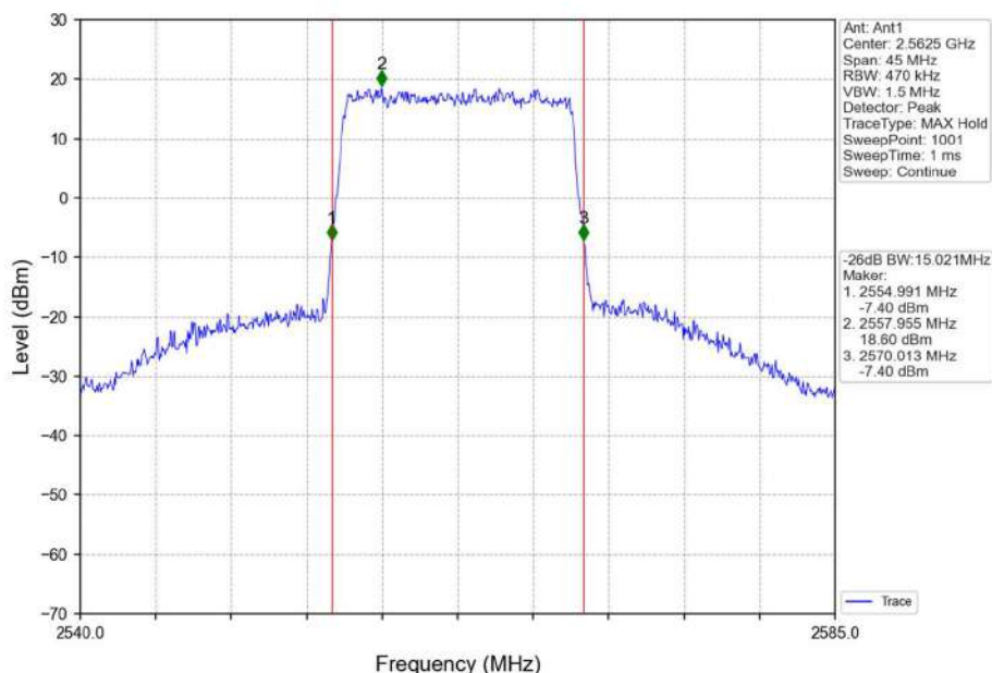
Band7_15MHz_16QAM_HCH_2562.5MHz_RB_75_0_NTNV
