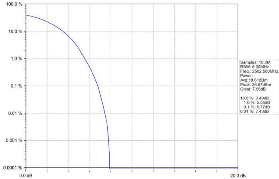
Band7_15MHz_QPSK_HCH_2562.5MHz_RB_75_0_NTNV
