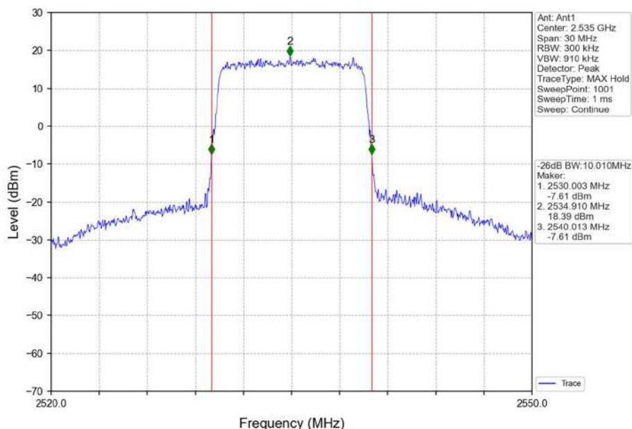
Band7_10MHz_16QAM_MCH_2535MHz_RB_50_0_NTNV
