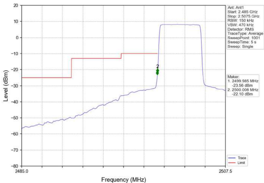
Band7_5MHz_16QAM_LCH_2502.5MHz_RB_25_0_NTNV
