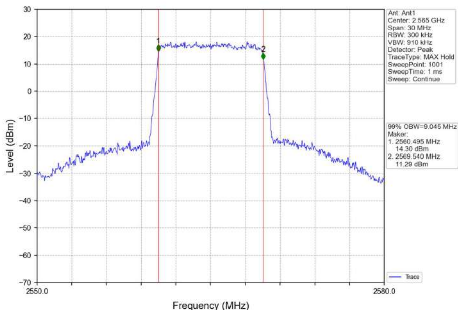
Band7_10MHz_16QAM_HCH_2565MHz_RB_50_0_NTNV
