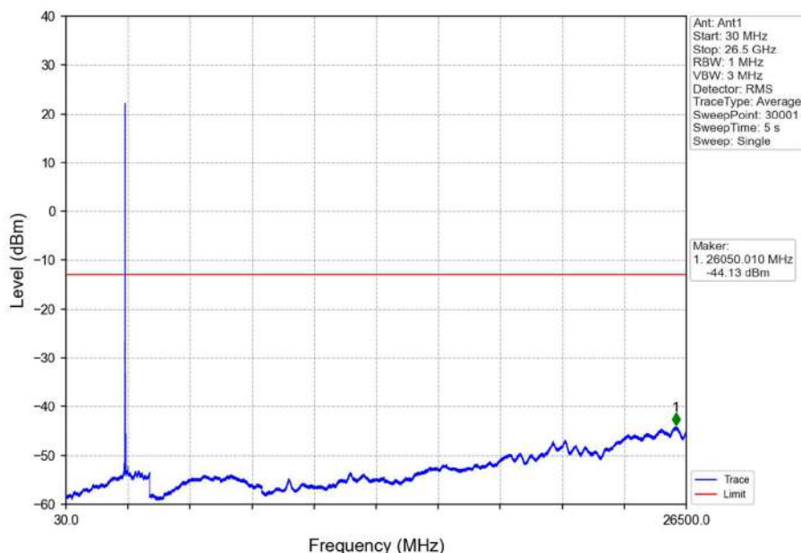
Band7_15MHz_QPSK_HCH_2562.5MHz_RB_1_0_NTNV
