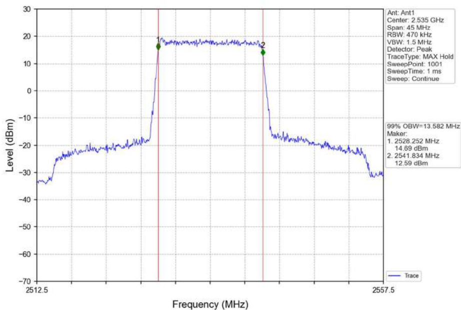
Band7_15MHz_QPSK_MCH_2535MHz_RB_75_0_NTNV
