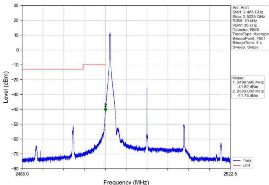
Band7_15MHz_16QAM_LCH_2507.5MHz_RB_1_0_NTNV
