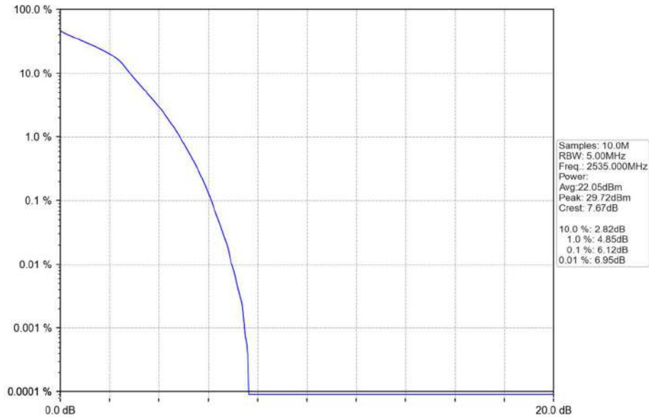
Band7_5MHz_16QAM_MCH_2535MHz_RB_25_0_NTNV
