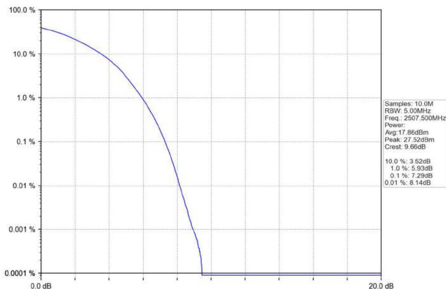
Band7_15MHz_16QAM_LCH_2507.5MHz_RB_75_0_NTNV
