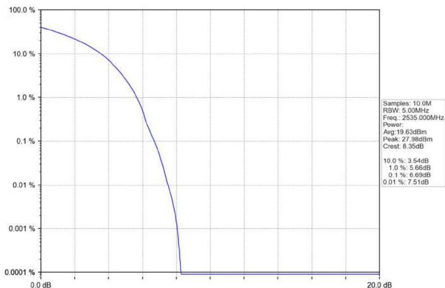
Band7_10MHz_16QAM_MCH_2535MHz_RB_50_0_NTNV
