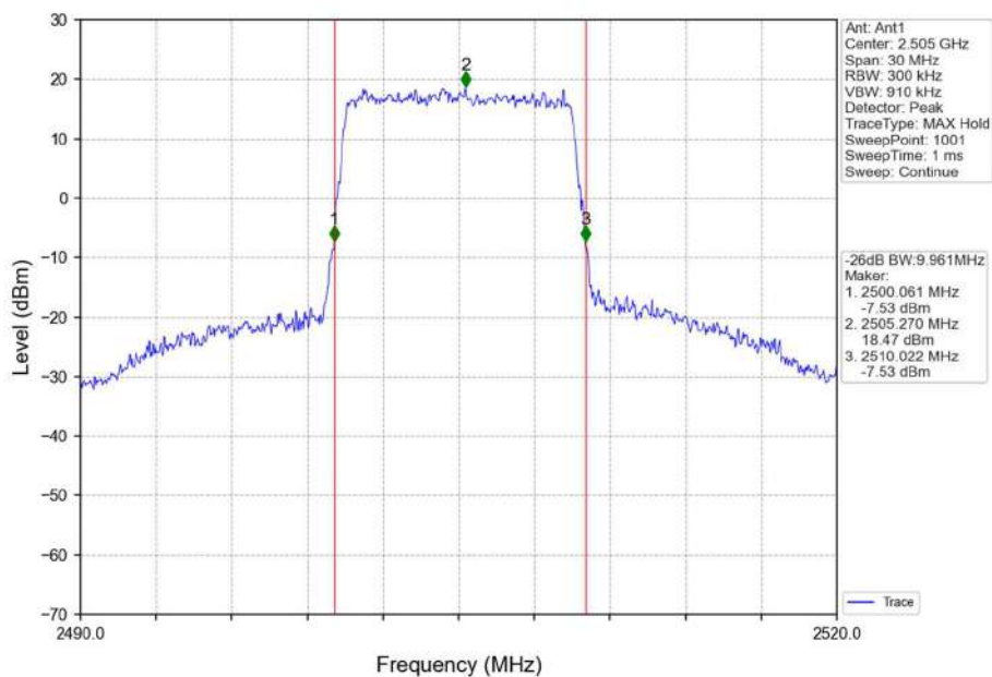
Band7_10MHz_16QAM_LCH_2505MHz_RB_50_0_NTNV
