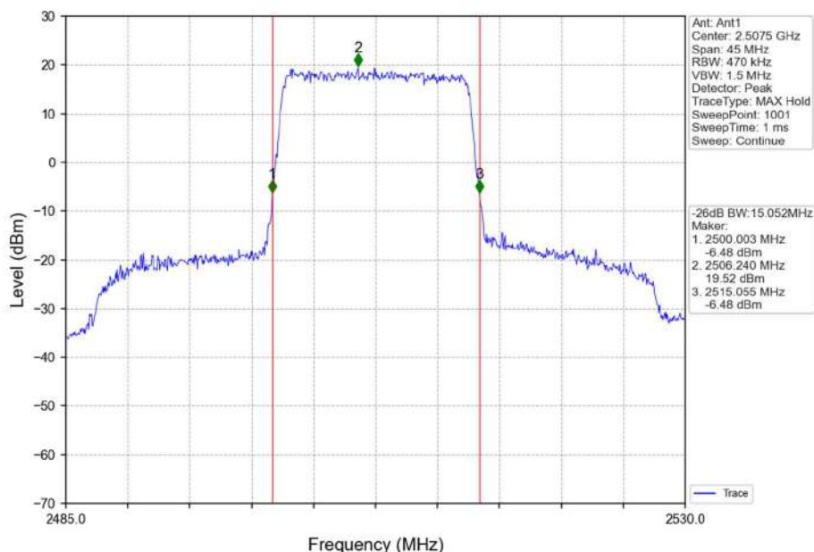
Band7_15MHz_QPSK_LCH_2507.5MHz_RB_75_0_NTNV
