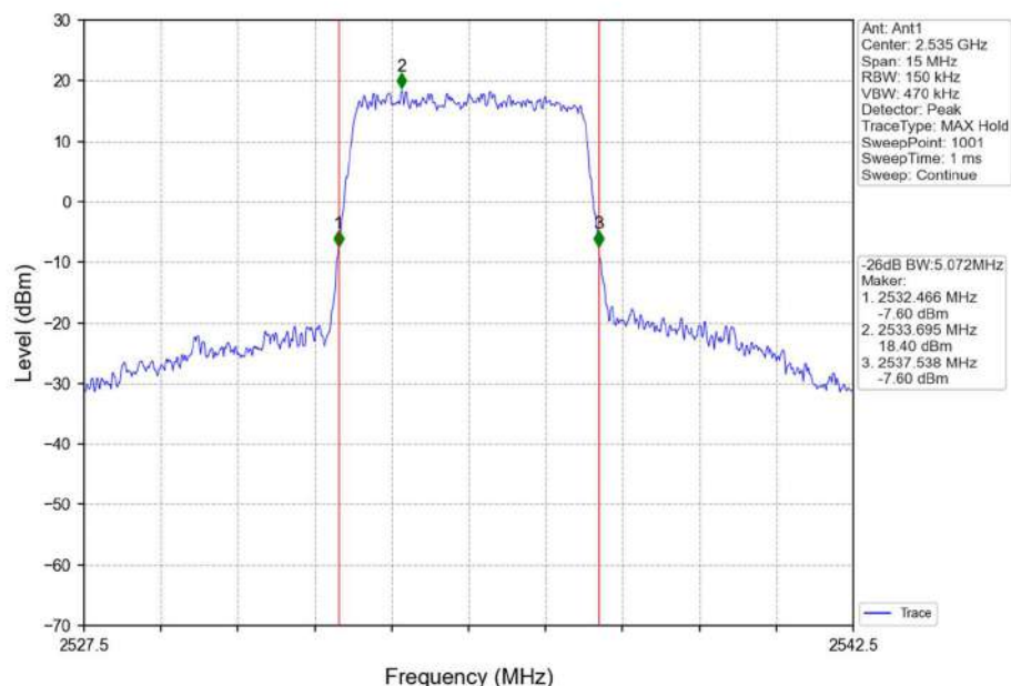
Band7_5MHz_16QAM_MCH_2535MHz_RB_25_0_NTNV
