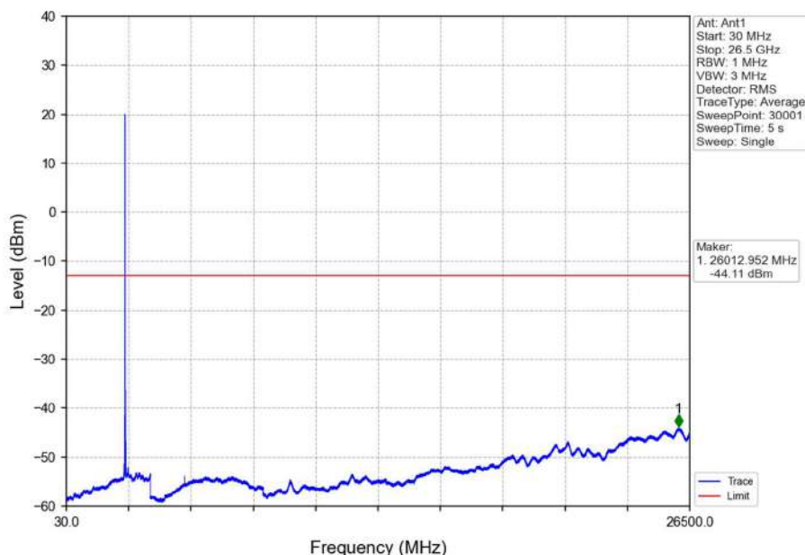
Band7_15MHz_16QAM_MCH_2535MHz_RB_1_0_NTNV
