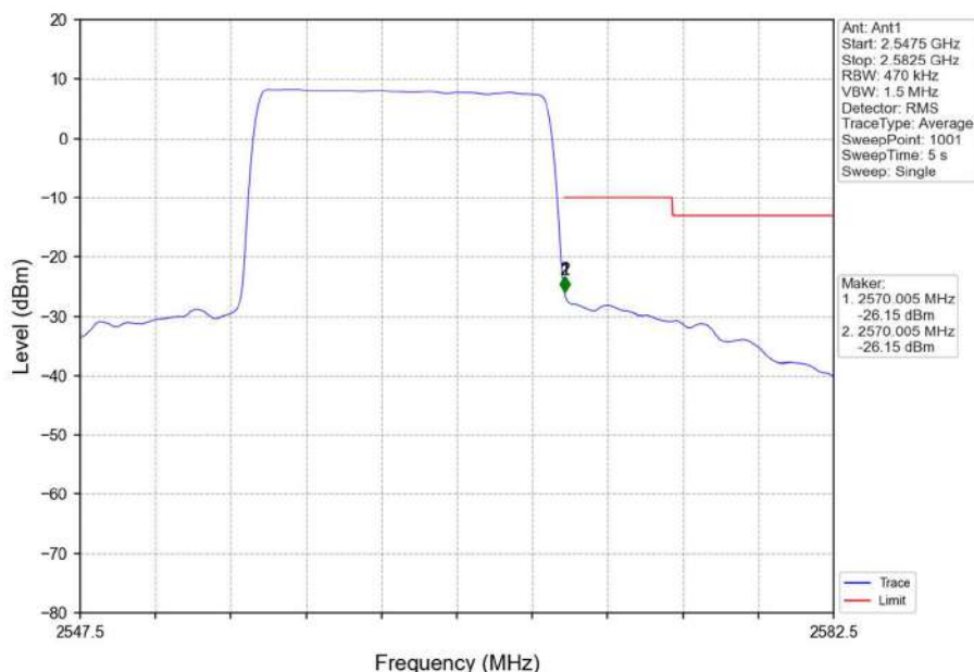
Band7_15MHz_16QAM_HCH_2562.5MHz_RB_75_0_NTNV
