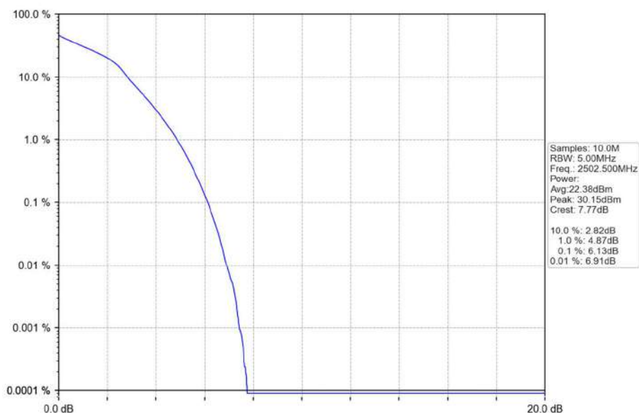
Band7_5MHz_16QAM_LCH_2502.5MHz_RB_25_0_NTNV
