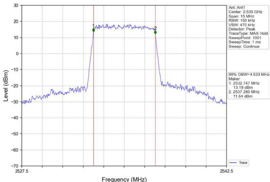
Band7_5MHz_16QAM_MCH_2535MHz_RB_25_0_NTNV
