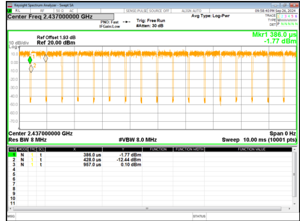
(802.11 n40) plot on channel 6
