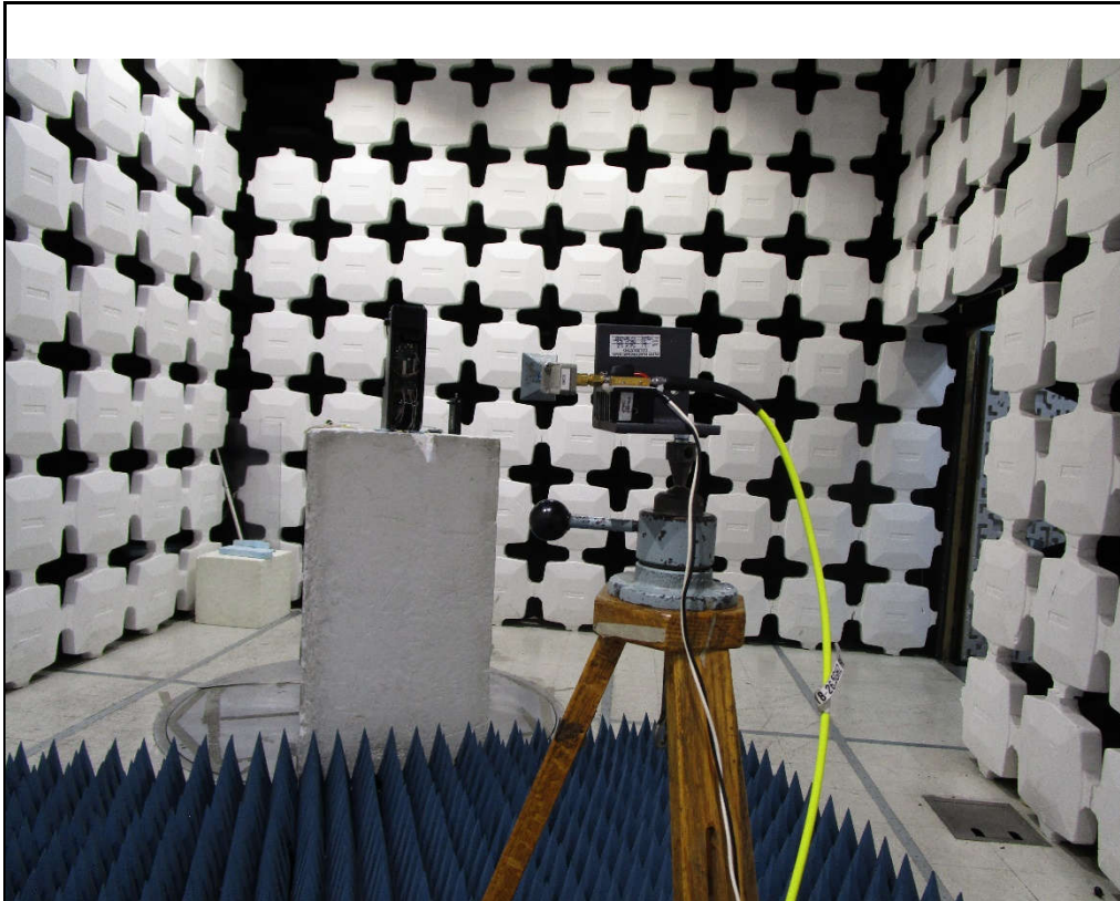
Test Setup for Spurious Radiated Emissions, Above 18GHz – Antenna Polarization Horizontal
