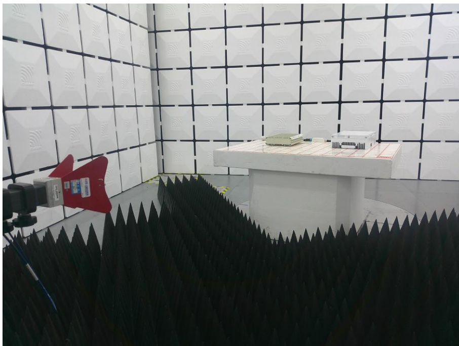
1GHz-3GHz
