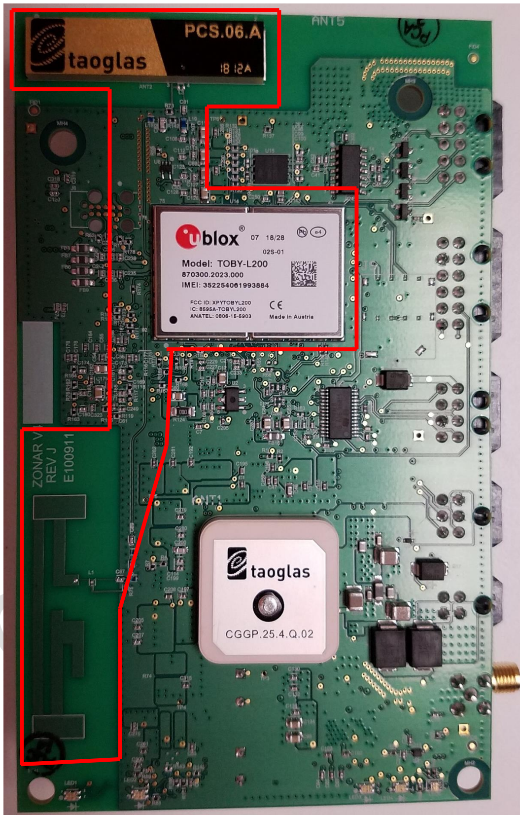
Figure 3 Cellular Radio Sub-Circuit
