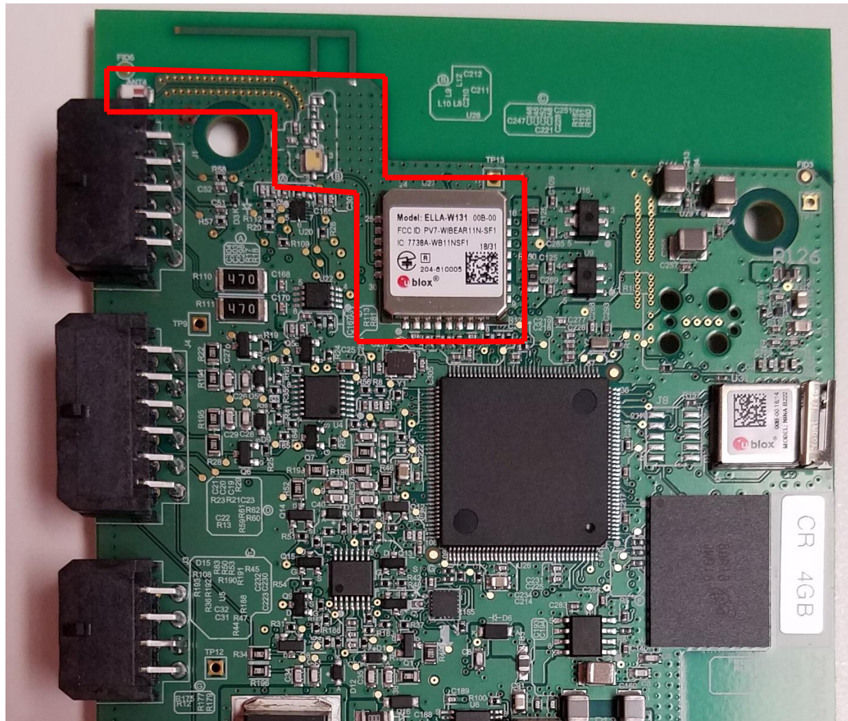
Figure 5 Wi-Fi radio Sub-Circuit (bottom side)
