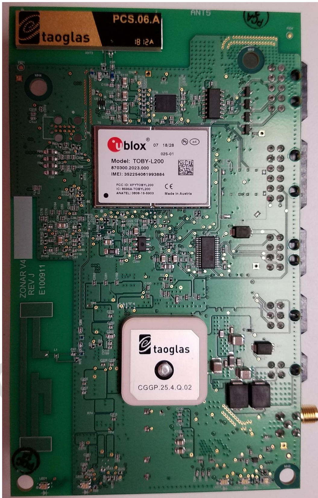
Figure 2 Antenna/Top Side
