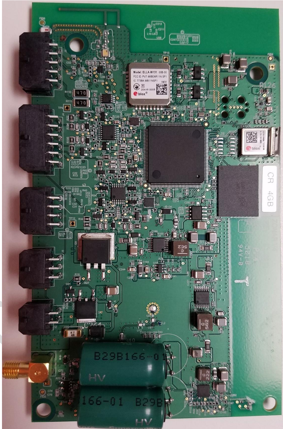
Figure 1 Component/Bottom Side
