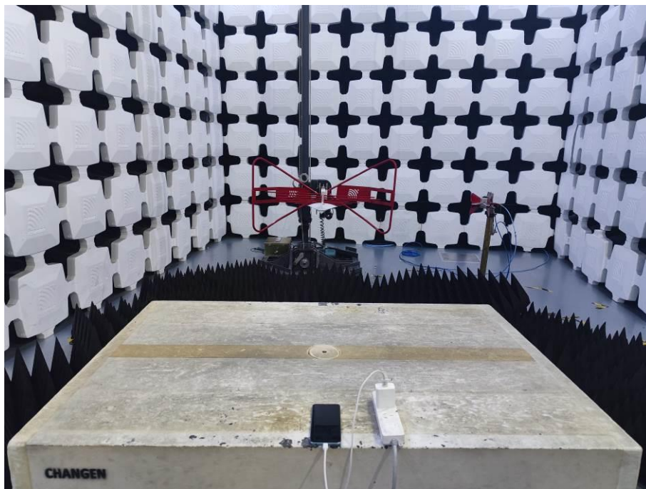
2. Radiated Emissions (Part 15B, Fiberglass Material Shell, Camera, 1GHz-18GHz)
