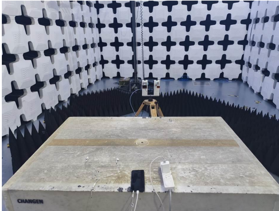
7. Radiated Emissions (Part 15B, FM receiver, 18GHz-26.5GHz)
