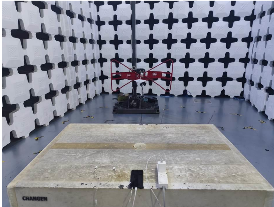
5. Radiated Emissions (Part 15B, FM receiver, 30MHz-1GHz)
