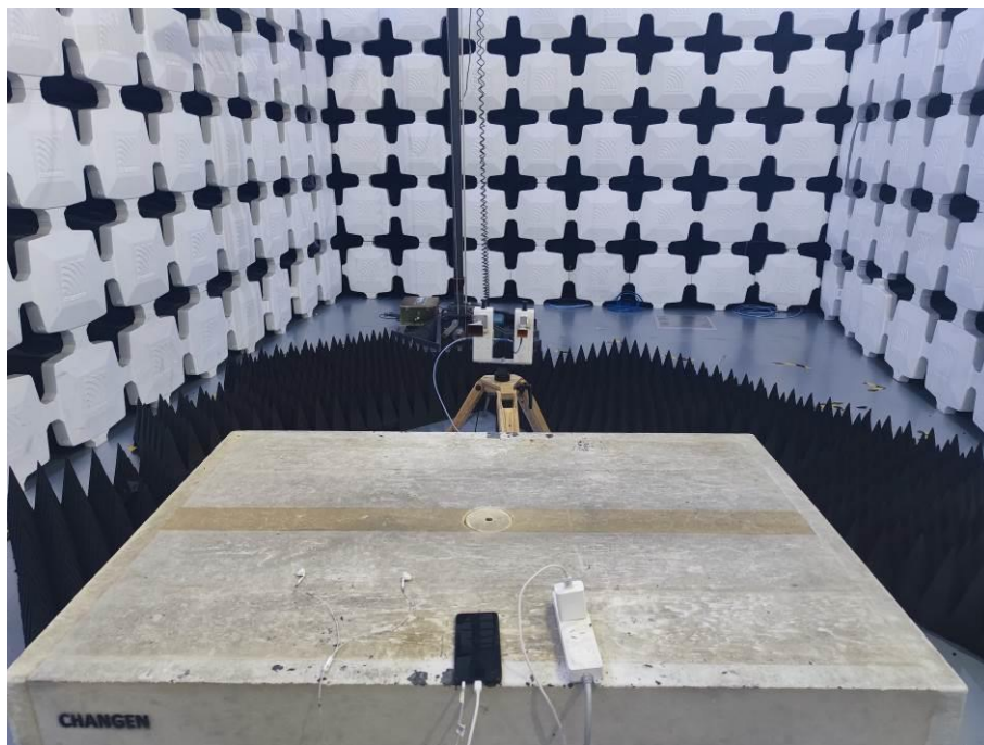
8. Radiated Emissions (Part 15B, FM receiver, 26.5GHz-40GHz)
