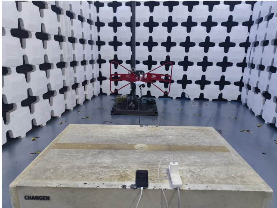
1. Radiated Emissions (Part 15B, Fiberglass Material Shell, Camera, 30MHz-1GHz)
