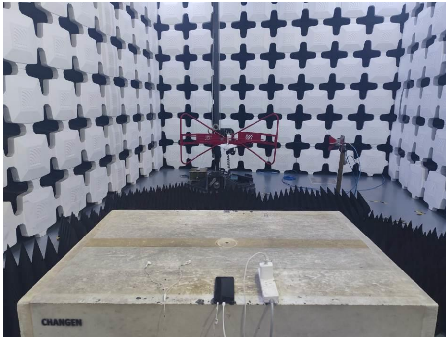
6. Radiated Emissions (Part 15B, FM receiver, 1GHz-18GHz)
