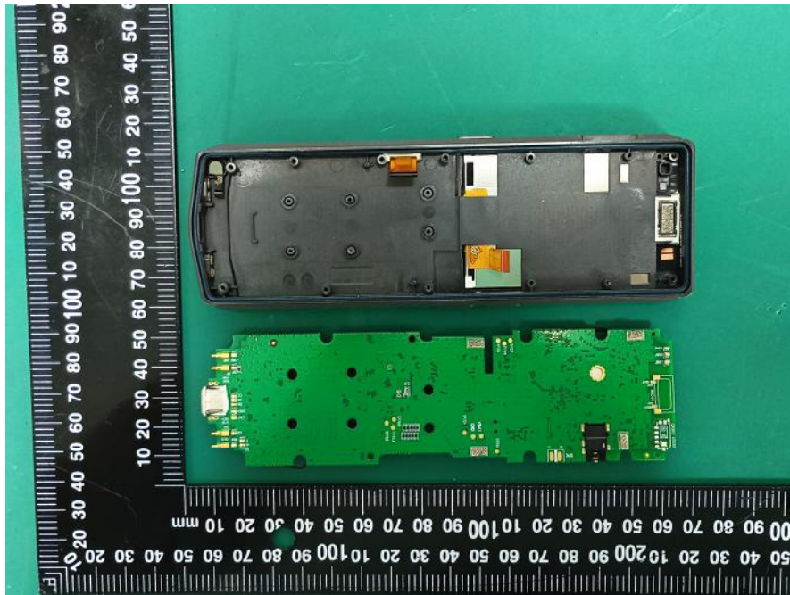
WIFI ANT 2
