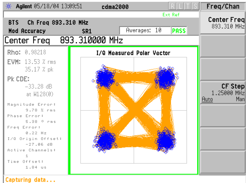
Channel 777 – 893.31 MHz
