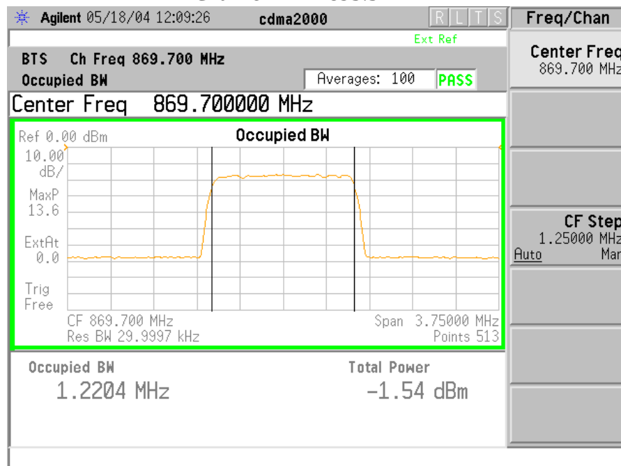
Channel 1020 – 869.7 MHz
