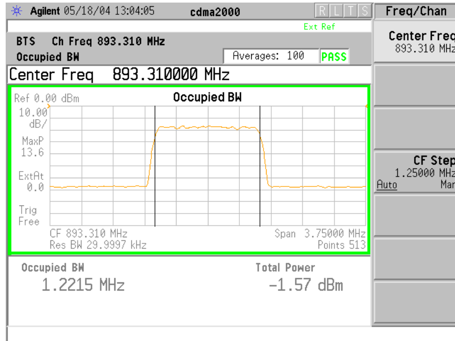
Channel 777 – 893.31 MHz
