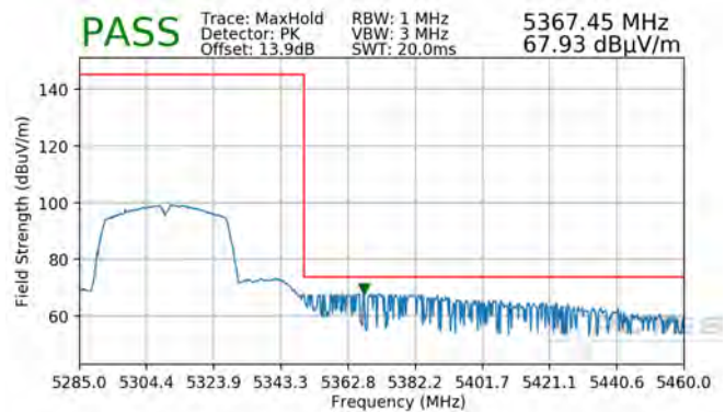
Plot 7-95. Radiated Upper Band Edge Plot (Peak – UNII Band 2A)
