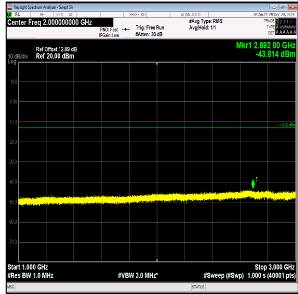
Band12_3MHz_16QAM_23165_1RB#0_1000~3000_1000~3000
