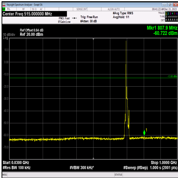
Band12_10MHz_QPSK_23095_1RB#0_30~1000_30~1000
