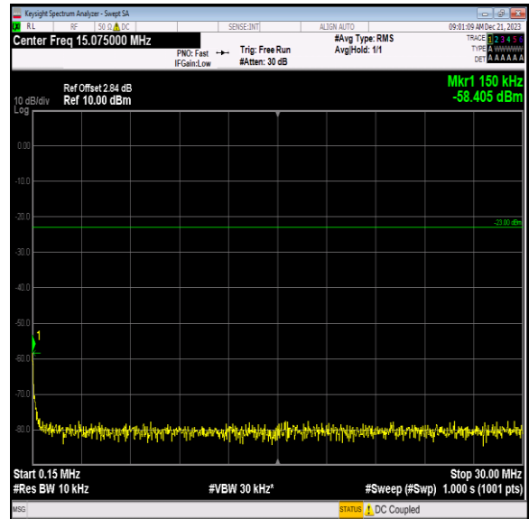
Band12_5MHz_QPSK_23035_1RB#0_0.15~30_0.15~30
