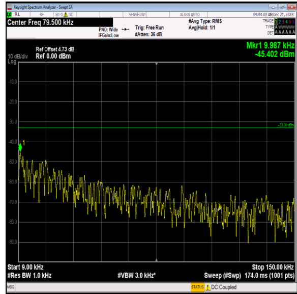
Band12_10MHz_QPSK_23130_1RB#0_0.009~0.15_0.009~0. 15
