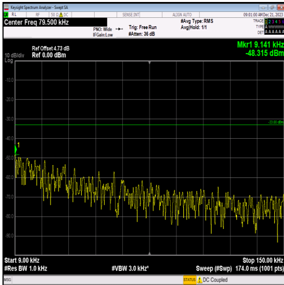
Band12_5MHz_QPSK_23035_1RB#0_0.009~0.15_0.009~0.1 5
