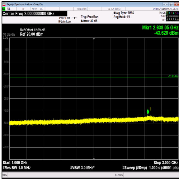
Band12_5MHz_64QAM_23095_1RB#0_1000~3000_1000~30 00
