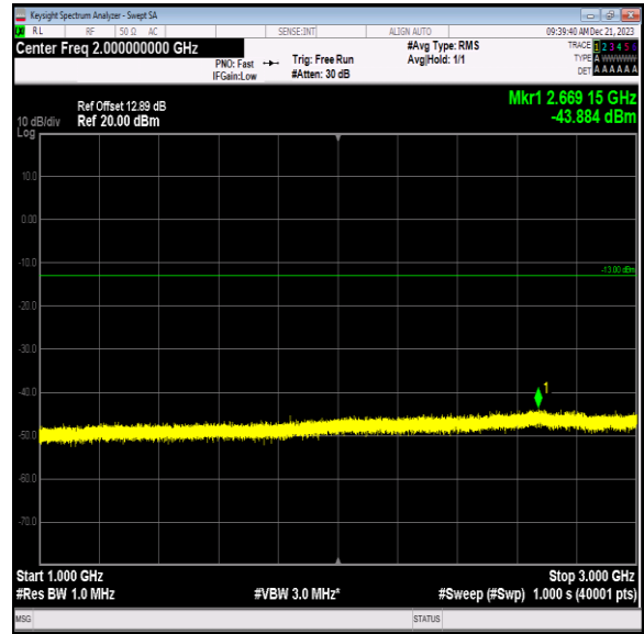
Band12_10MHz_16QAM_23060_1RB#0_1000~3000_1000~3000
