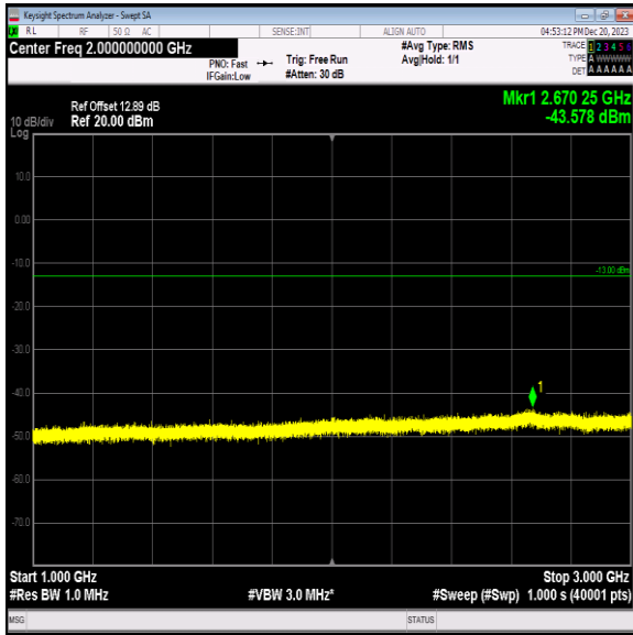
Band12_3MHz_16QAM_23095_1RB#0_1000~3000_1000~30 00
