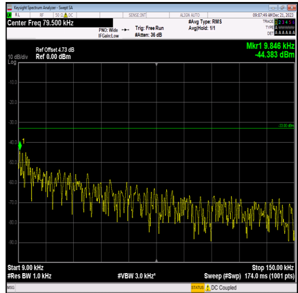
Band12_5MHz_16QAM_23155_1RB#0_0.009~0.15_0.009~0.15 15
