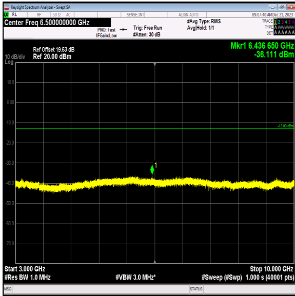
Band12_5MHz_QPSK_23155_1RB#0_3000~10000_3000~10000
