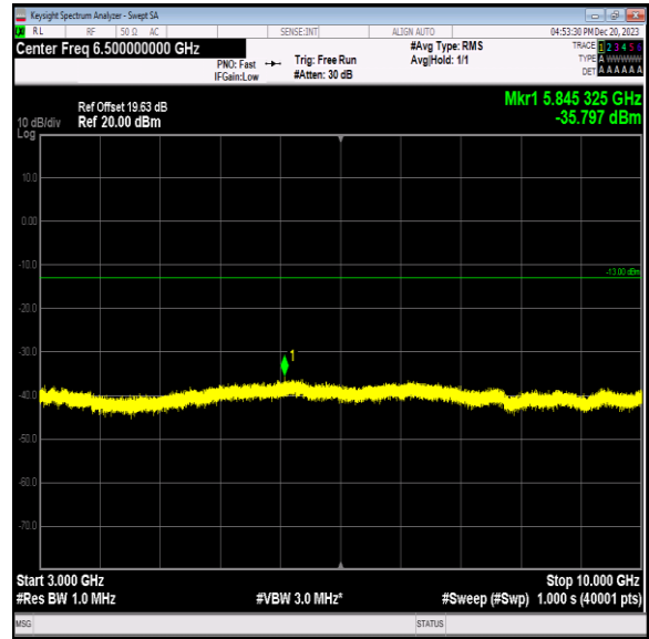
Band12_3MHz_16QAM_23095_1RB#0_3000~10000_3000~1 0000
