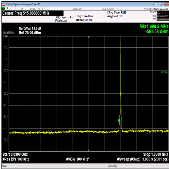
Band12_3MHz_64QAM_23095_1RB#0_30~1000_30~1000
