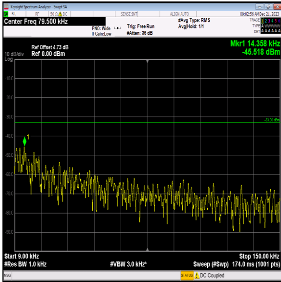
Band12_5MHz_64QAM_23035_1RB#0_0.009~0.15_0.009~0.15 15
