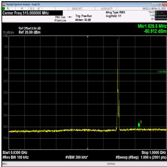
Band12_5MHz_64QAM_23035_1RB#0_30~1000_30~1000
