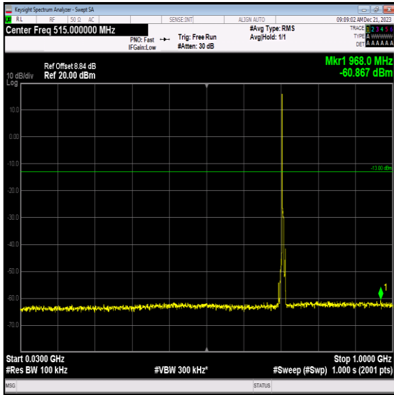
Band12_5MHz_64QAM_23155_1RB#0_30~1000_30~1000
