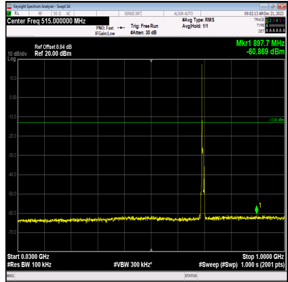
Band12_5MHz_16QAM_23035_1RB#0_30~1000_30~1000
