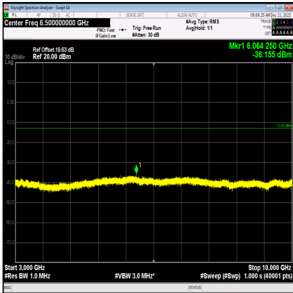
Band12_5MHz_64QAM_23155_1RB#0_3000~10000_3000~10000
