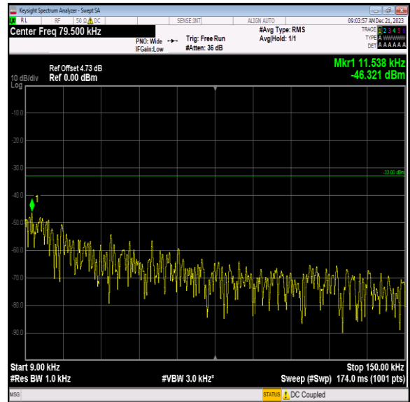
Band12_5MHz_QPSK_23095_1RB#0_0.009~0.15_0.009~0.15 5
