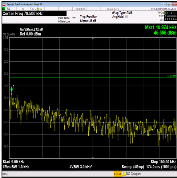
Band12_3MHz_64QAM_23095_1RB#0_0.009~0.15_0.009~0.15
