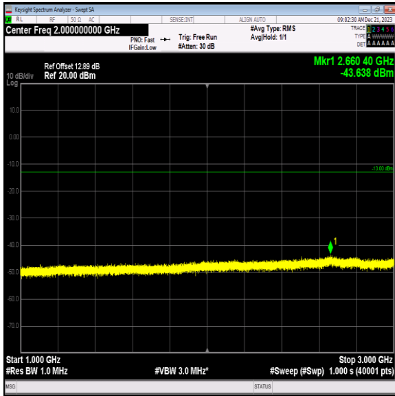
Band12_5MHz_16QAM_23035_1RB#0_1000~3000_1000~30 00
