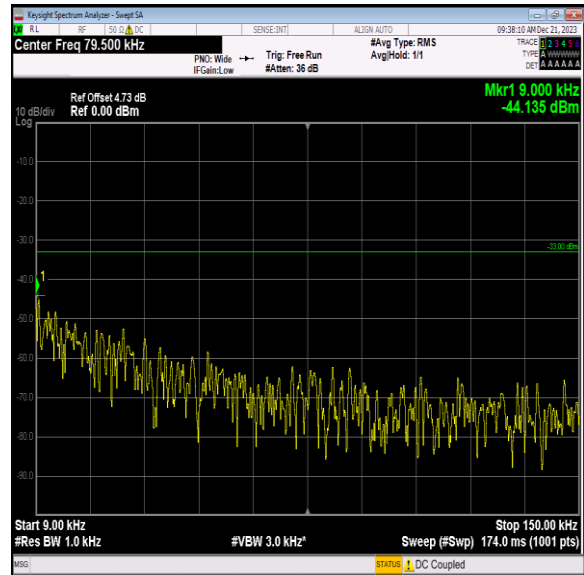
Band12_10MHz_QPSK_23060_1RB#0_0.009~0.15_0.009~0.15
