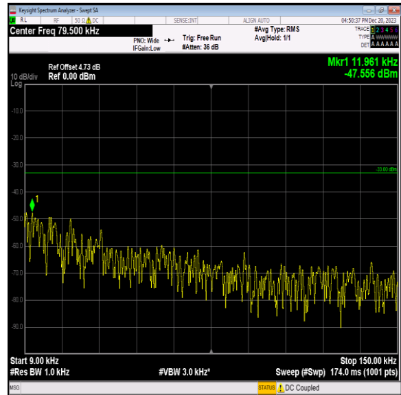
Band12_3MHz_64QAM_23025_1RB#0_0.009~0.15_0.009~0.15
