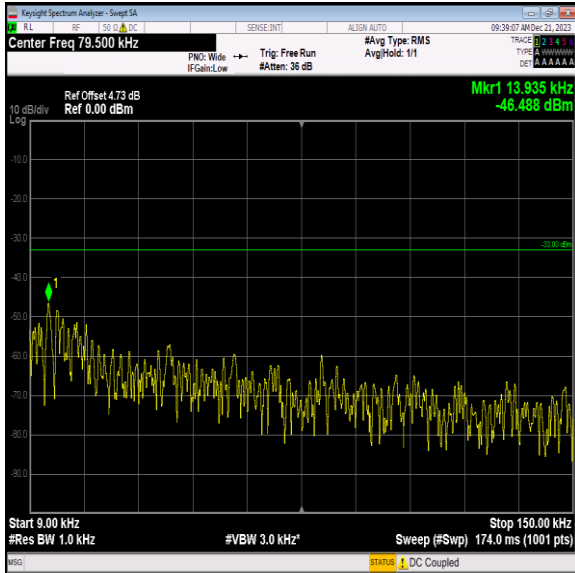
Band12_10MHz_16QAM_23060_1RB#0_0.009~0.15_0.009~ 0.15
