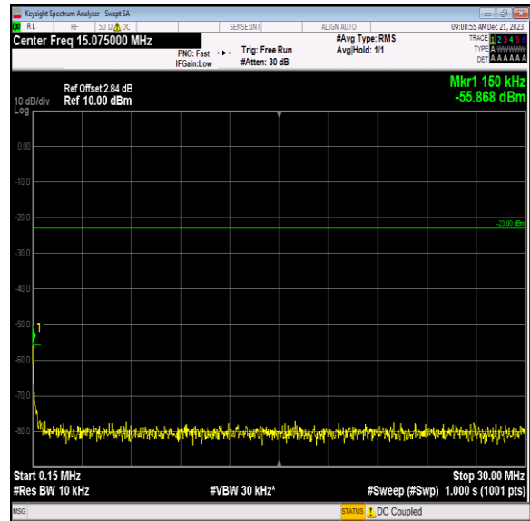
Band12_5MHz_64QAM_23155_1RB#0_0.15~30_0.15~30
