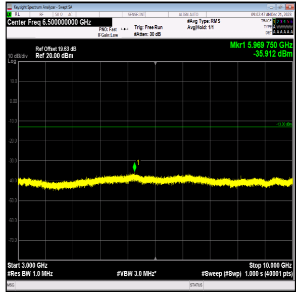
Band12_5MHz_16QAM_23035_1RB#0_3000~10000_3000~1 0000
