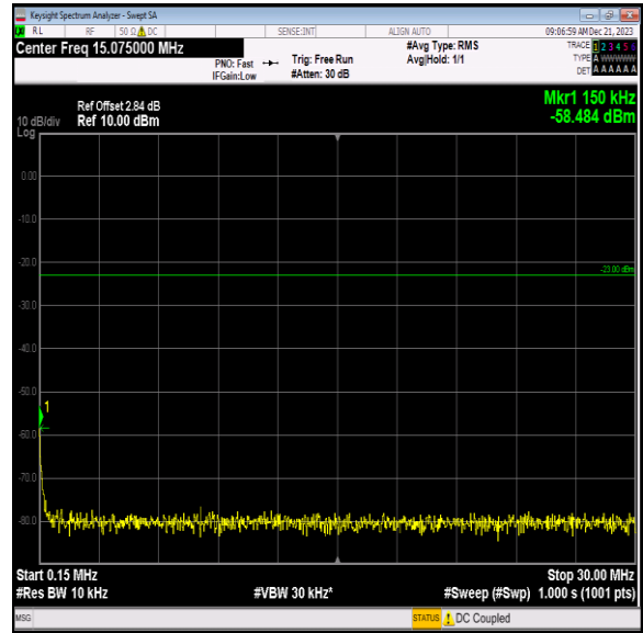
Band12_5MHz_QPSK_23155_1RB#0_0.15~30_0.15~30
