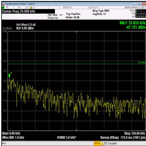
Band12_5MHz_16QAM_23095_1RB#0_0.009~0.15_0.009~0. 15
