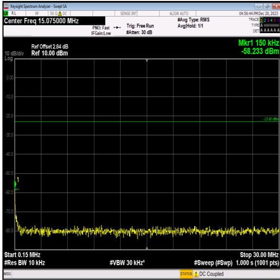
Band12_3MHz_64QAM_23165_1RB#0_0.15~30_0.15~30
