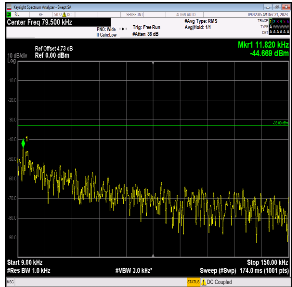
Band12_10MHz_16QAM_23095_1RB#0_0.009~0.15_0.009~0.15
