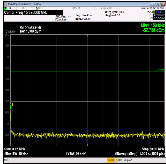
Band12_3MHz_16QAM_23025_1RB#0_0.15~30_0.15~30
