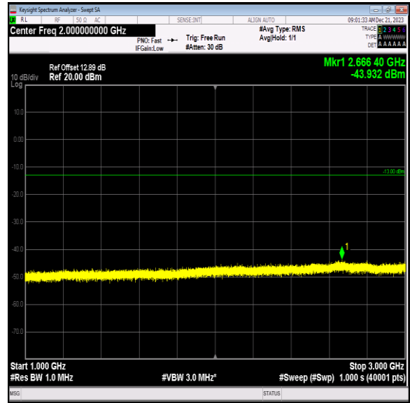
Band12_5MHz_QPSK_23035_1RB#0_1000~3000_1000~3000 0
