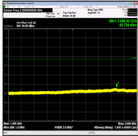
Band12_5MHz_64QAM_23155_1RB#0_1000~3000_1000~3000
