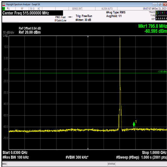
Band12_5MHz_QPSK_23155_1RB#0_30~1000_30~1000
