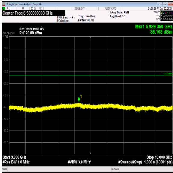
Band12_3MHz_16QAM_23025_1RB#0_3000~10000_3000~1 0000
