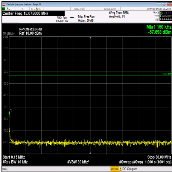
Band12_10MHz_QPSK_23130_1RB#0_0.15~30_0.15~30
