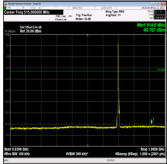
Band12_5MHz_64QAM_23095_1RB#0_30~1000_30~1000
