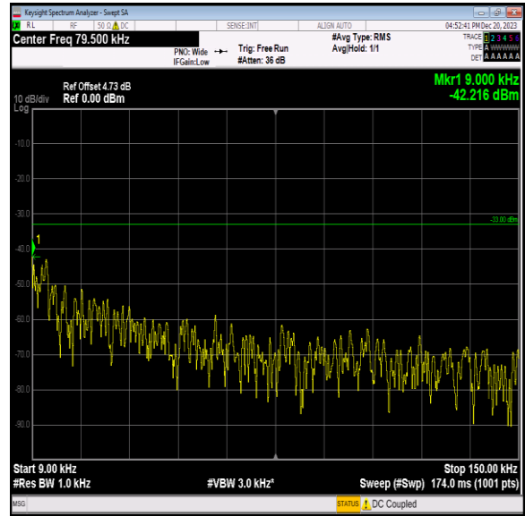
Band12_3MHz_16QAM_23095_1RB#0_0.009~0.15_0.009~0. 15
