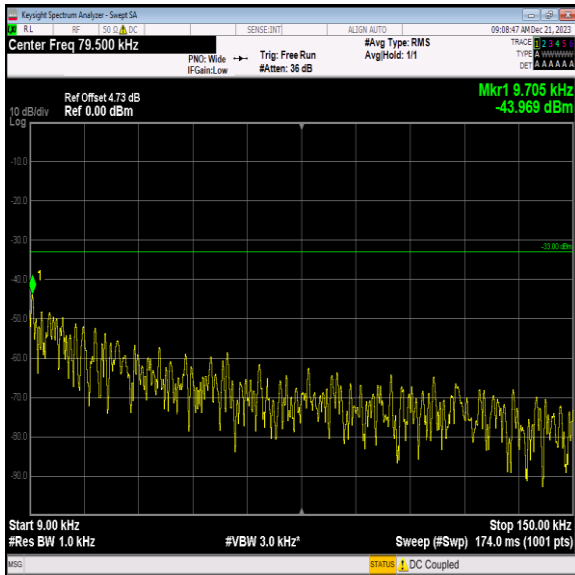
Band12_5MHz_64QAM_23155_1RB#0_0.009~0.15_0.009~0. 15
