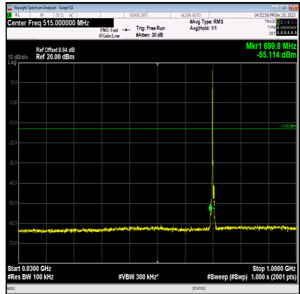
Band12_3MHz_16QAM_23095_1RB#0_30~1000_30~1000
