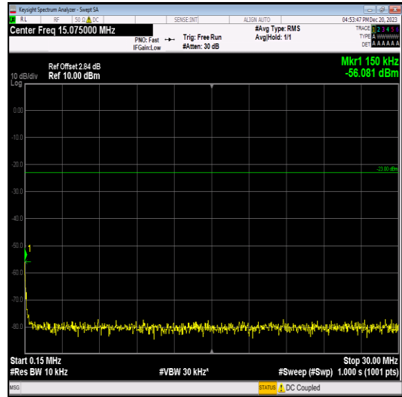
Band12_3MHz_64QAM_23095_1RB#0_0.15~30_0.15~30
