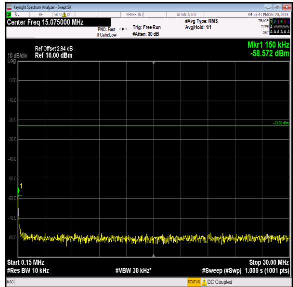
Band12_3MHz_16QAM_23165_1RB#0_0.15~30_0.15~30
