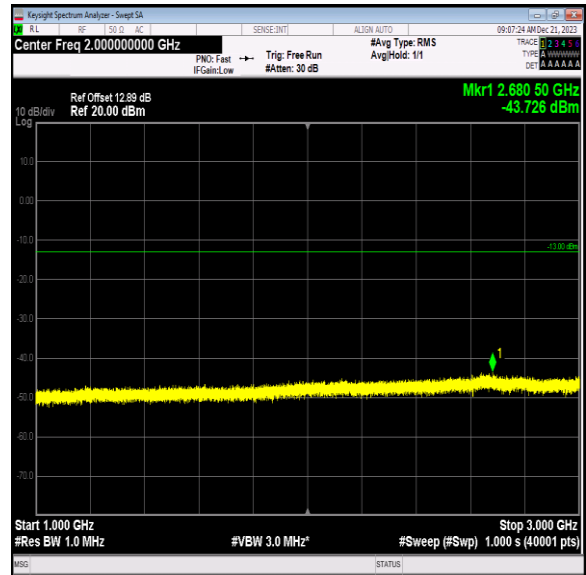
Band12_5MHz_QPSK_23155_1RB#0_1000~3000_1000~300 0
