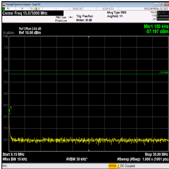
Band12_3MHz_16QAM_23095_1RB#0_0.15~30_0.15~30
