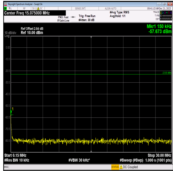
Band12_10MHz_QPSK_23095_1RB#0_0.15~30_0.15~30
