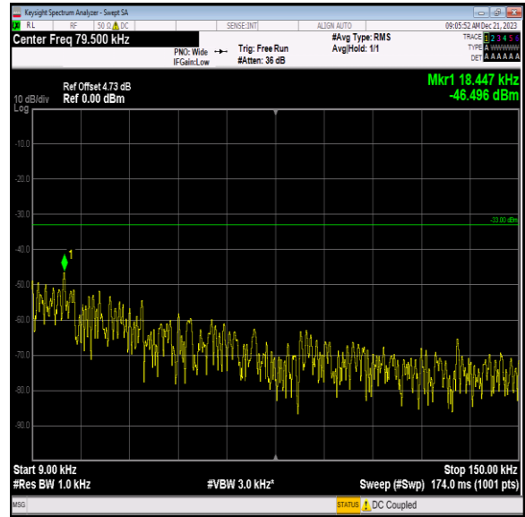
Band12_5MHz_64QAM_23095_1RB#0_0.009~0.15_0.009~0. 15
