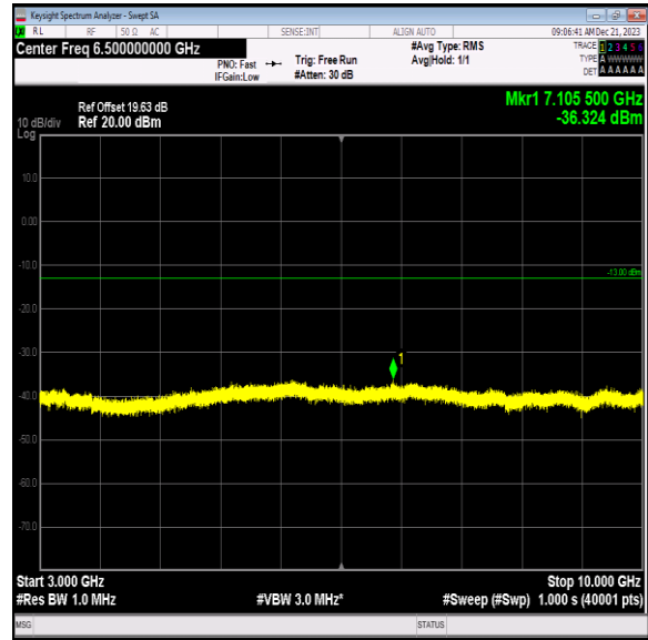
Band12_5MHz_64QAM_23095_1RB#0_3000~10000_3000~1 0000
