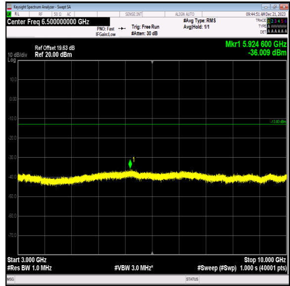
Band12_10MHz_QPSK_23130_1RB#0_3000~10000_3000~1 0000
