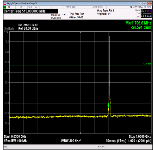
Band12_3MHz_64QAM_23165_1RB#0_30~1000_30~1000
