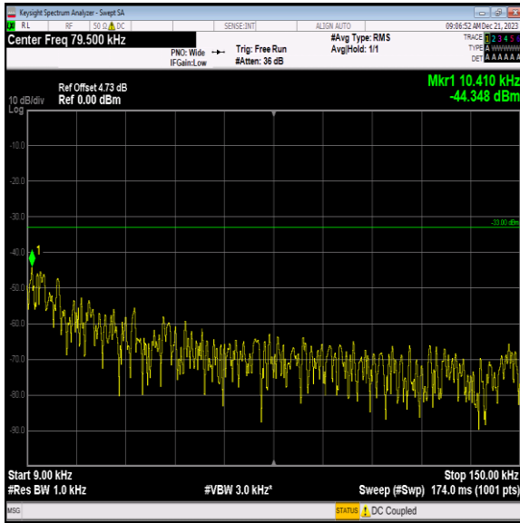
Band12_5MHz_QPSK_23155_1RB#0_0.009~0.15_0.009~0.1 5
