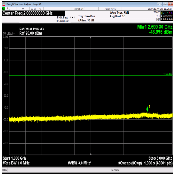
Band12_10MHz_QPSK_23130_1RB#0_1000~3000_1000~30 00
