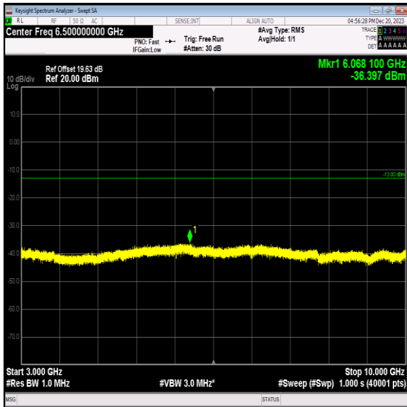
Band12_3MHz_16QAM_23165_1RB#0_3000~10000_3000~10000
