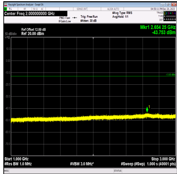
Band12_3MHz_16QAM_23025_1RB#0_1000~3000_1000~3000 00
