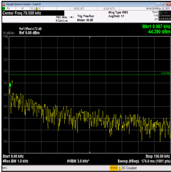
Band12_3MHz_16QAM_23025_1RB#0_0.009~0.15_0.009~0.15 15
