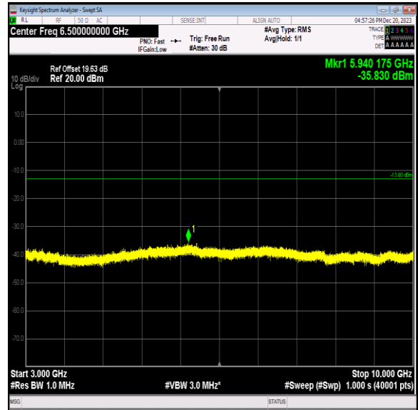
Band12_3MHz_64QAM_23165_1RB#0_3000~10000_3000~1 0000
