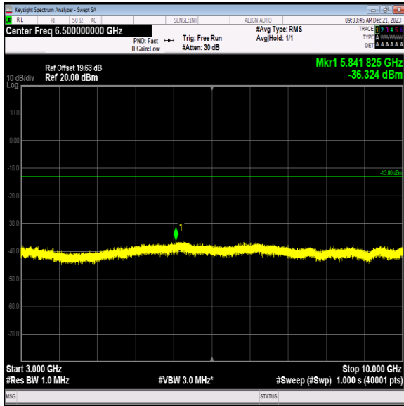
Band12_5MHz_64QAM_23035_1RB#0_3000~10000_3000~1 0000
