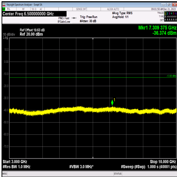
Band12_5MHz_QPSK_23035_1RB#0_3000~10000_3000~10000 000
