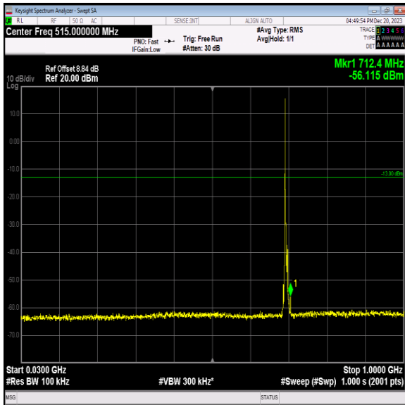
Band12_3MHz_16QAM_23025_1RB#0_30~1000_30~1000
