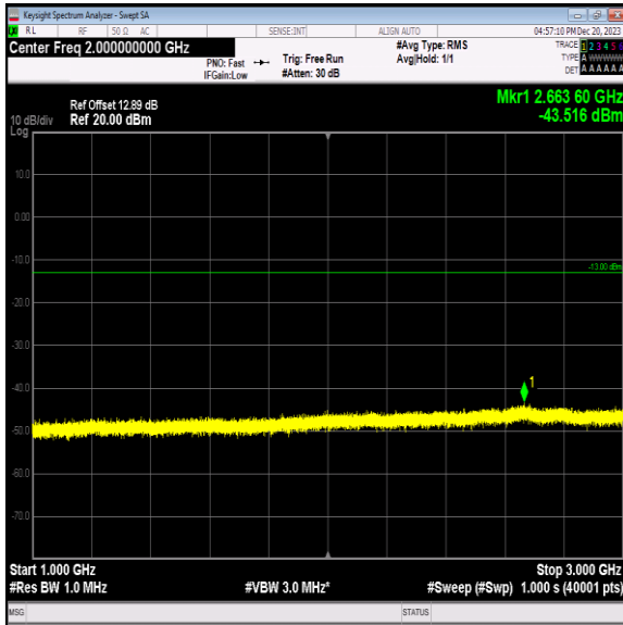
Band12_3MHz_64QAM_23165_1RB#0_1000~3000_1000~30 00
