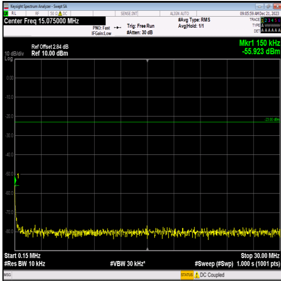
Band12_5MHz_64QAM_23095_1RB#0_0.15~30_0.15~30
