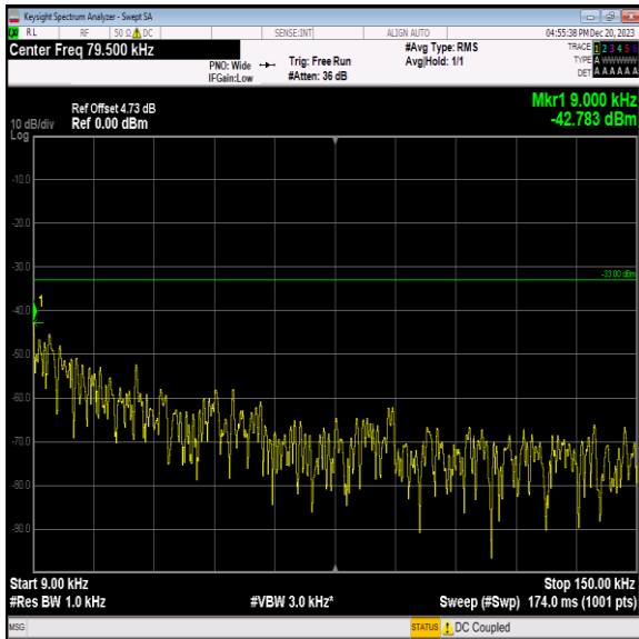
Band12_3MHz_16QAM_23165_1RB#0_0.009~0.15_0.009~0. 15
