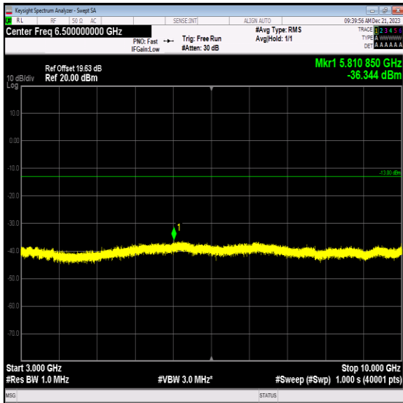
Band12_10MHz_16QAM_23060_1RB#0_3000~10000_3000~10000
