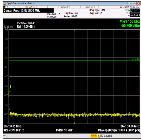
Band12_5MHz_64QAM_23035_1RB#0_0.15~30_0.15~30
