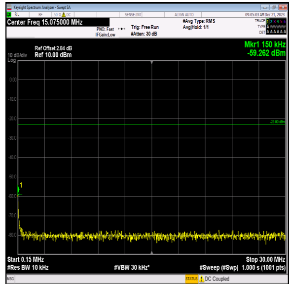
Band12_5MHz_16QAM_23095_1RB#0_0.15~30_0.15~30
