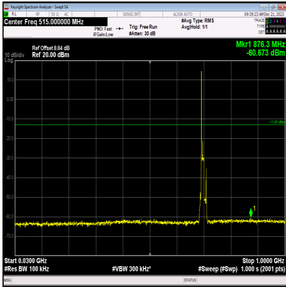
Band12_10MHz_16QAM_23060_1RB#0_30~1000_30~1000
