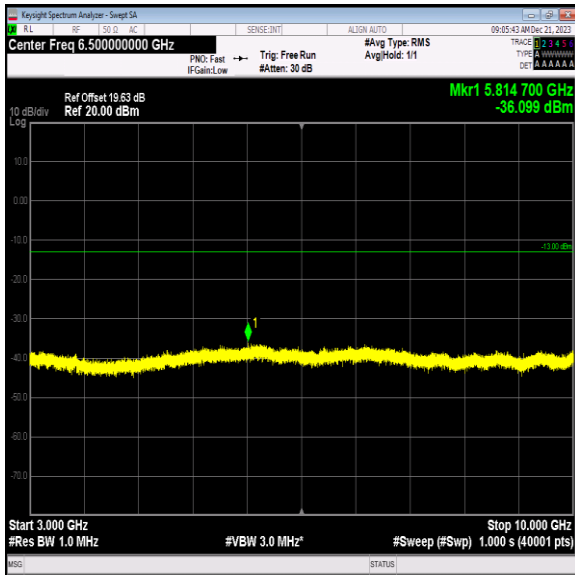
Band12_5MHz_16QAM_23095_1RB#0_3000~10000_3000~10000 0000
