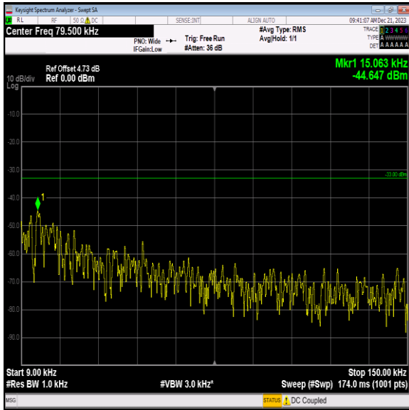
Band12_10MHz_QPSK_23095_1RB#0_0.009~0.15_0.009~0.15
