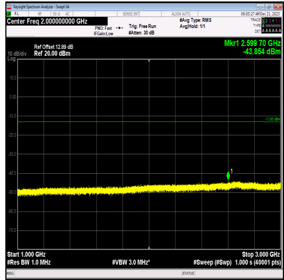
Band12_5MHz_16QAM_23095_1RB#0_1000~3000_1000~3000 00
