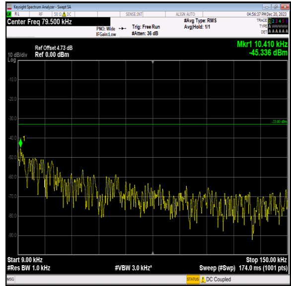
Band12_3MHz_64QAM_23165_1RB#0_0.009~0.15_0.009~0. 15
