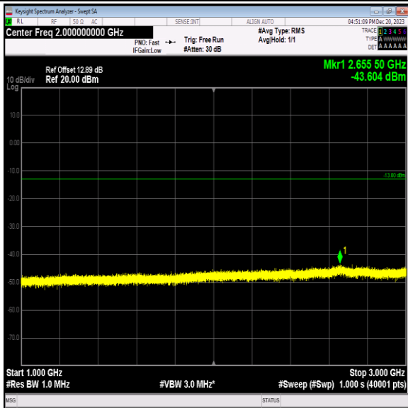
Band12_3MHz_64QAM_23025_1RB#0_1000~3000_1000~30
