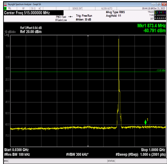
Band12_10MHz_QPSK_23130_1RB#0_30~1000_30~1000
