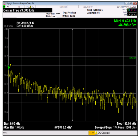
Band12_5MHz_16QAM_23035_1RB#0_0.009~0.15_0.009~0.15
