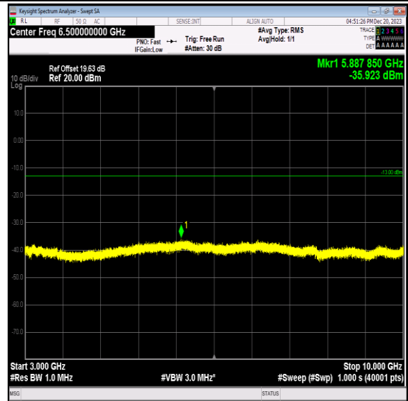
Band12_3MHz_64QAM_23025_1RB#0_3000~10000_3000~1
