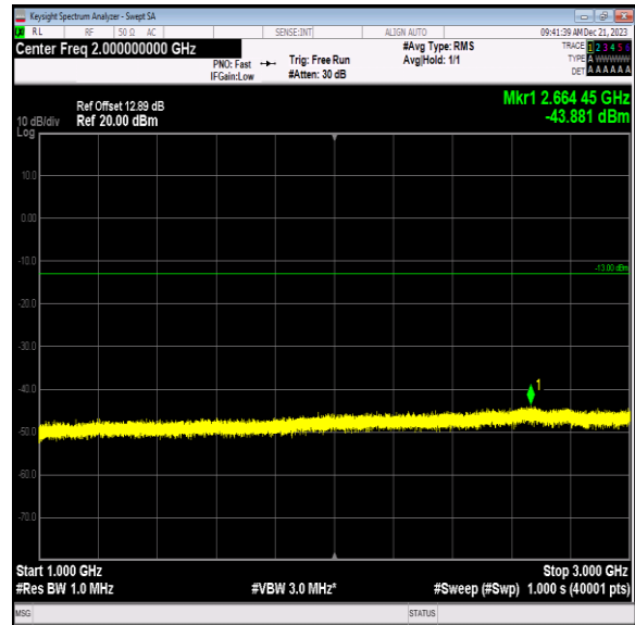
Band12_10MHz_QPSK_23095_1RB#0_1000~3000_1000~3000
