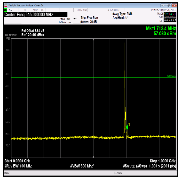
Band12_3MHz_64QAM_23025_1RB#0_30~1000_30~1000
