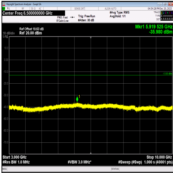
Band12_3MHz_64QAM_23095_1RB#0_3000~10000_3000~1 0000
