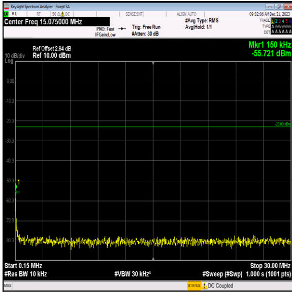
Band12_5MHz_16QAM_23035_1RB#0_0.15~30_0.15~30
