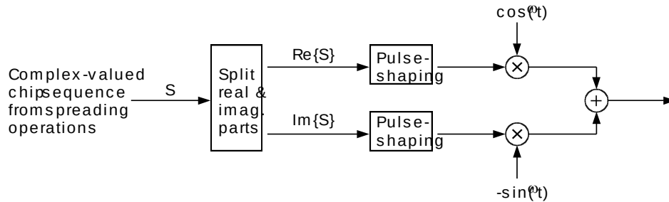
Figure 3-3: Uplink modulation
