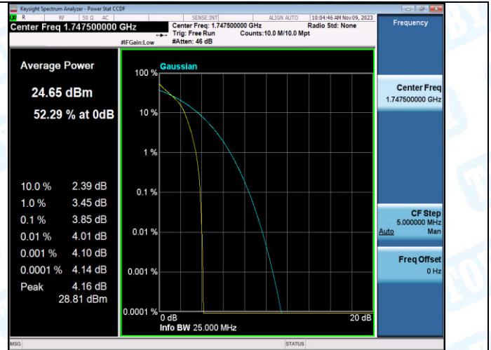
Band4-15MHz-QPSK-20325-1RB#0-PASS
