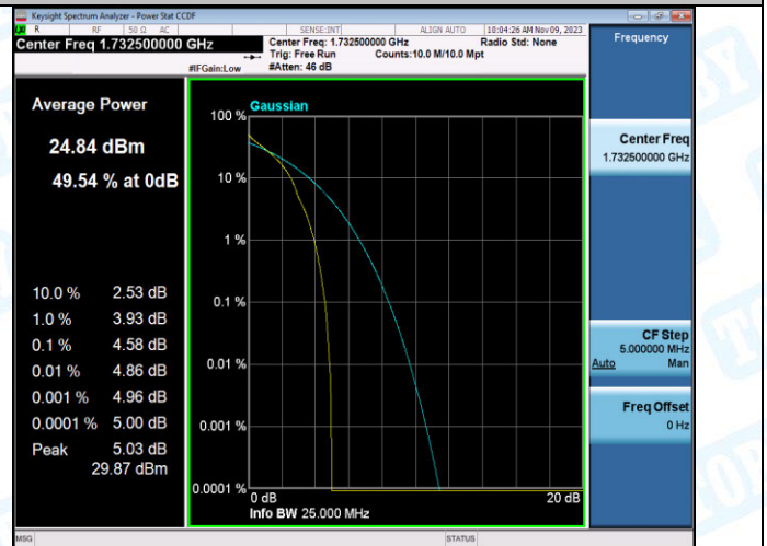
Band4-15MHz-QPSK-20175-1RB#0-PASS
