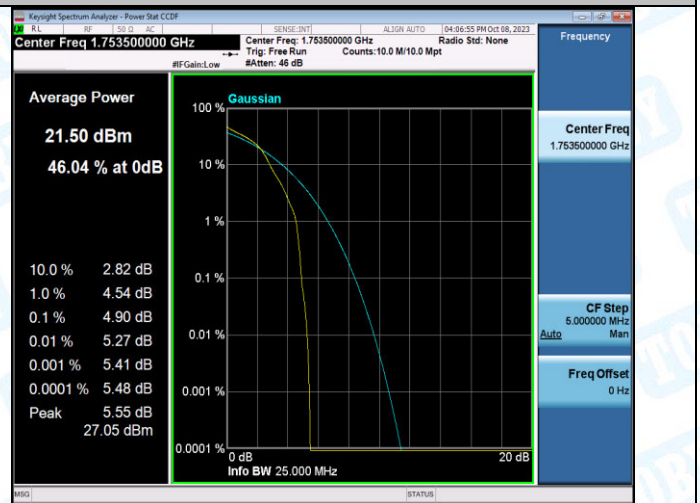
Band4-3MHz-16QAM-20385-1RB#0-PASS
