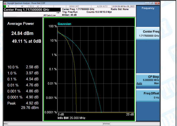
Band4-15MHz-QPSK-20025-1RB#0-PASS
