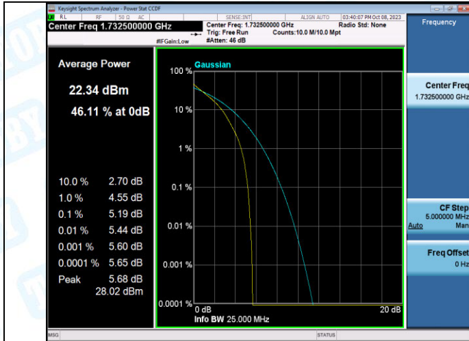
Band4-1.4MHz-QPSK-20175-6RB#0-PASS
