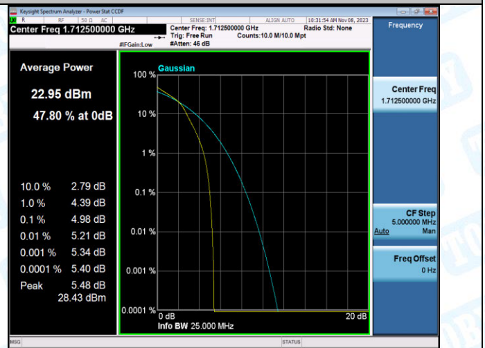
Band4-5MHz-16QAM-19975-25RB#0-PASS
