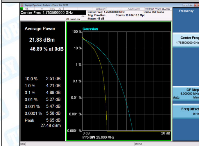
Band4-3MHz-QPSK-20385-15RB#0-PASS
