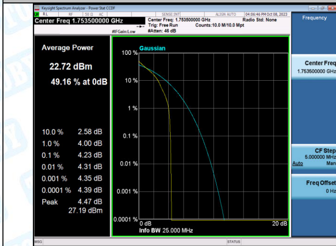
Band4-3MHz-QPSK-20385-1RB#0-PASS
