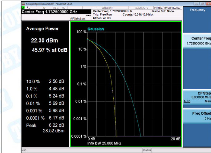
Band4-3MHz-QPSK-20175-15RB#0-PASS
