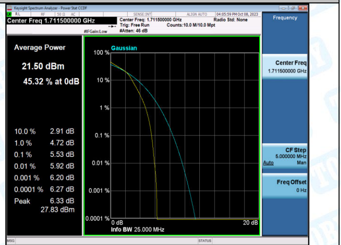
Band4-3MHz-16QAM-19965-15RB#0-PASS
