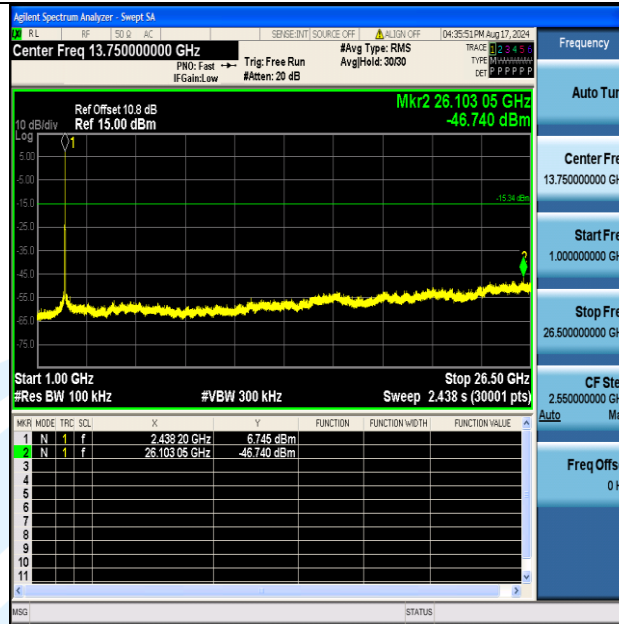
11G-Ant2-2437-1000~PASS
