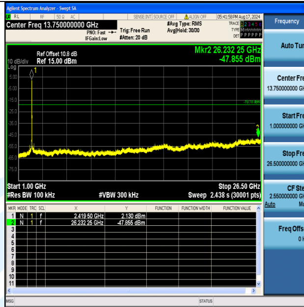
11N40MIMO-Ant2-2422-1000-26500-PASS
