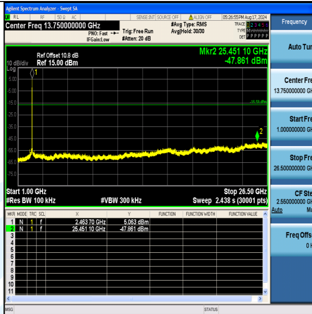
11N20MIMO-Ant2-2462-1000-26500-PASS
