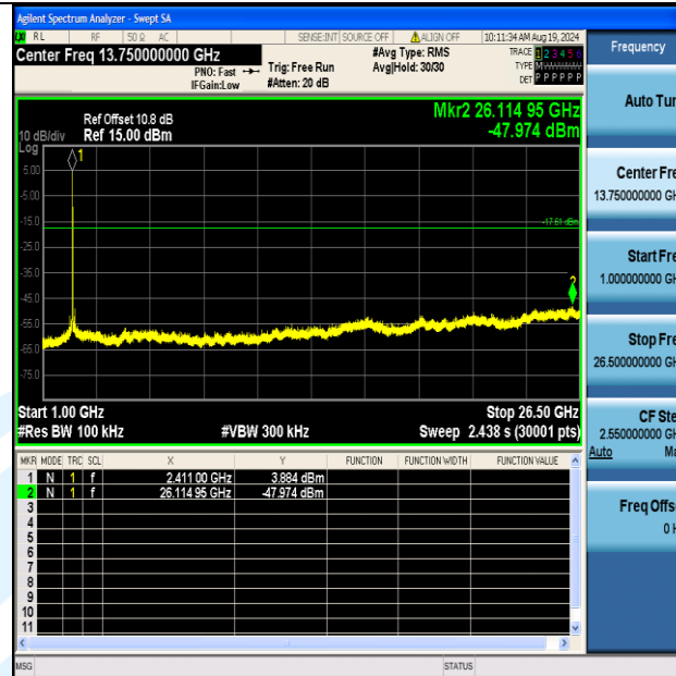
11AX20MIMO-Ant2-2412-1000~26500-PASS
