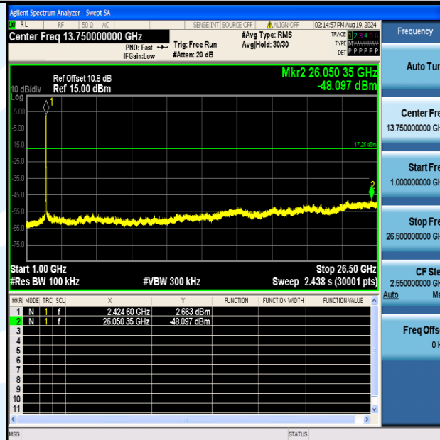
11N40MIMO-Ant1-2437-0-Reference-PASS
