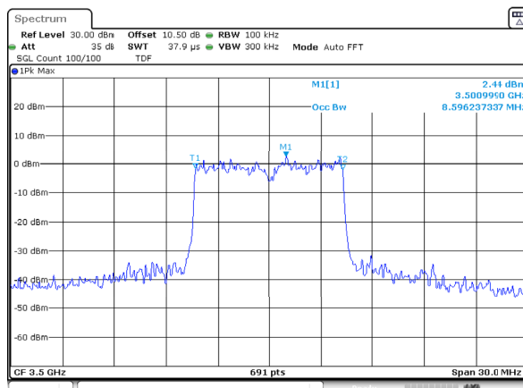
n78_1_10MHz_30kHz_3500MHz_CP-OFDM 64 QAM_RB24@0 Occupied Bandwidth
