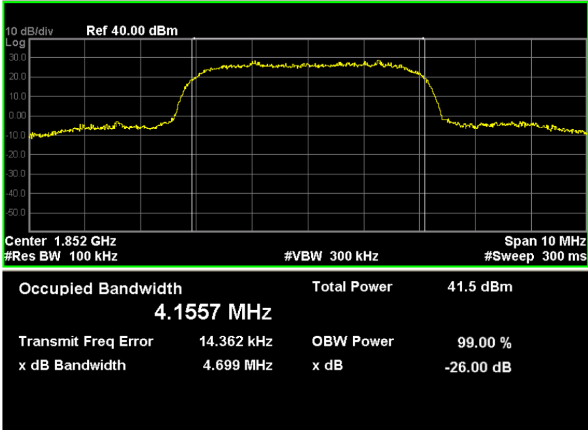
HSDPA Band II, Channel 9262
