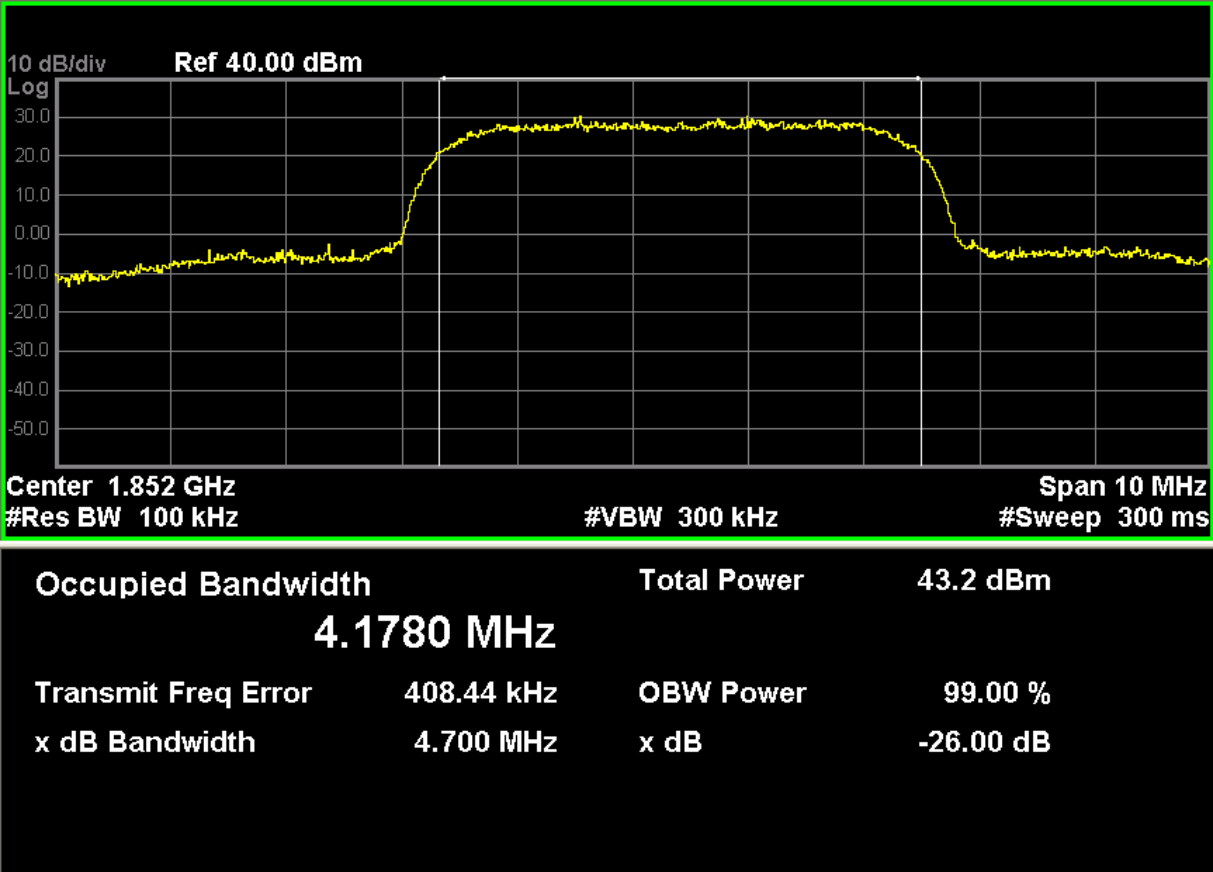
WCDMA Band II, Channel 9262
