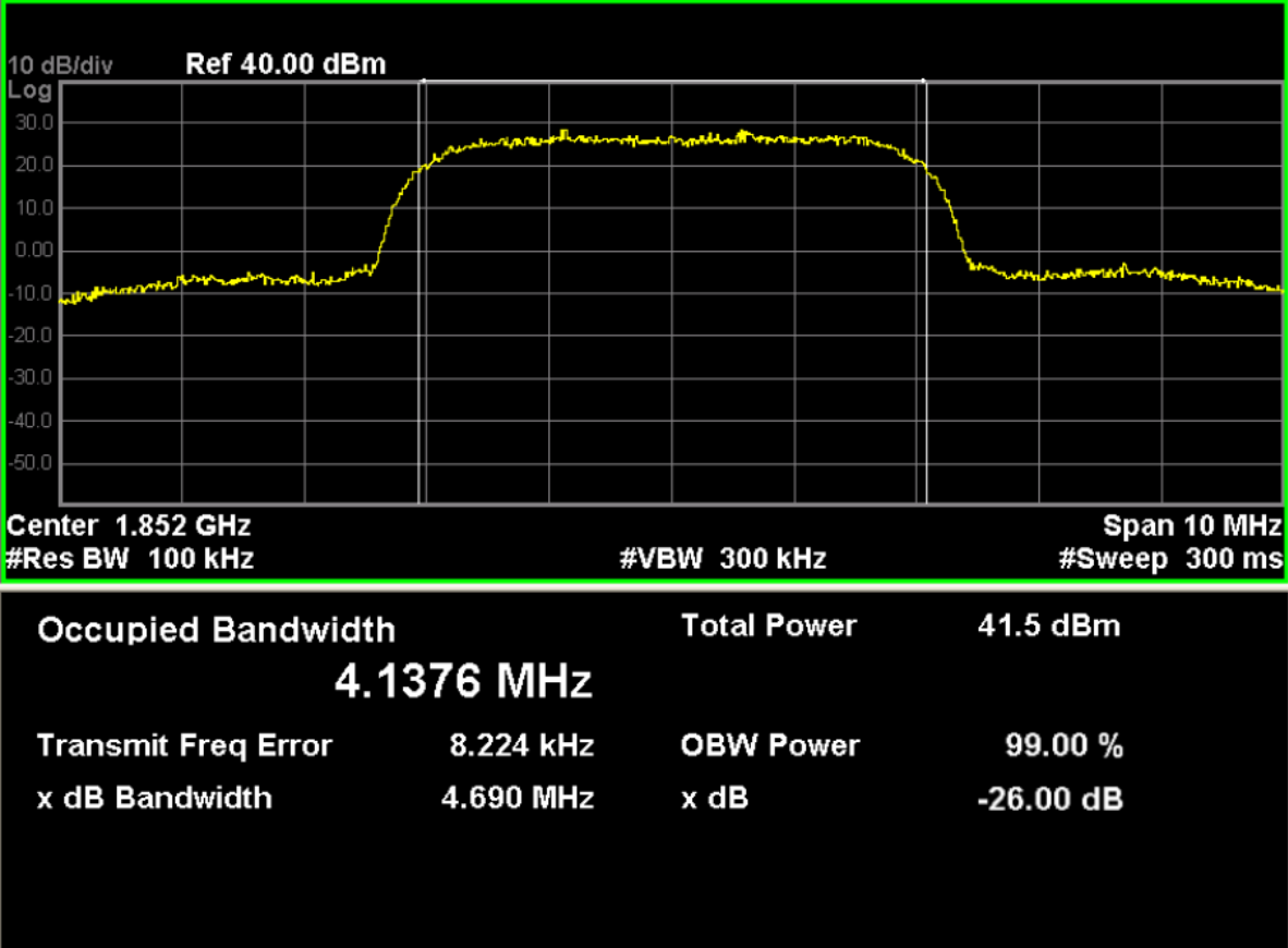
HSUPA Band II, Channel 9262
