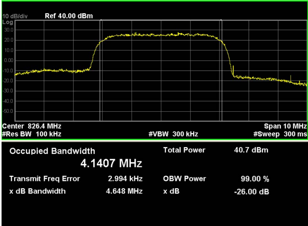
HSUPA Band V, Channel 4132
