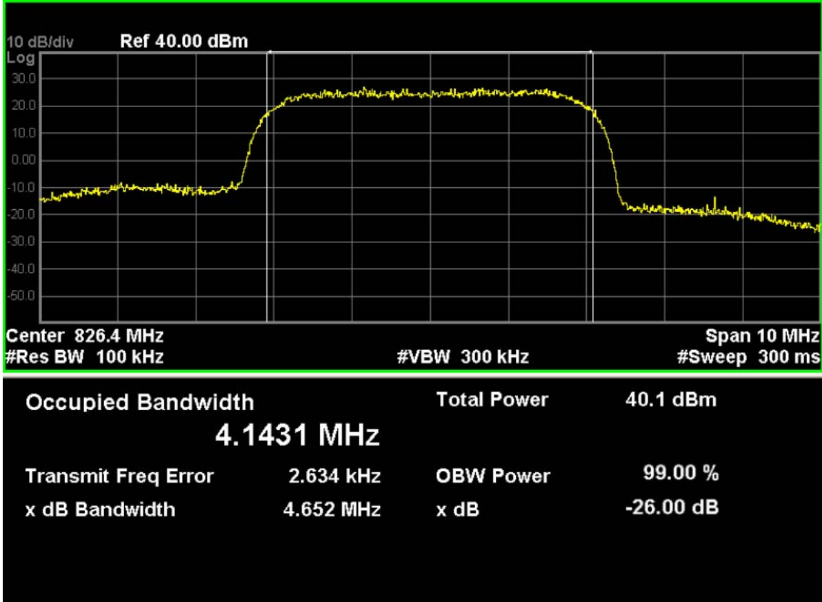
HSDPA Band V, Channel 4132
