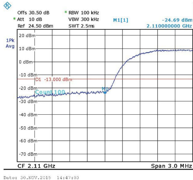
Figure 106. — WCDMA 2112.5 MHz
