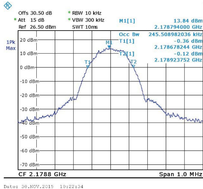
Figure 83. — GSM (2178.8 MHz) OUT
