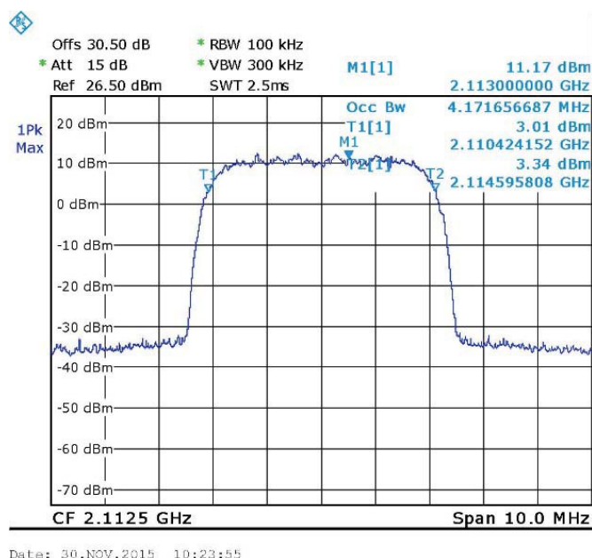
Figure 85. — WCDMA (2112.5 MHz) OUT
