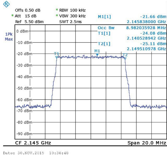
Figure 74. — LTE 64QAM (2145.0 MHz) IN
