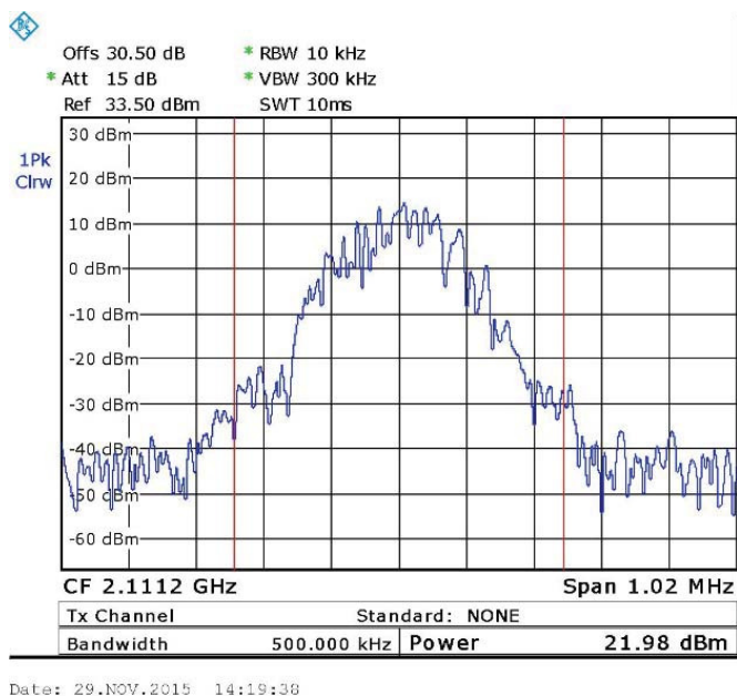
Figure 64. — GSM (2111.2 MHz)
