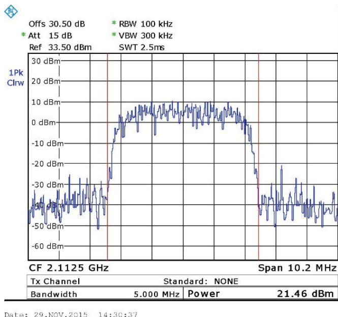
Figure 67. — WCDMA (2112.5 MHz)
