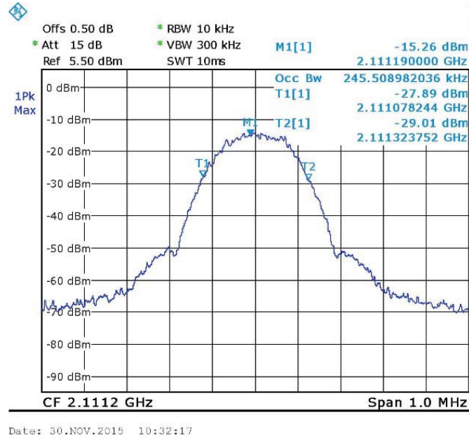
Figure 78. — GSM (2111.2 MHz) IN
