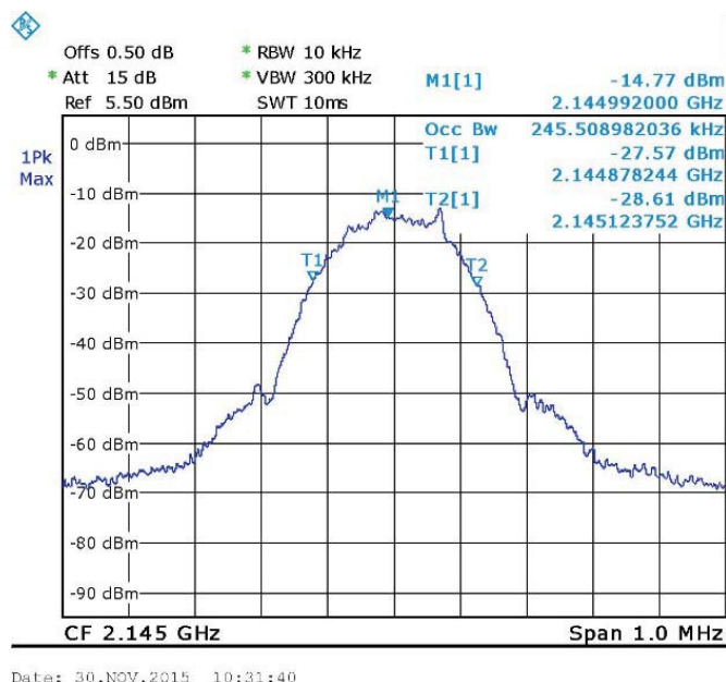
Figure 80. — GSM (2145.0 MHz) IN
