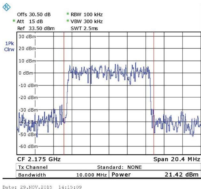
Figure 63. — LTE 64QAM (2175.0 MHz)
