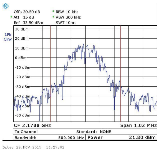
Figure 66. — GSM (2178.8 MHz)
