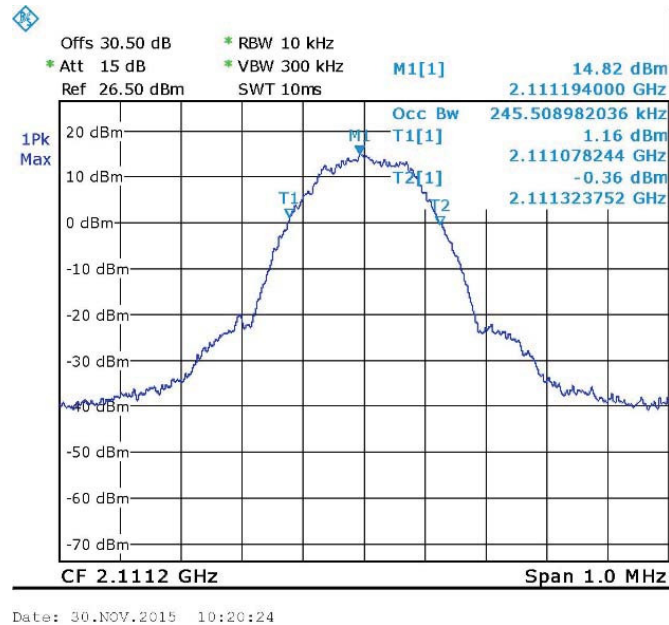
Figure 79. — GSM (2111.2 MHz) OUT
