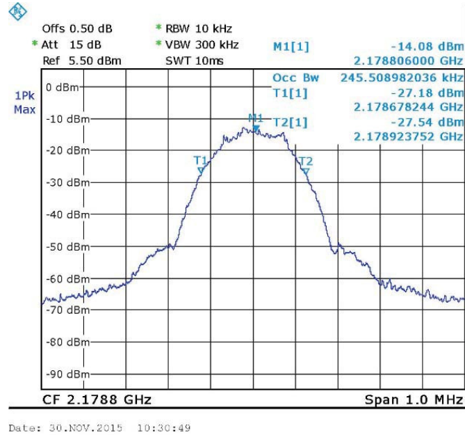
Figure 82. — GSM (2178.8 MHz) IN
