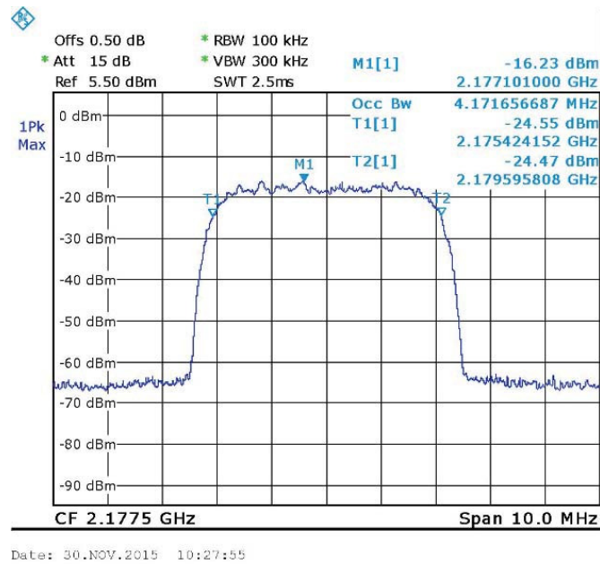
Figure 88. — WCDMA (2177.5 MHz) IN
