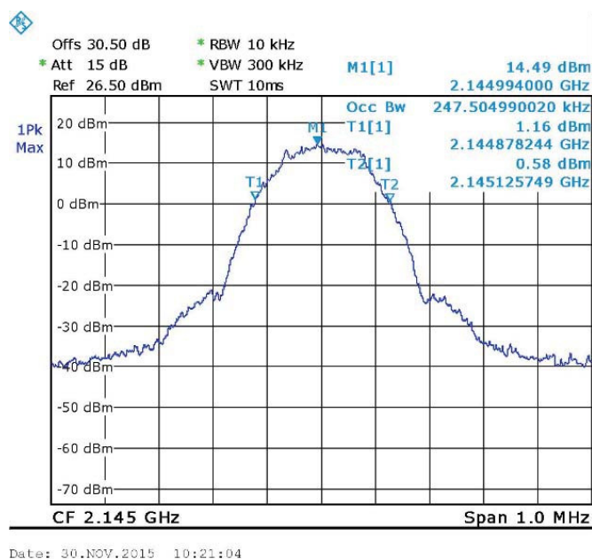
Figure 81. — GSM (2145.0 MHz) OUT
