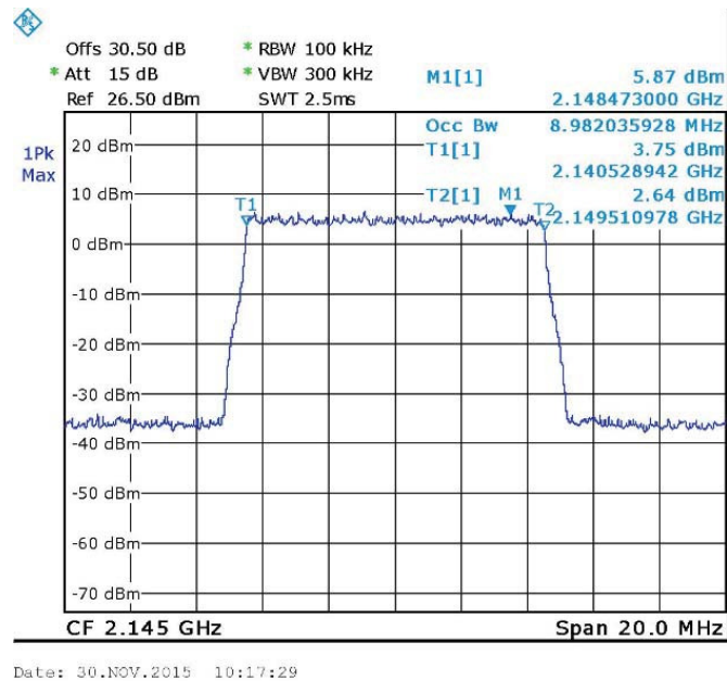
Figure 75. — LTE 64QAM (2145.0 MHz) OUT
