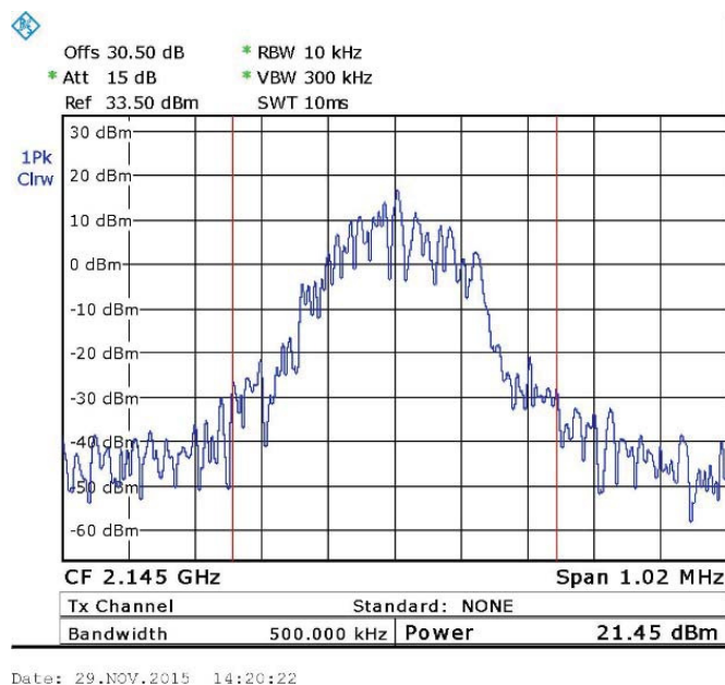
Figure 65. — GSM (2145.0 MHz)
