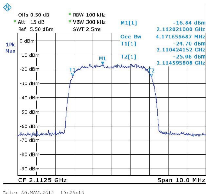
Figure 84. — WCDMA (2112.5 MHz) IN
