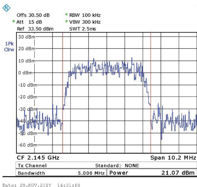
Figure 68. — WCDMA (2145.0 MHz)
