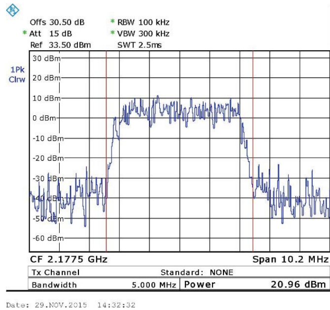
Figure 69. — WCDMA (2177.5 MHz)
