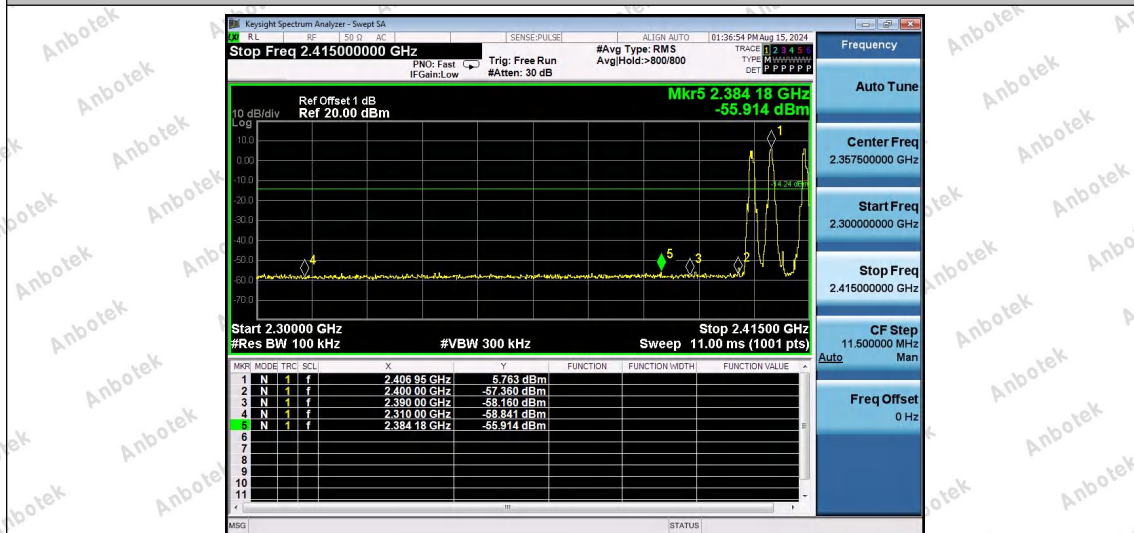
2.4G-Ant1-Hop_2403-PASS
