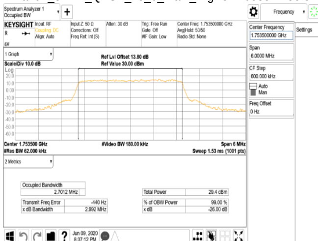
Band4_3MHz_QPSK_15_0_Main_HighCH20385-1753.5
