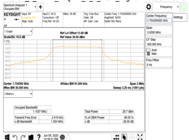
Band4_1_4MHz_16QAM_6_0_Main_HighCH20393-1754.3
