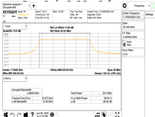
Band4_10MHz_16QAM_50_0_Main_HighCH20350-1750
