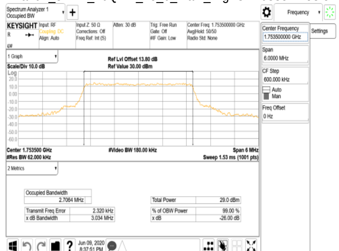
Band4_3MHz_16QAM_15_0_Main_HighCH20385-1753.5
