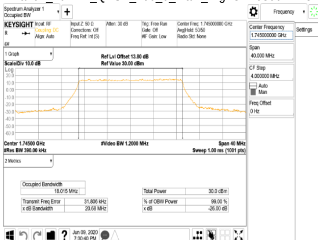
Band4_20MHz_QPSK_100_0_Main_HighCH20300-1745
