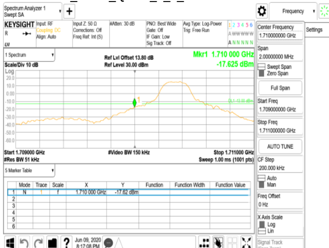
Band4_5MHz_QPSK_1_0_LowCH19975-1712.5
