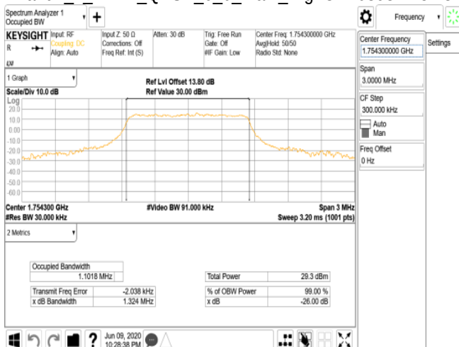
Band4_1_4MHz_QPSK_6_0_Main_HighCH20393-1754.3
