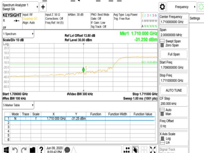
Band4_10MHz_QPSK_50_0_LowCH20000-1715
