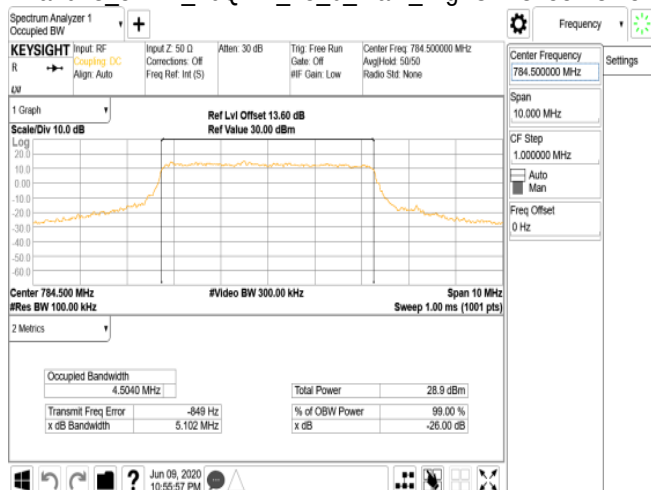
Band13_5MHz_16QAM_25_0_Main_HighCH23255-784.5
