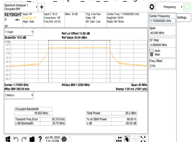
Band4_20MHz_16QAM_100_0_Main_HighCH20300-1745
