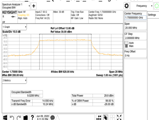
Band4_10MHz_QPSK_50_0_Main_HighCH20350-1750
