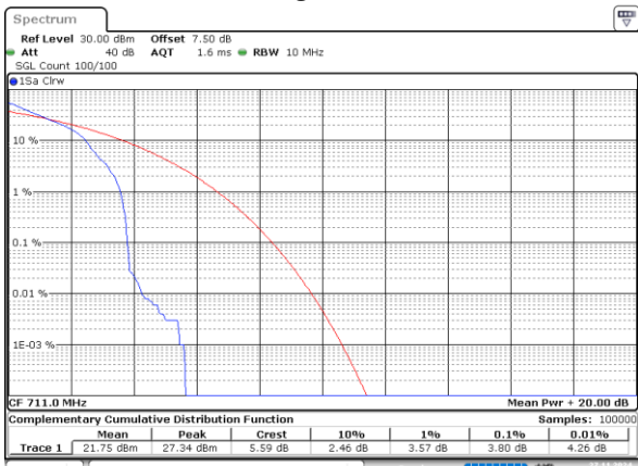
10MHz_High_QPSK_1@0
