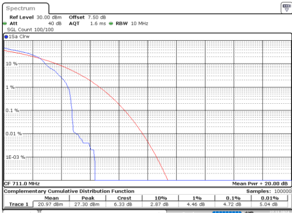
10MHz_High_16QAM_1@0
