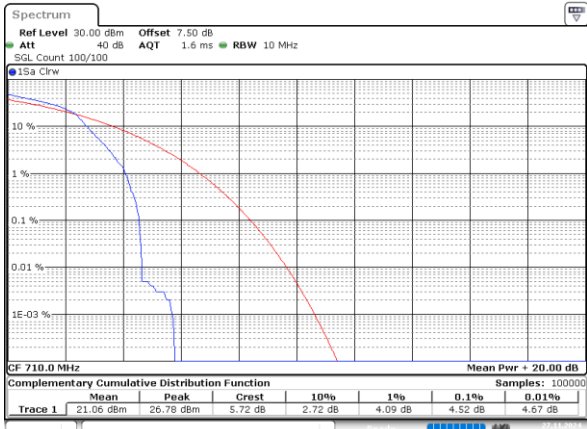
10MHz_Middle_16QAM_1@0
