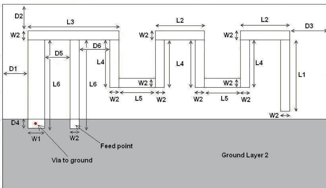
Figure 3: Antenna Dimensions
