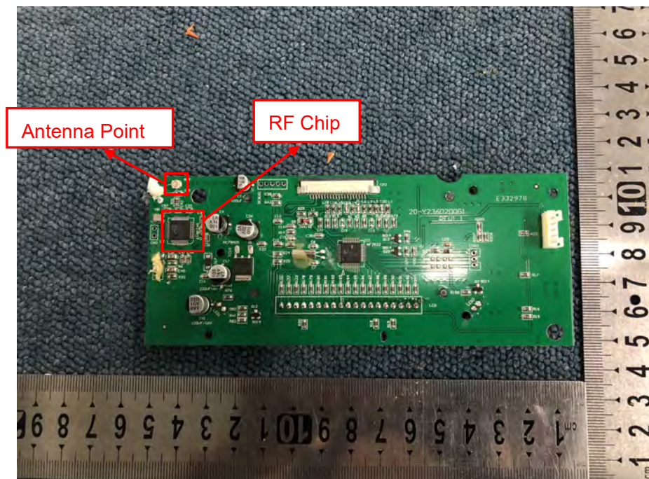
MAIN BOARD 3 BACK VIEW
