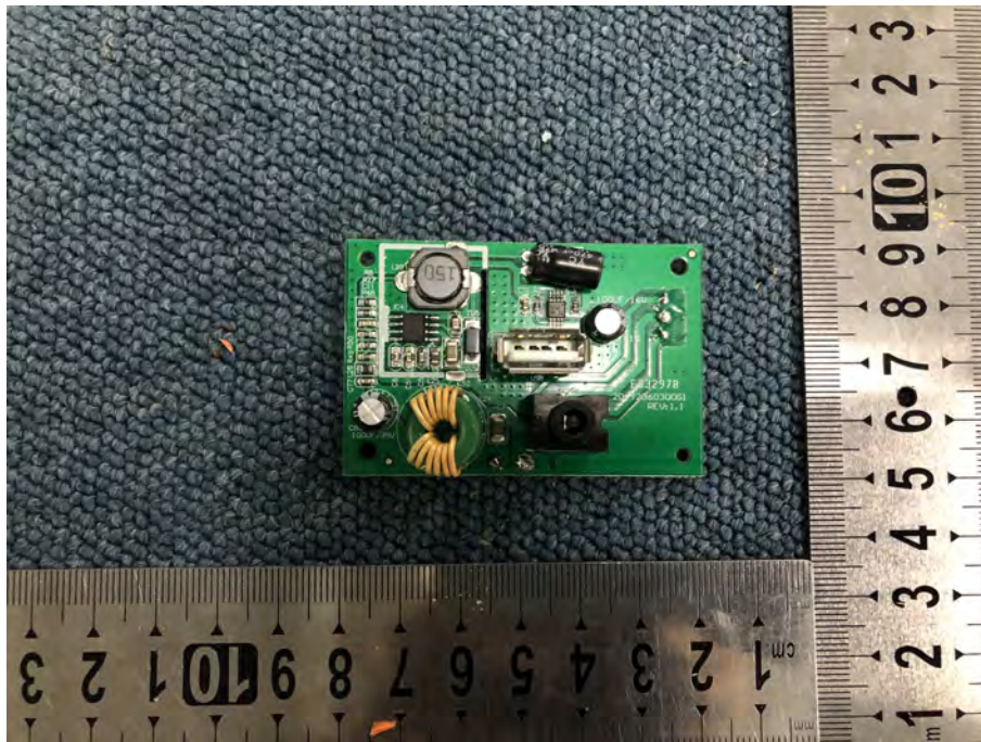
MAIN BOARD 2 FRONT VIEW(WITHOUT SHIELDING)
