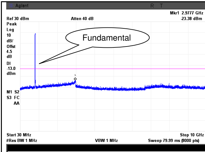
LTE Band 5 - Low Channel-1
