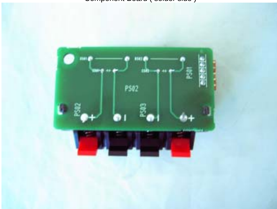
Component Board ( solder side )
