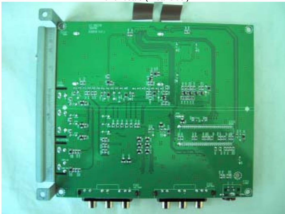
Tuner board ( Rear side )
