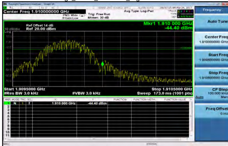
Band Edge_EDGE_1900MHz_HighCH810-1909.8
