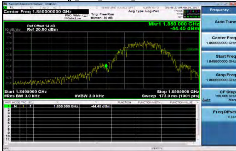
Band Edge_EDGE_1900MHz_LowCH512-1850.2
