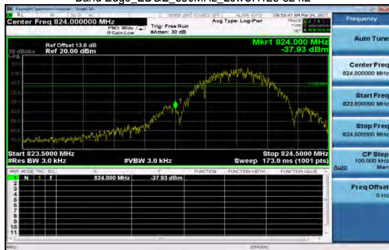
Band Edge_EDGE_850MHz_LowCH128-824.2
