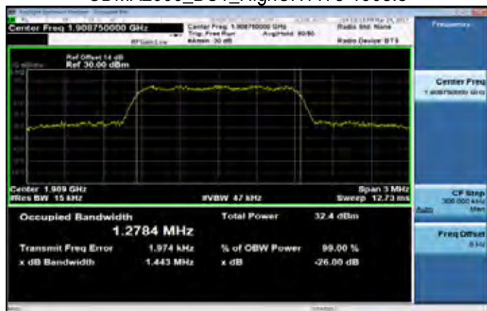
CDMA2000_BC1_HighCH1175-1908.8
