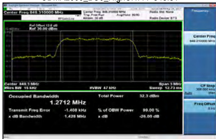
CDMA2000_BC0_HighCH777-848.31
