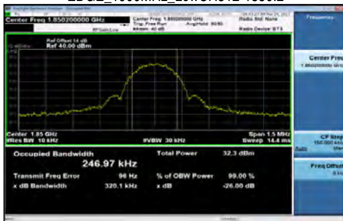
EDGE_1900MHz_LowCH512-1850.2
