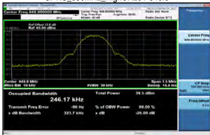
GPRS_850MHz_HighCH251-848.8
