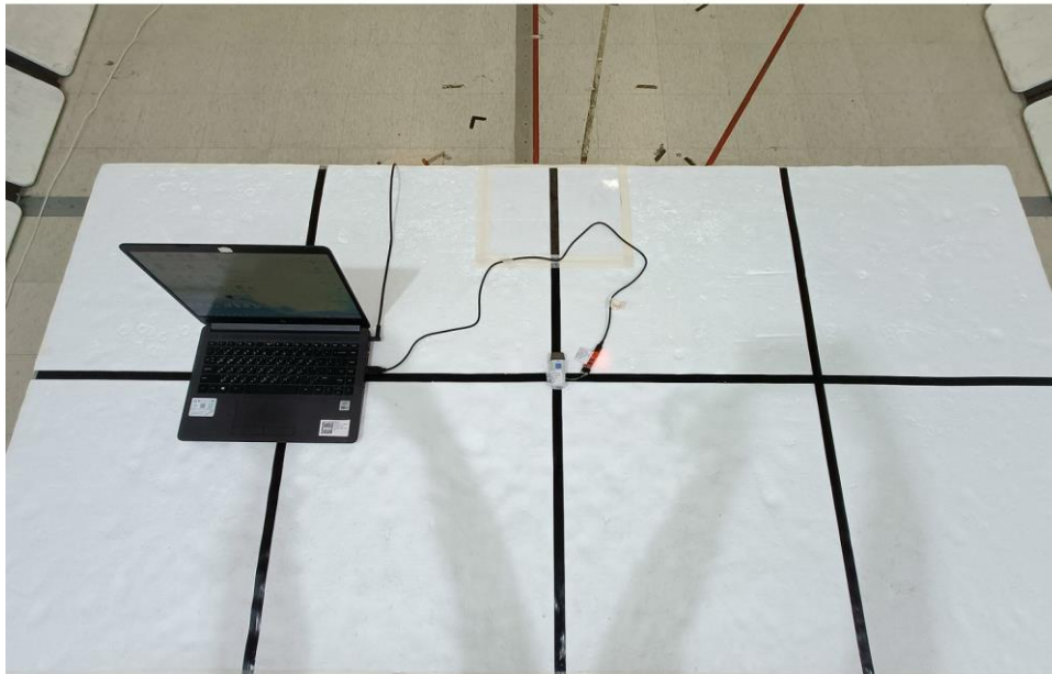
Below 1 GHz _ Rear View
