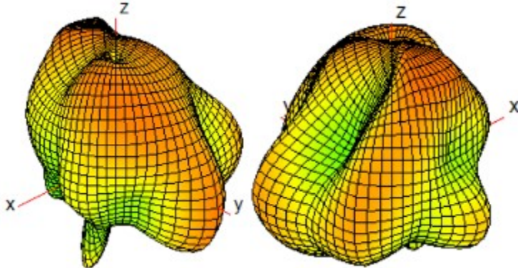
Ant 7(WiFi0/BT/GPS L1)_5800MHz
