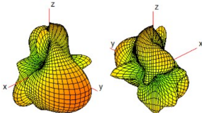
Ant 8(WiFi1/BT)_5200MHz
