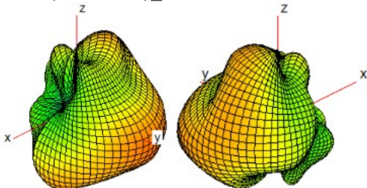
Ant 8(WiFi1/BT)_5200MHz
