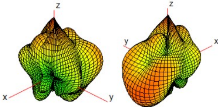
Ant 7(WiFi0/BT/GPS L1)_7000MHz
