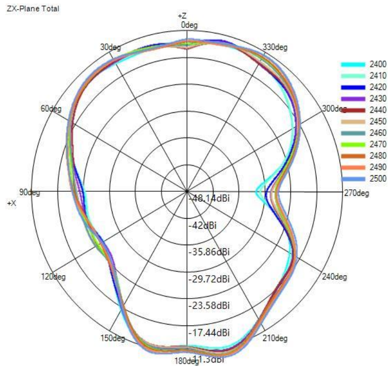
(1) X-Z Plane(unit:dBi):
