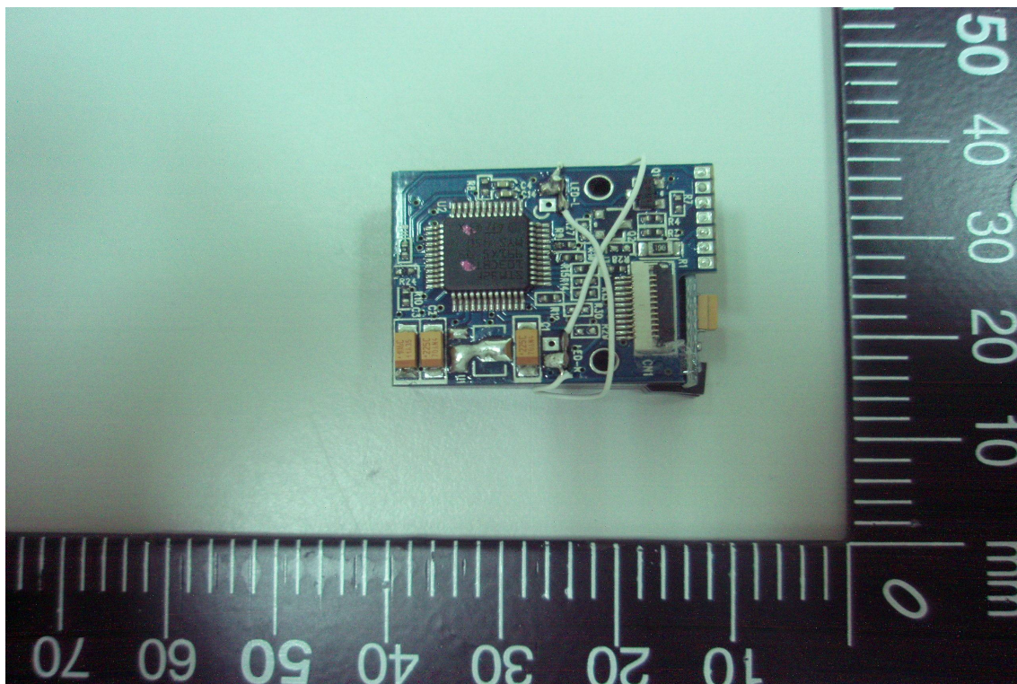
< PCB2-R >
