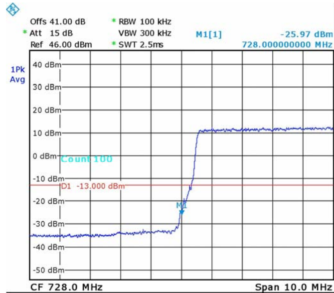
Figure 69.—64QAM, 733.0 MHz
