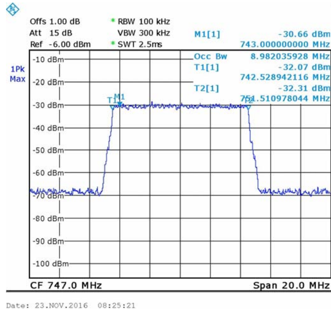
Figure 35. — QPSK 747 MHz IN
