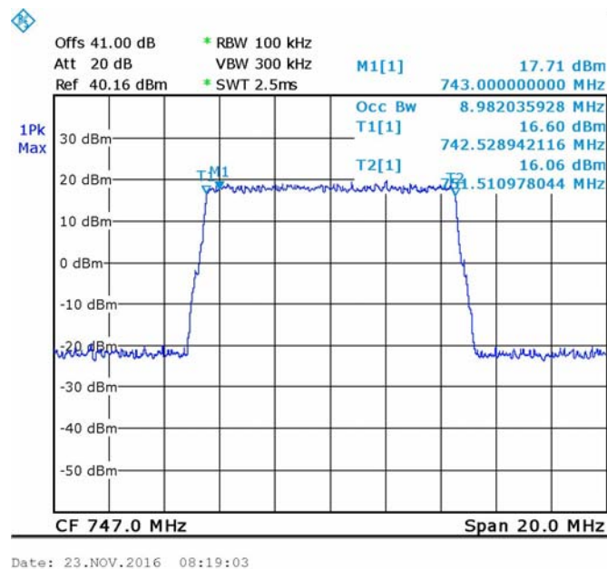
Figure 36. — QPSK 747 MHz OUT
