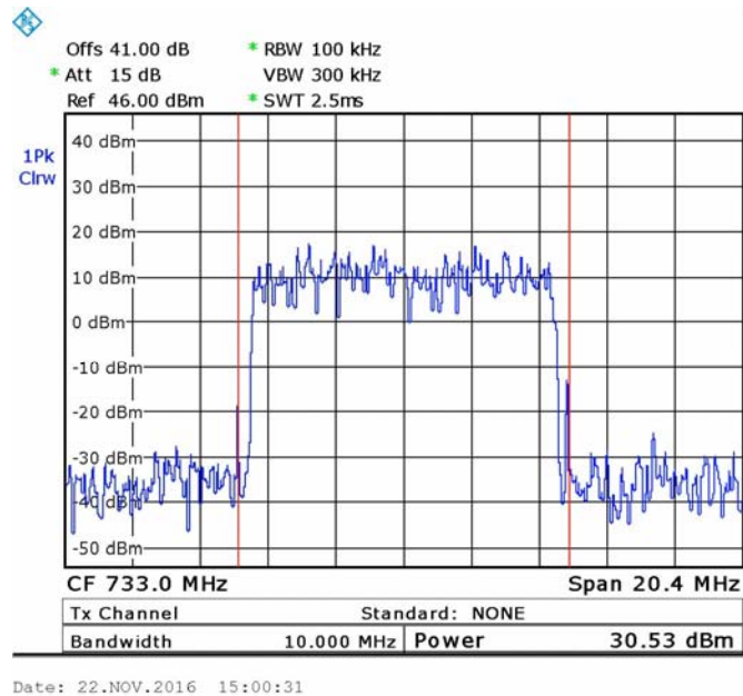
Figure 10. — 64QAM, 733 MHz
