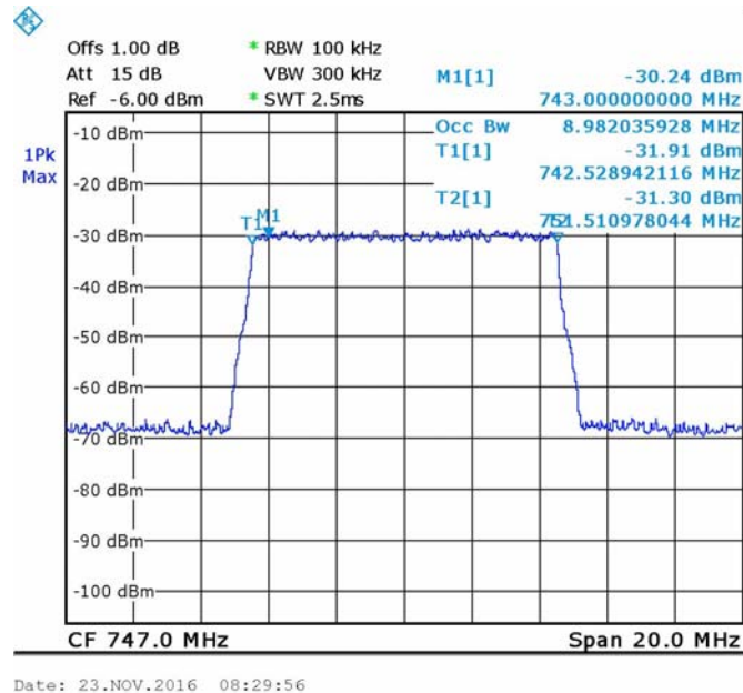
Figure 23. — 64QAM 747 MHz IN
