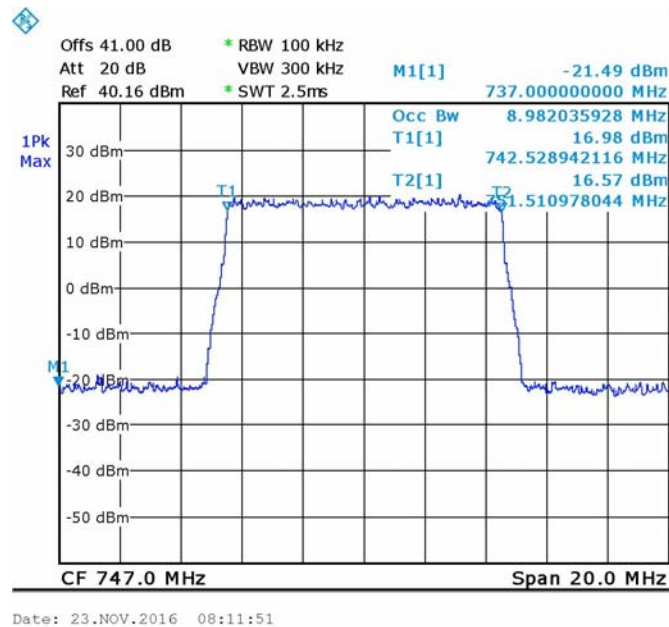
Figure 24. — 64QAM 747 MHz OUT
