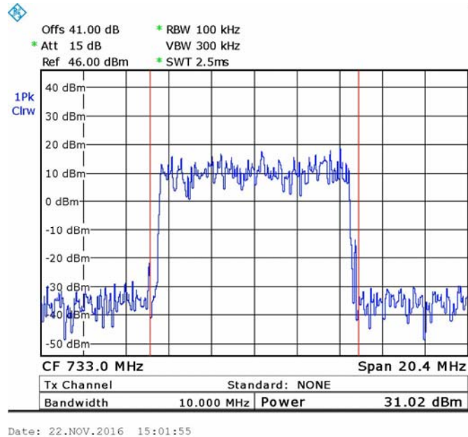
Figure 16. — QPSK 733 MHz
