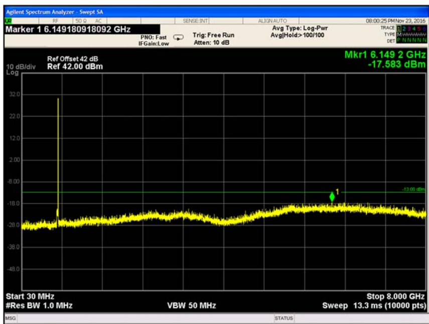
Figure 48 Spurious Emissions at Antenna Terminals 64QAM, 753MHz
