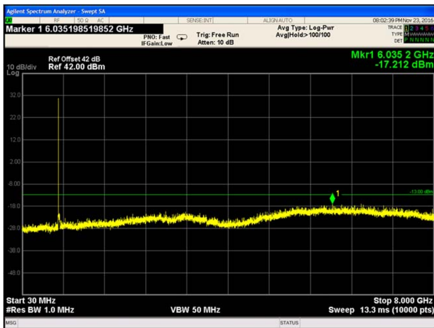
Figure 51 Spurious Emissions at Antenna Terminals QPSK, 733MHz
