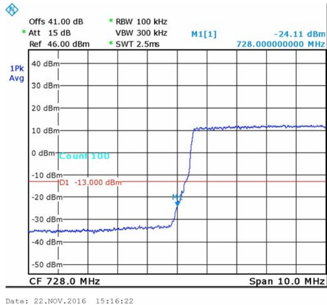
Figure 73. — QPSK, 733.0 MHz
