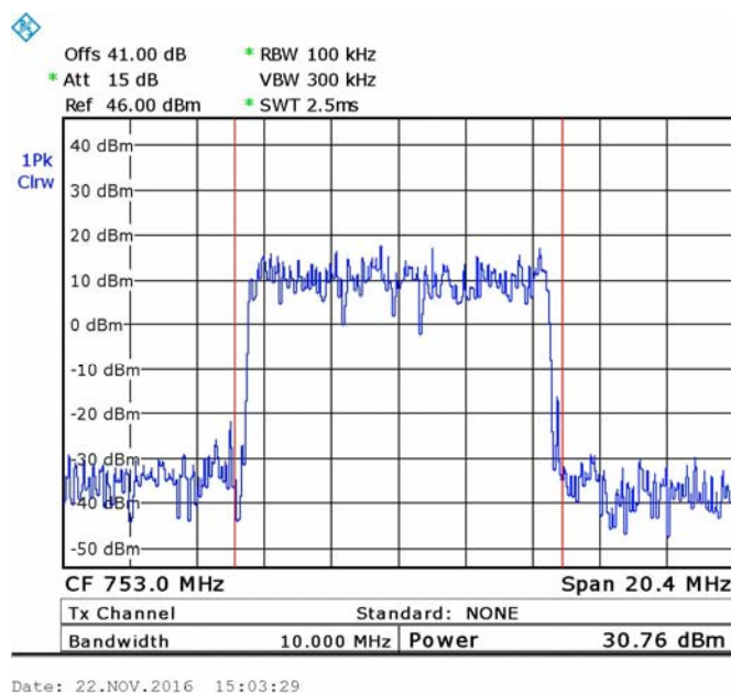
Figure 18. — QPSK 753 MHz
