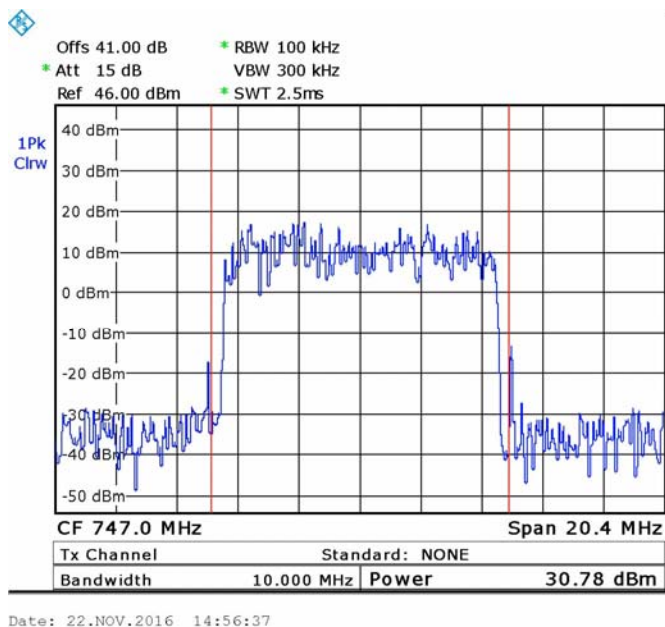
Figure 14. — 16QAM 747 MHz
