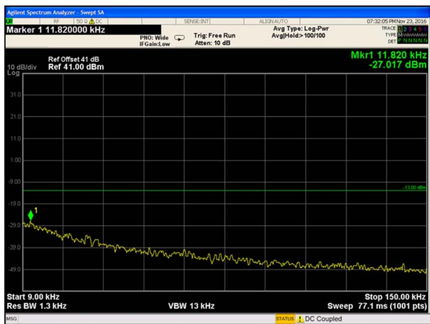
Figure 64 Spurious Emissions at Antenna Terminals 16QAM, 753MHz
