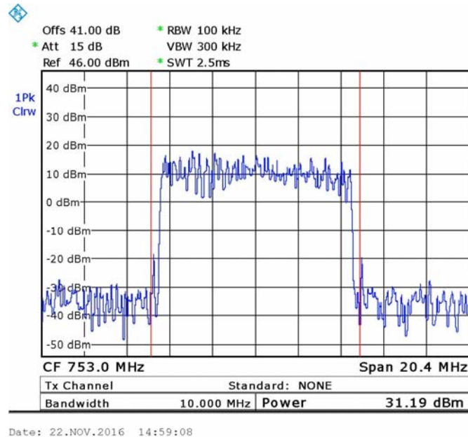
Figure 12. — 64QAM 753 MHz
